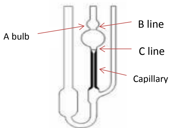
Figure 40. Ubbelohde Viscometer
