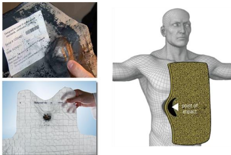
Figure 5. Back-face deformation. [6]
