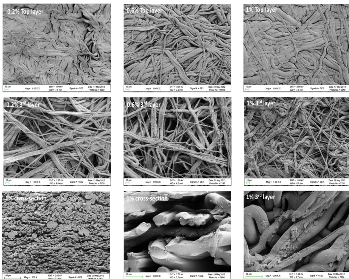
Figure 95. SEM imagers of hot pressed C60 sandwich composites: top layer, 3 rd layer, and cross-section.
