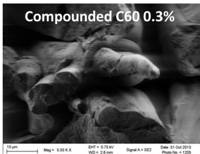
Figure 103. Cross-section of liquid nitrogen fractured samples.
