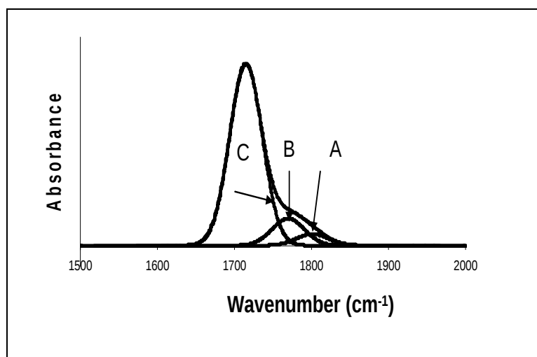
Dodecanoic acid
