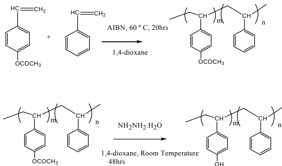
Figure 2.1 Schematic showing the synthesis of poly(styrene-co-4-vinyl phenol)
