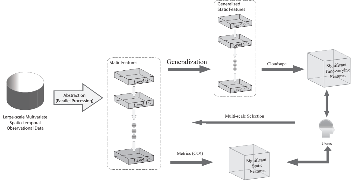
Figure 6.1: A general feature analysis pipeline
