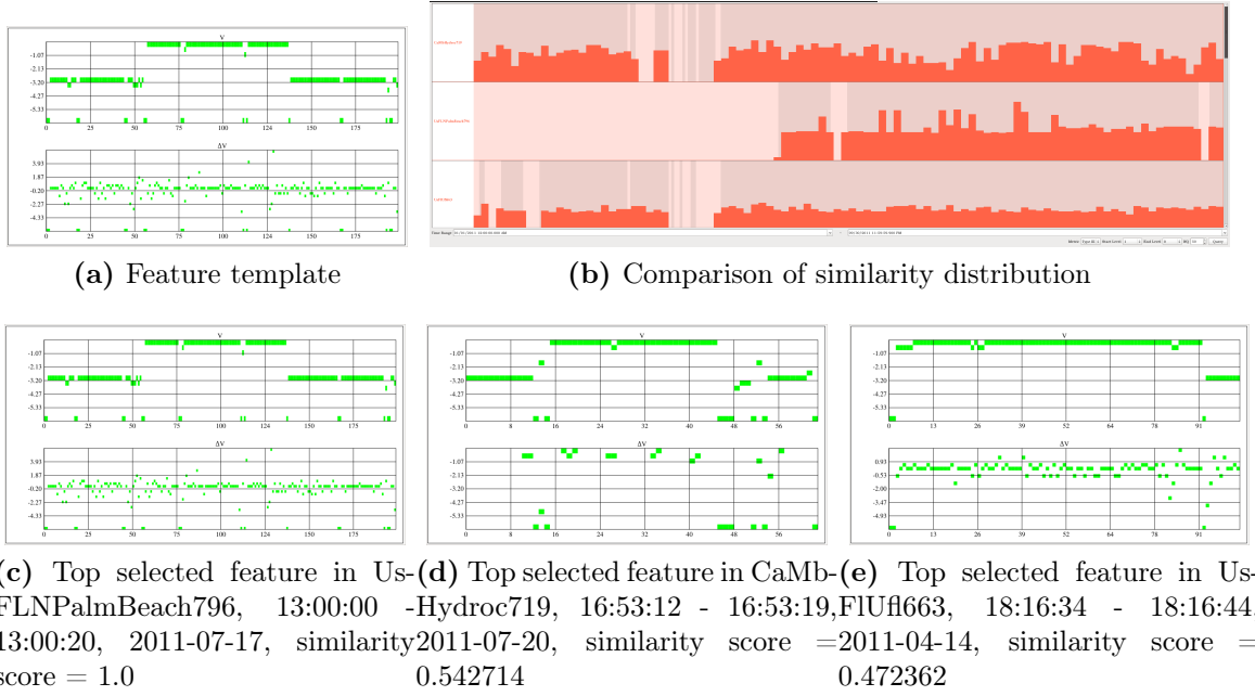
Figure 6.19: A time-varying feature template is created using a recorded transient step-shaped voltage variation pattern. The feature selection result using the created template of three locations including UsFLNPalmBeach796, CaMbHydroc719 and UsFLUf663 are compared on the similarity distribution.
