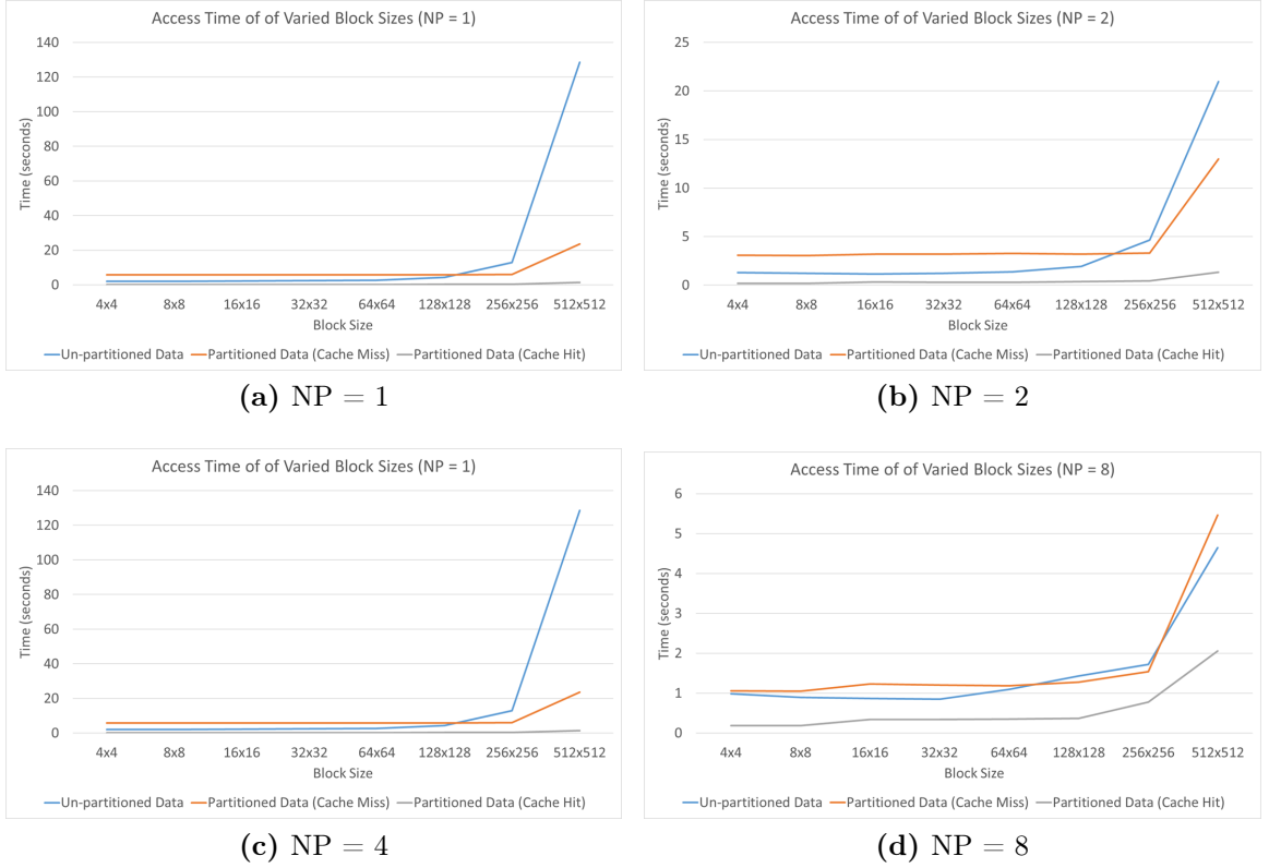
Figure 5.1: Data access time of varied block sizes when executed with 1 to 8 processes.
