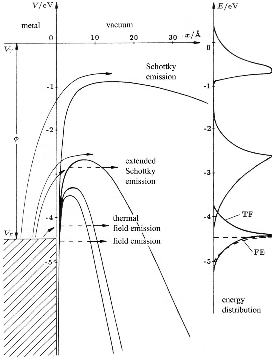
Figure 2.6: Energy distributions of different emission processes. The extended Schottky emission shows the biggest energy spread because two emission mechanisms overlap.
