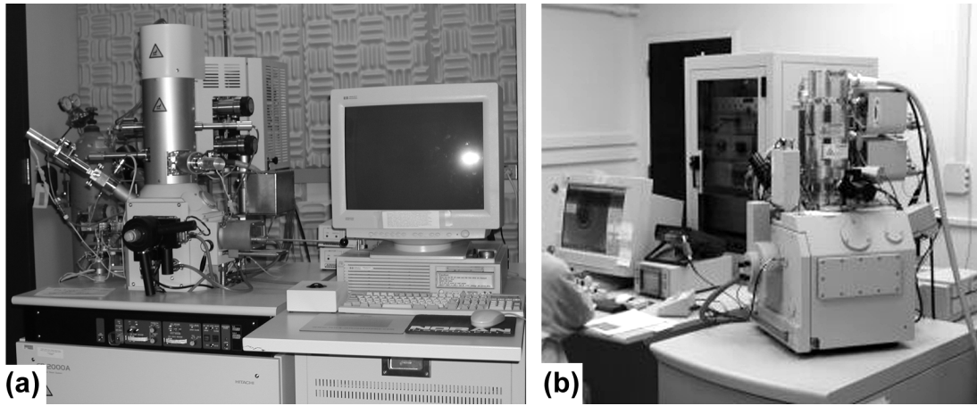
Figure 5.4: Single and dual beam FIB systems: (a) The Hitachi FB-2000 single beam FIB. (b) The FEI Strata 235 dual beam system.
