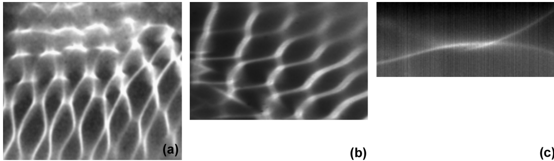
Figure 3.14: First reflection images obtained with the PPM. The images show a copper grid with increasing magnification from (a) to (c).
