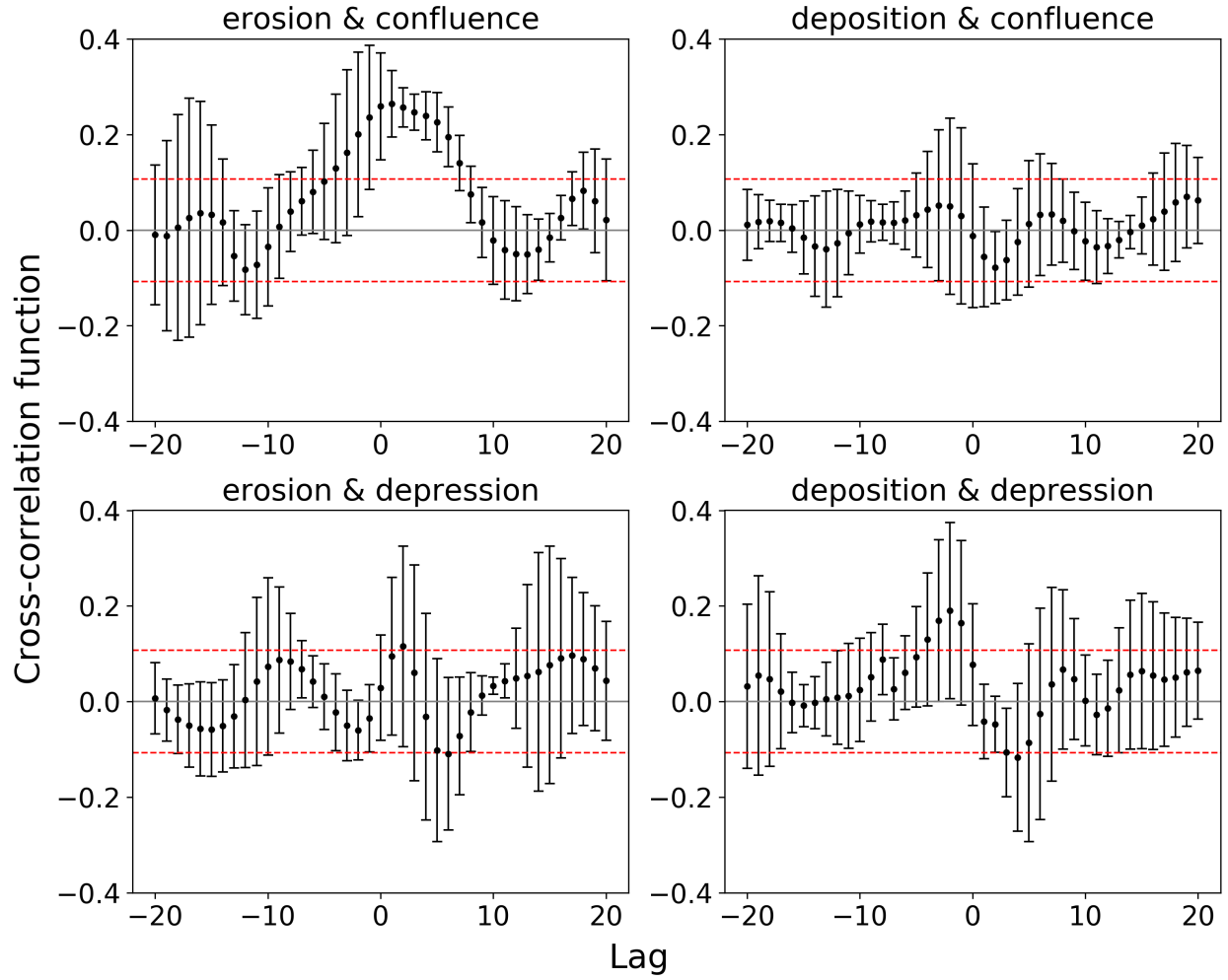
Figure 4.8: Results of the CCF between two sedimentological series (erosion and deposition) and two topographic series (confluence and depressions). Red dashed lines represent the 0.95 confidence interval. The spatial distance between any two adjacent locations of the same series is 0.05 m.
