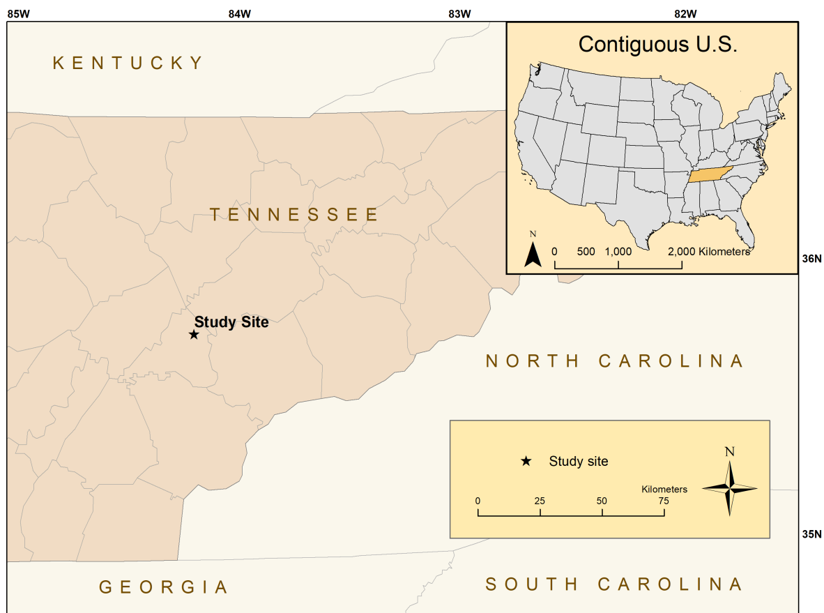
Figure 3.1: Study area of this research
