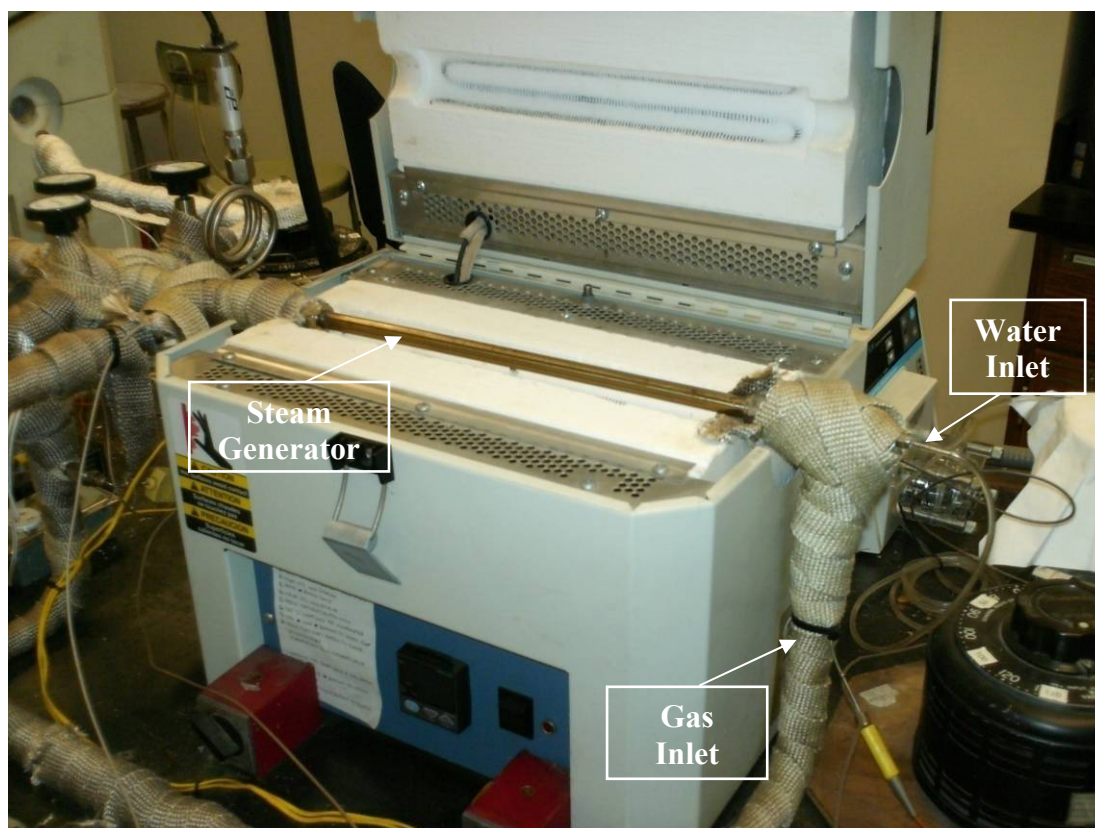
Figure 3.3.2 – Steam generator assembly
