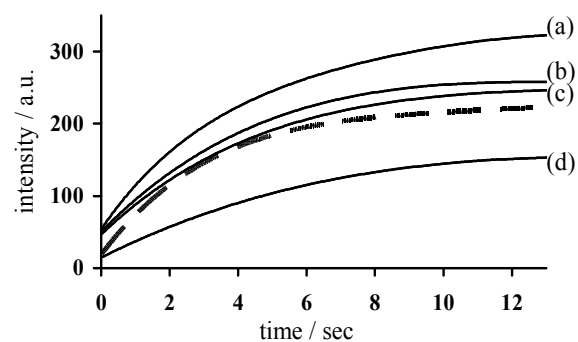
Figure 5.2 Kinetic test showing increase of the 1E-4 M rhodamine 6G SERS signal (peak 1495 cm -1 ) over time while mixed with AgNP pluronic complex concentrations of (a) 3 µg/mL, (b) 50 µg/mL, (c) 100 µg/mL, and (d) 500 µg/mL. Dashed line indicates the signal of non modified AgNP's.
