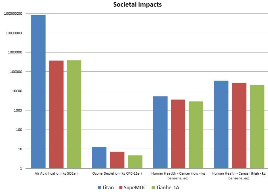
Figure 6: Societal Impacts of 3 Supercomputers for the Cooling Manufacturing and Use Phase and Compute Use Phase: Log Plot
