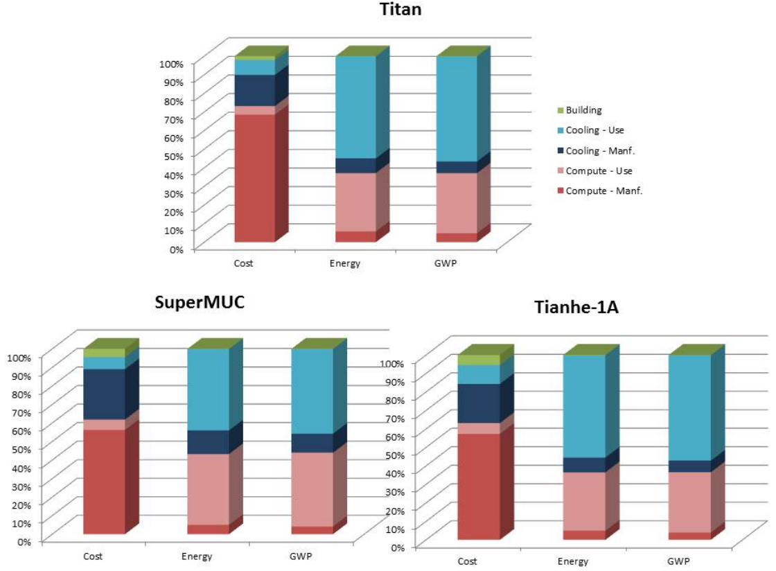
Figure 5: The Percentage of Cost, Energy, and Global Warming Potential by Infrastructure and Phase for 3 Supercomputers
