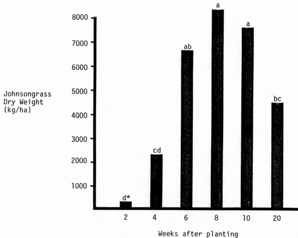
Figure 14. Seasonal growth of johnsongrass growing in competition with corn, Knoxville.
