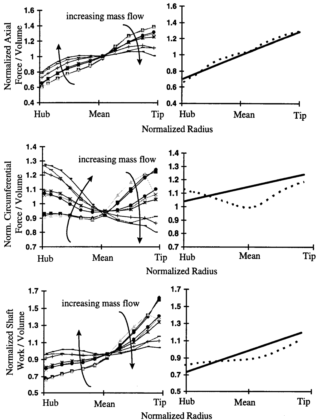
Figure 33. Source Term Correlation Based on Collapse in Mass Flow Found from Streamline Curvature Code Solutions
