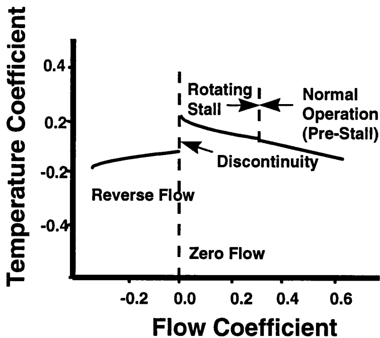
b. Temperature Coefficient, \Psi^T , Versus Flow Coefficient, \Phi
