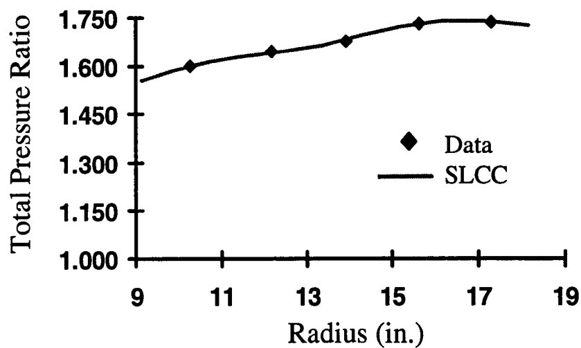
a. Total Pressure Ratio as a Function of Radius
