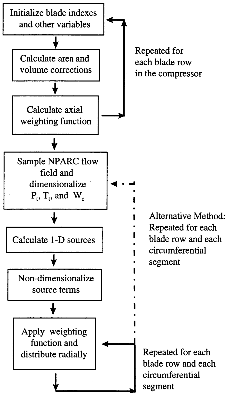
Figure 14. Block Diagram of 3-D Source Calculations.
