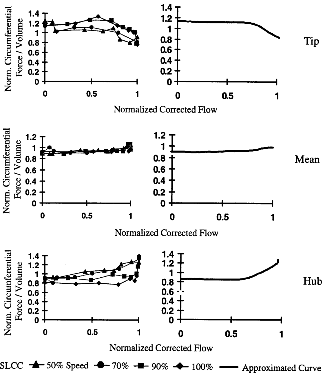
c. Normalized Circumferential Force on Per Volume Basis
