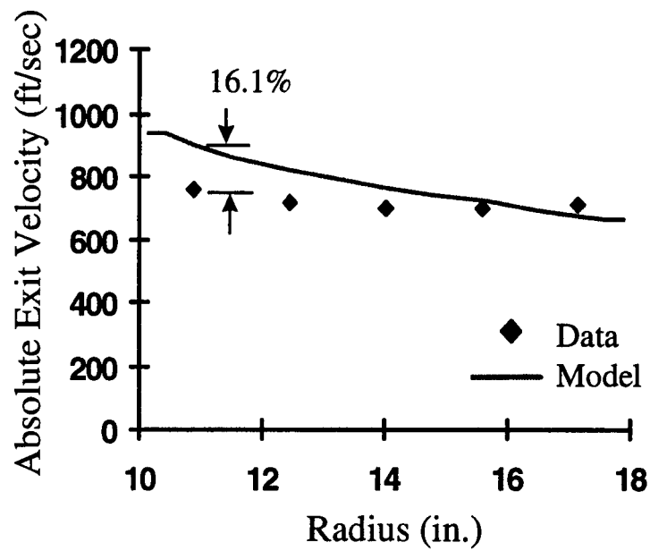
a. Absolute Exit Velocity as a Function of Radius
