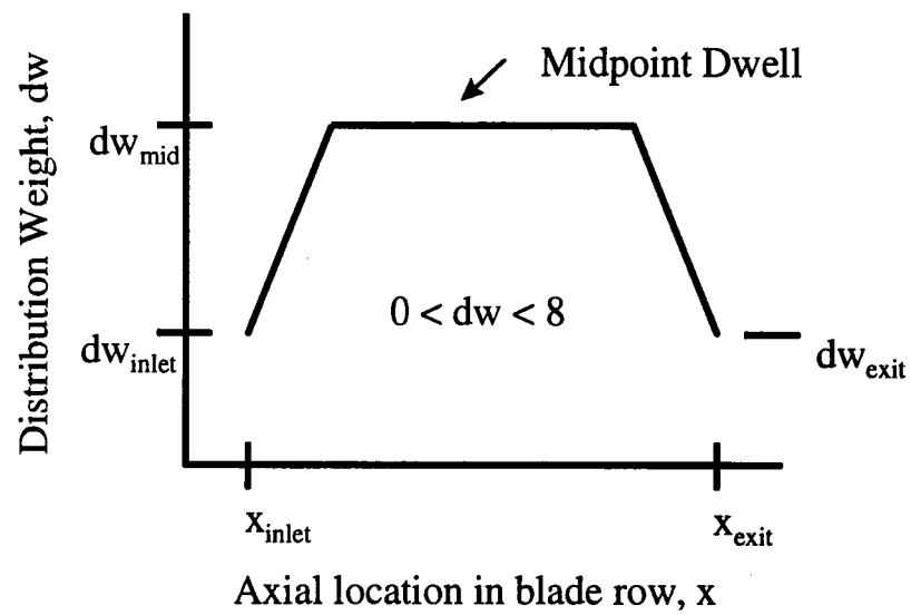
a. Typical Axial Distribution Shape
