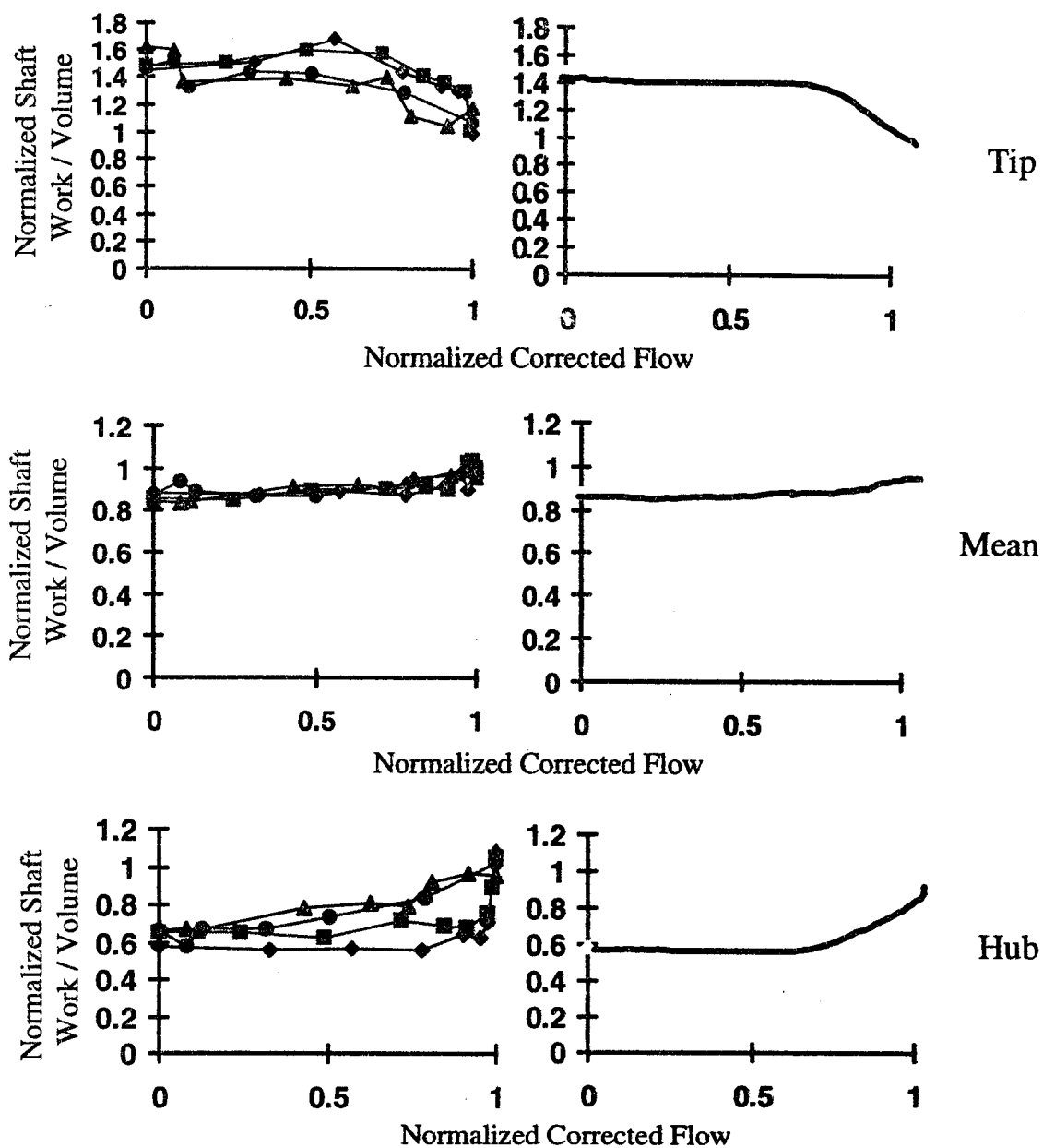
a. Normalized Shaft Work and Approximated Curves on Per Volume Basis
