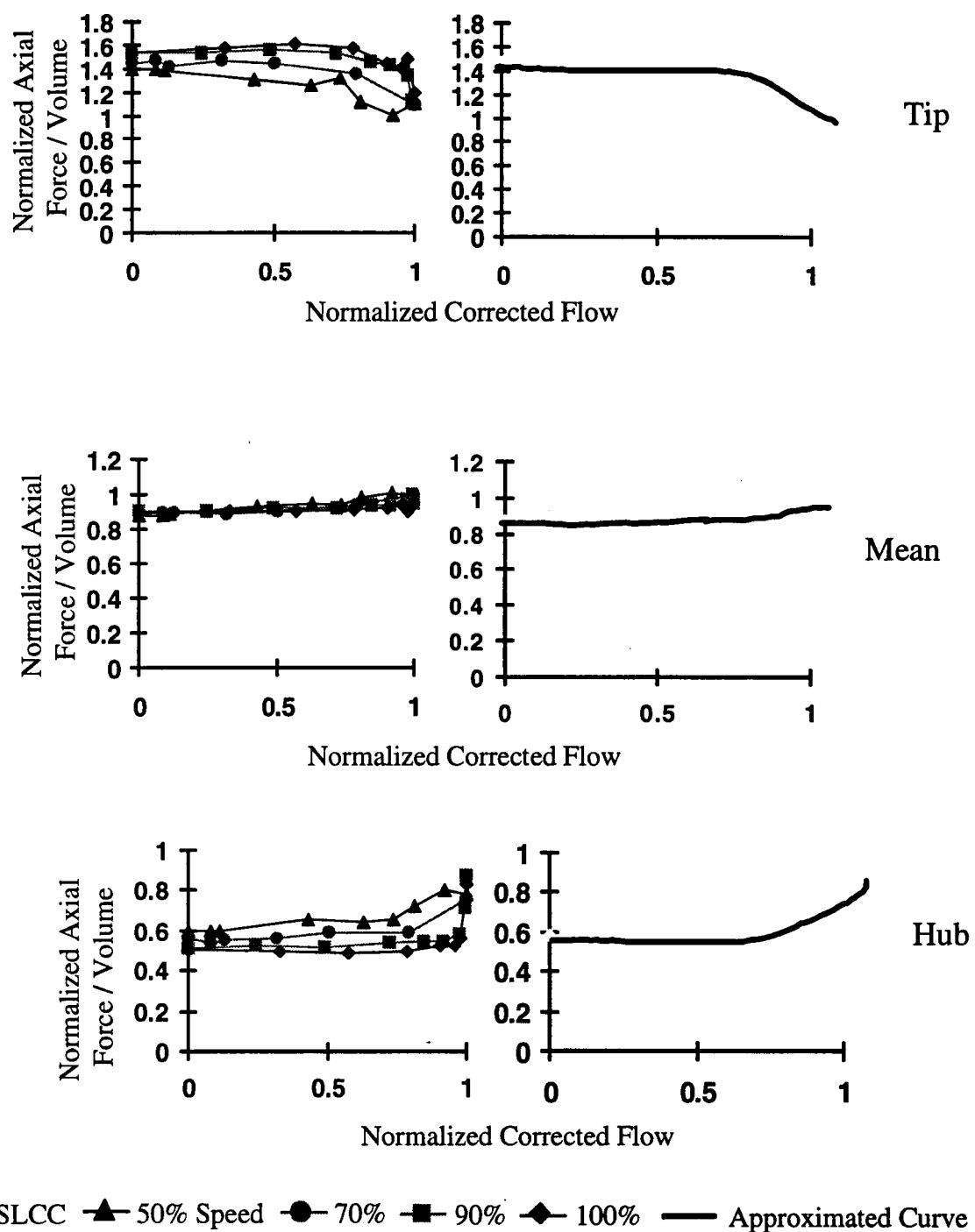
b. Normalized Axial Force on Per Volume Basis
