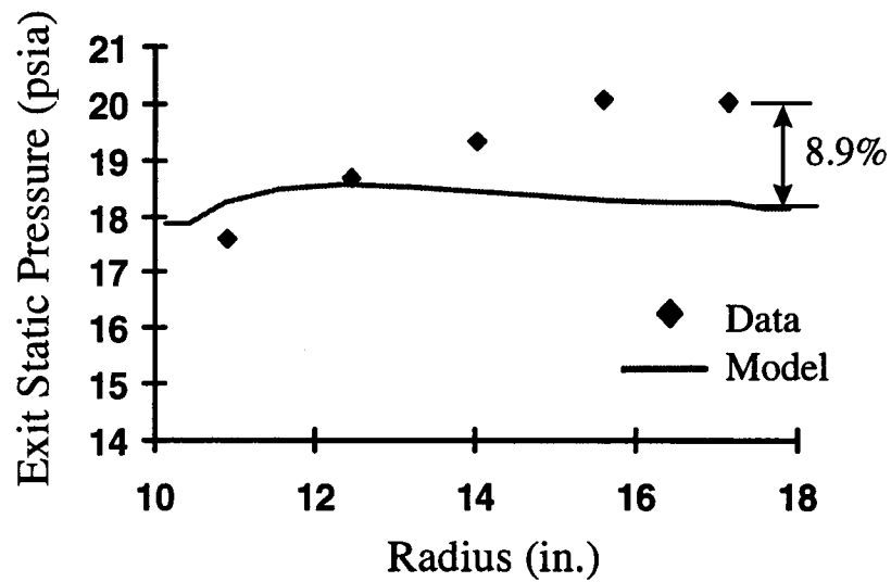
b. Exit Static Pressure as a Function of Radius
