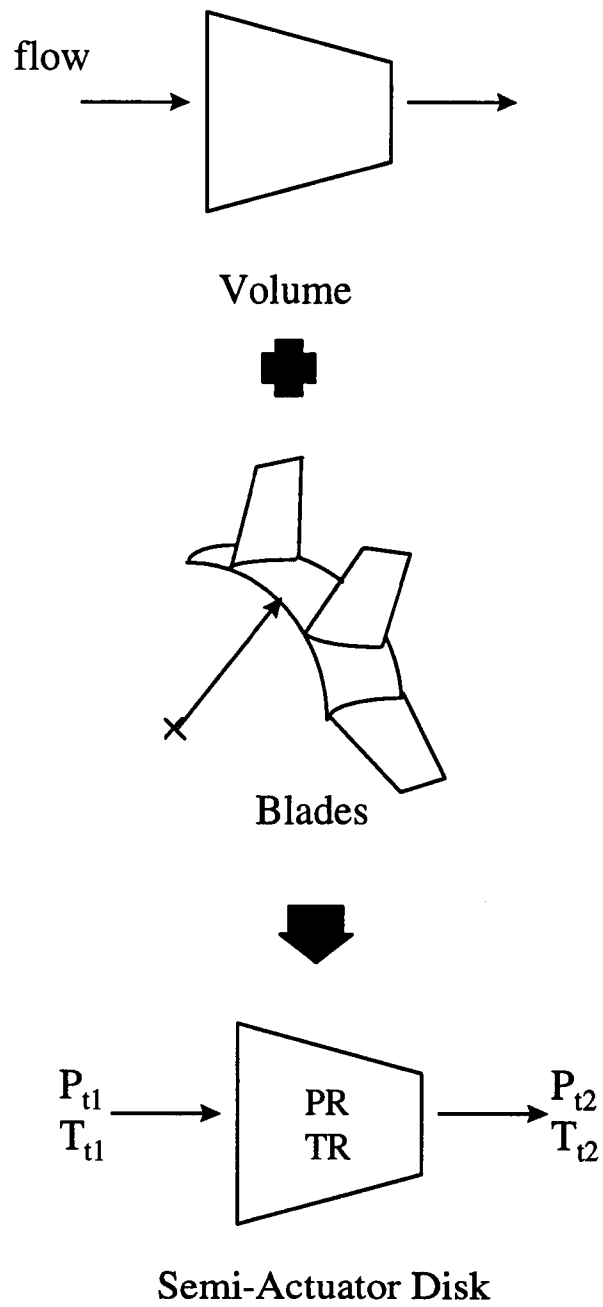
Figure 4. Semi-Actuator Disk Methodology.
