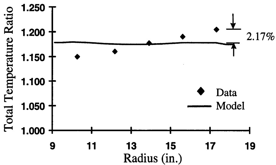
b. Total Temperature Ratio as a Function of Radius
