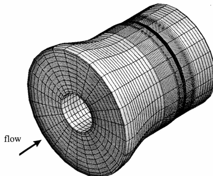
Figure 9. Three-Dimensional Computational Grid, 69x13x26, for Rotor 1B.
