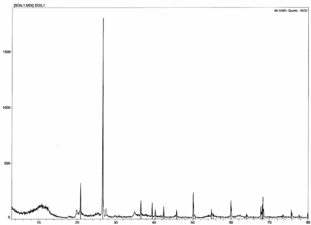
X-ray Diffraction Results: Clay
