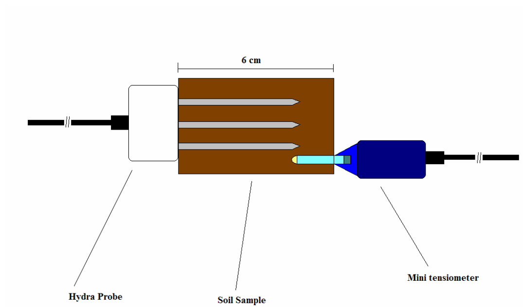
Setup of equipment within soil samples
