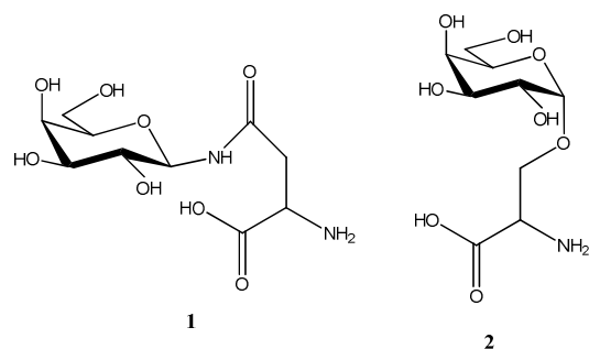
Figure 1. N-linked galactose and O-linked galactose
