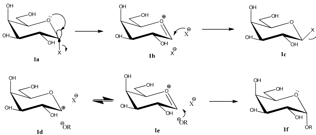
Figure 5. Halide mechanism
