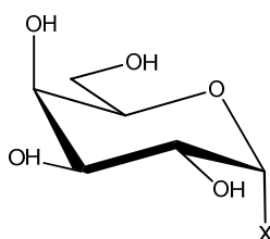
Figure 4. \alpha -Galactopyranosyl halide
