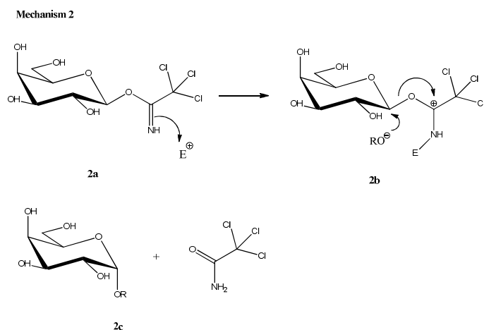
Figure 6. Mechanism of inverting the stereocenter
