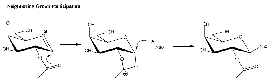
Figure 7. Neighboring group participation
