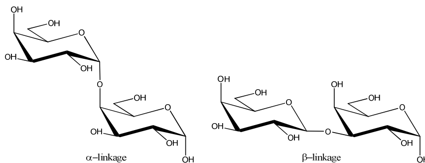
Figure 3. \alpha -Linked and \beta -linked galactose disaccharides
