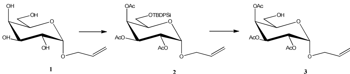
Scheme 1. Synthesis of allyl – O - 2,3,4- tri – O - acetyl- \alpha -D-galactopyranoside
