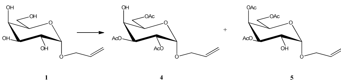
Scheme 2: Synthesis of allyl – O - 2,3,6-tri - O - acetyl- \alpha -D-galactopyranoside and allyl – O - 3,4,6 – tri – O- acetyl- \alpha -D-galactopyranoside
