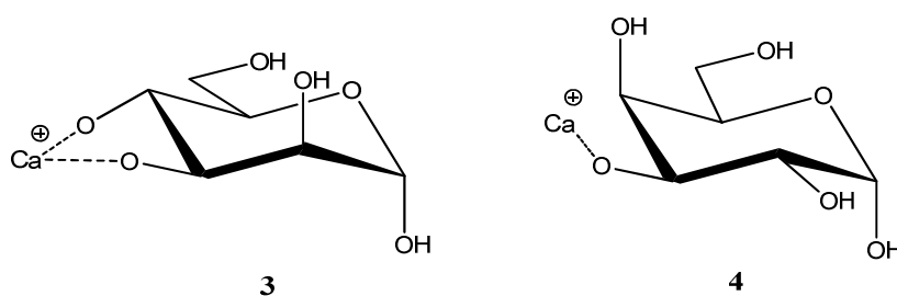
Figure 2. Calcium coordinated between two equatorial hydroxy groups (3) and calcium coordinated with galactose (4)
