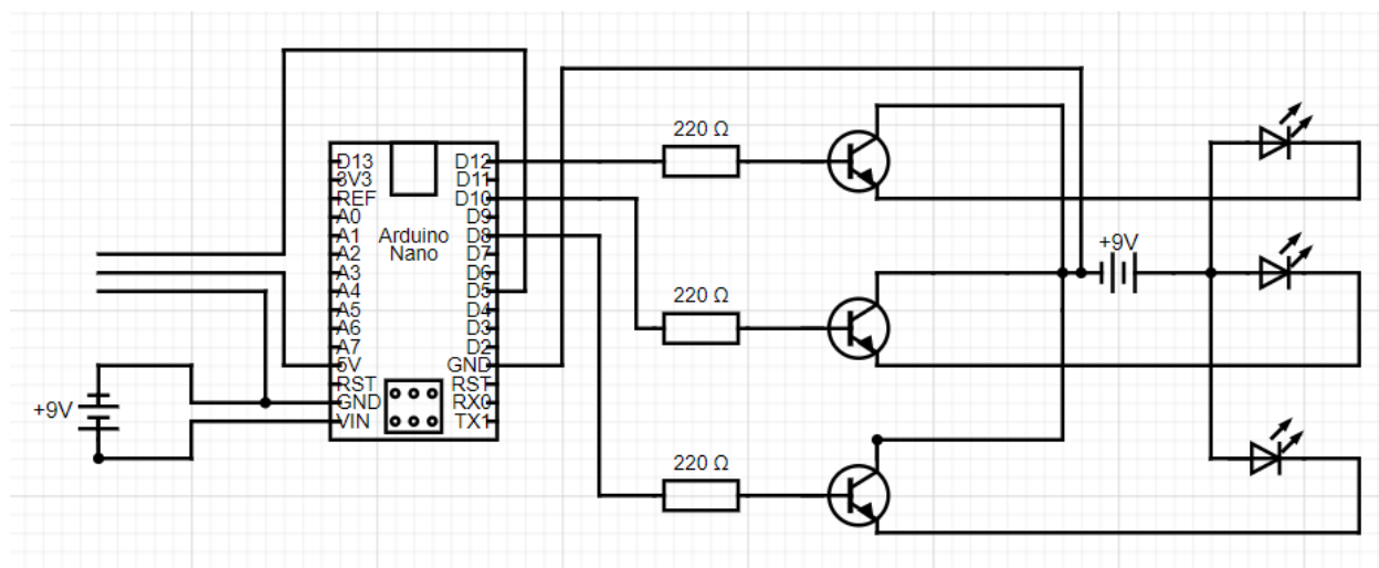
Figure 4.3: Circuit Diagram
