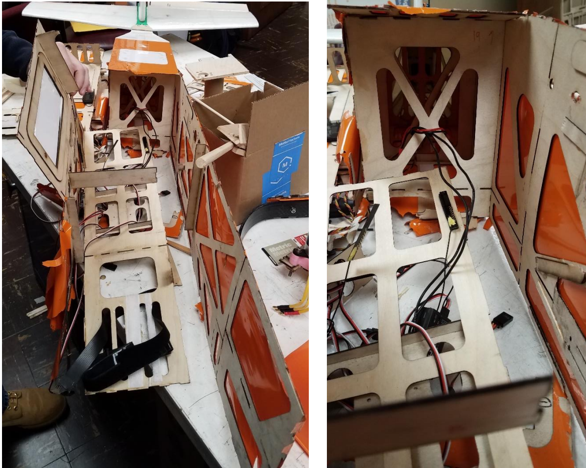
Figure 5.1: Images of the wreckage of Prototype 1, showing close-ups of the points of failure.
