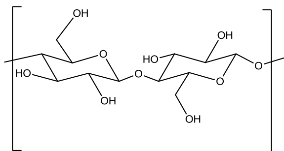
Figure 1.7: Chemical structure of cellulose chain.
