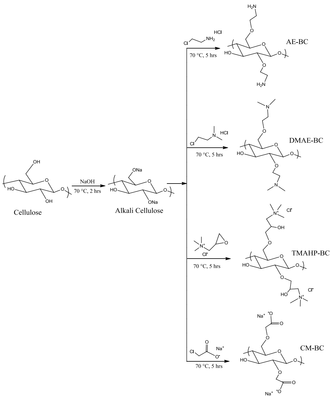
Figure 5.1: Surface functionalization reactions performed on bacterial cellulose.
