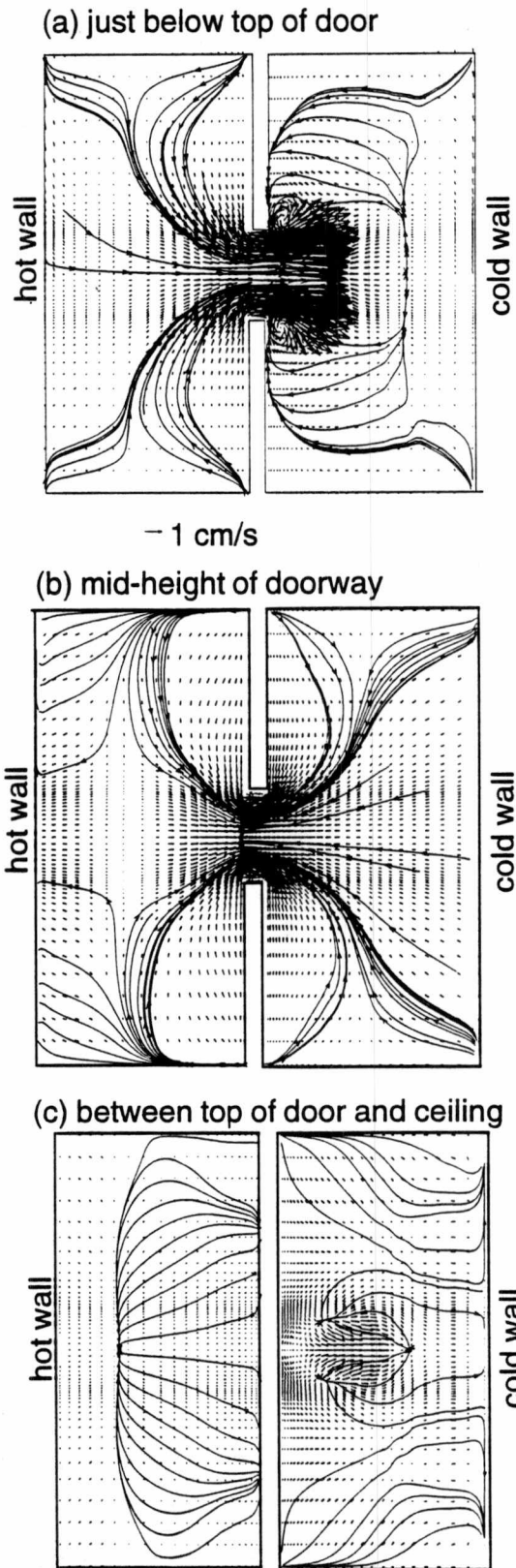
Figure 117. Streamlines projected onto horizontal planes - Ra=3.2 \times 10^{10} .
