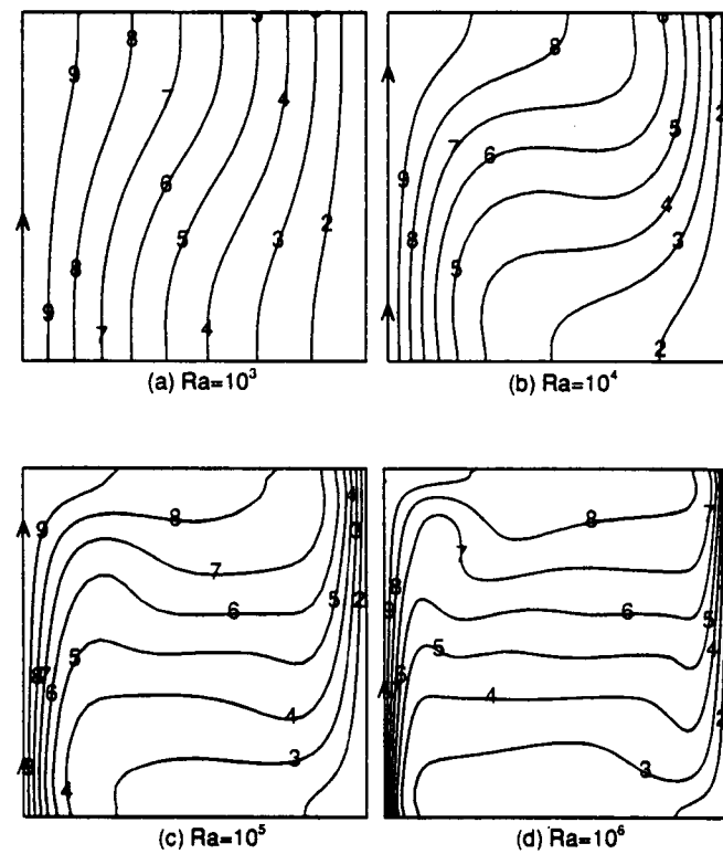
Figure 26. Temperature contours at 0(0.1)1 , present data.
