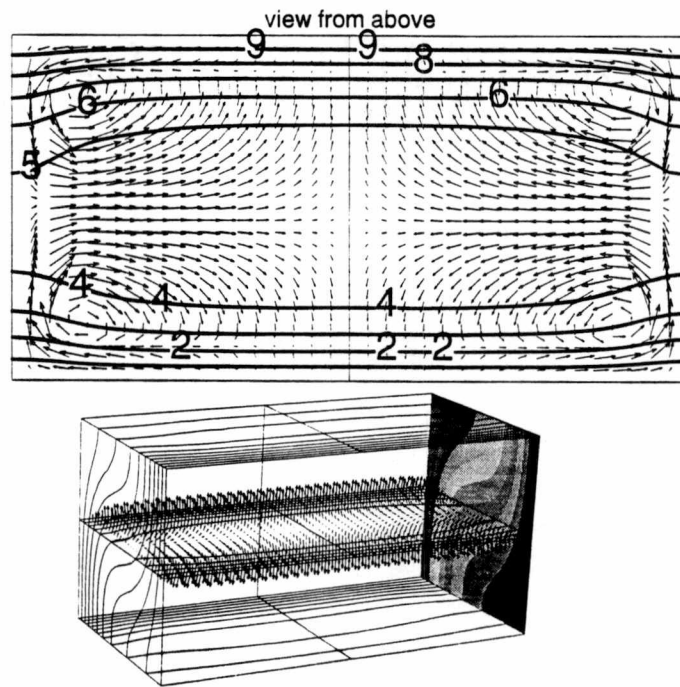
Figure 36. View of horizontal mid-plane Ra=10^4 Pr=0.1 : temperature \theta(0.1)1 .
