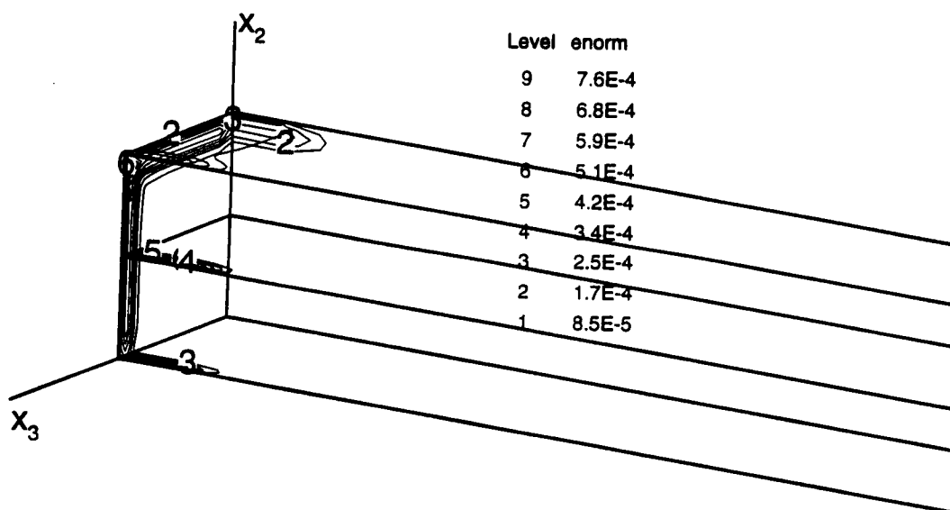
Figure 18. Developing flow in a square channel: \|\Phi\|_E distribution near entrance, Re=100 .
