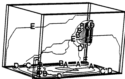
Figure 88. Isotherms for 15 ACH.
