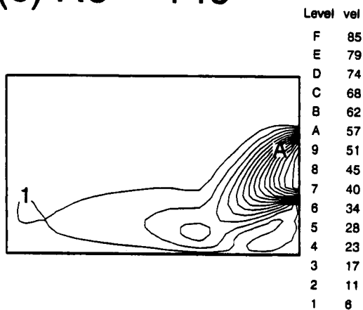
Figure 101. Air speed contours for 15 ACH, Ar=4.3 .
