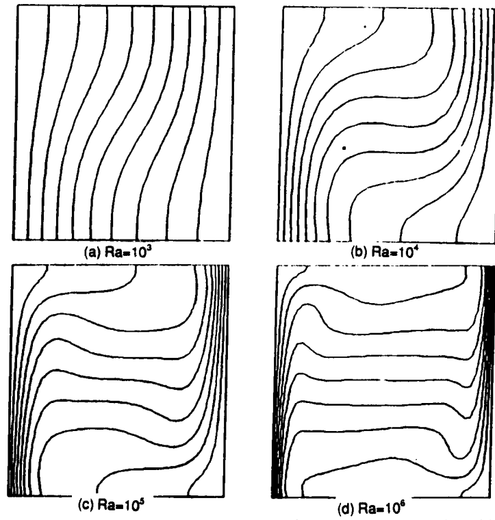
Figure 25. Temperature contours all at 0(0.1)1 , de Vahl Davis (1983).
