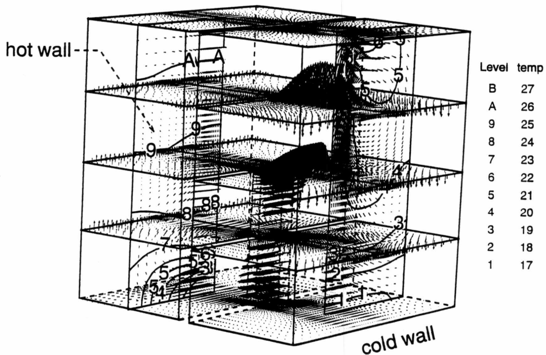
(b) temperature distributions on spanwise cutting planes
