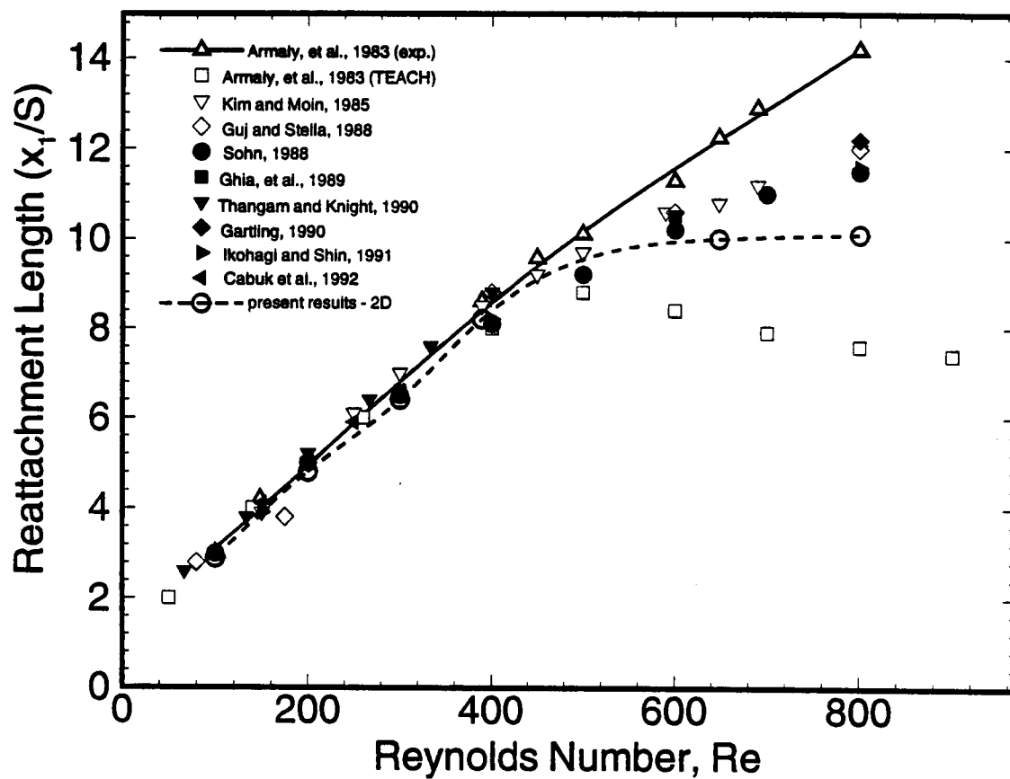
Figure 59. Primary reattachment length v. Re , 2-dimensional solutions.
