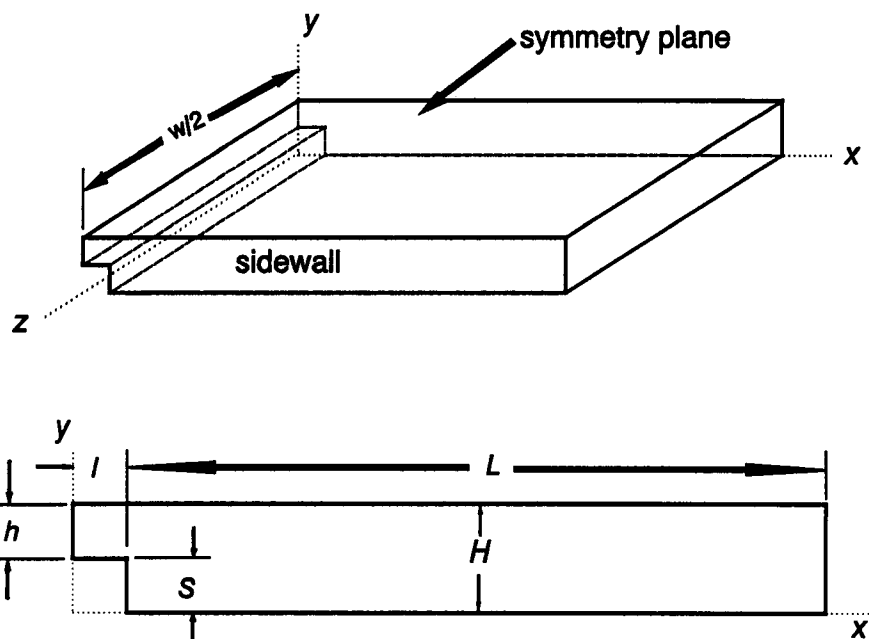
Figure 51. Step-wall diffuser geometry.
