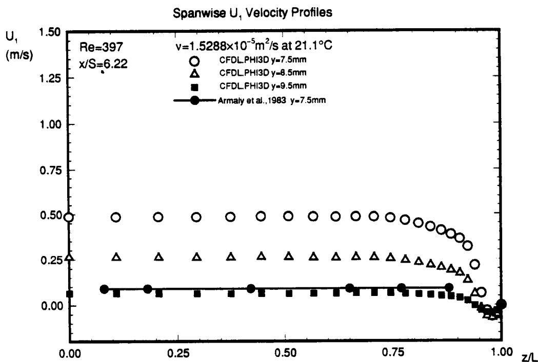
Figure 64. Comparison of spanwise velocity distributions, Re=397.
