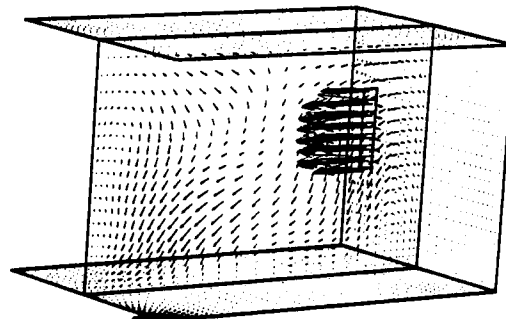
Figure 94. Longitudinal plane for 30 ACH.
