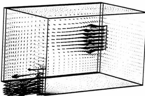
Figure 93. Velocity solutions for 30 ACH.
