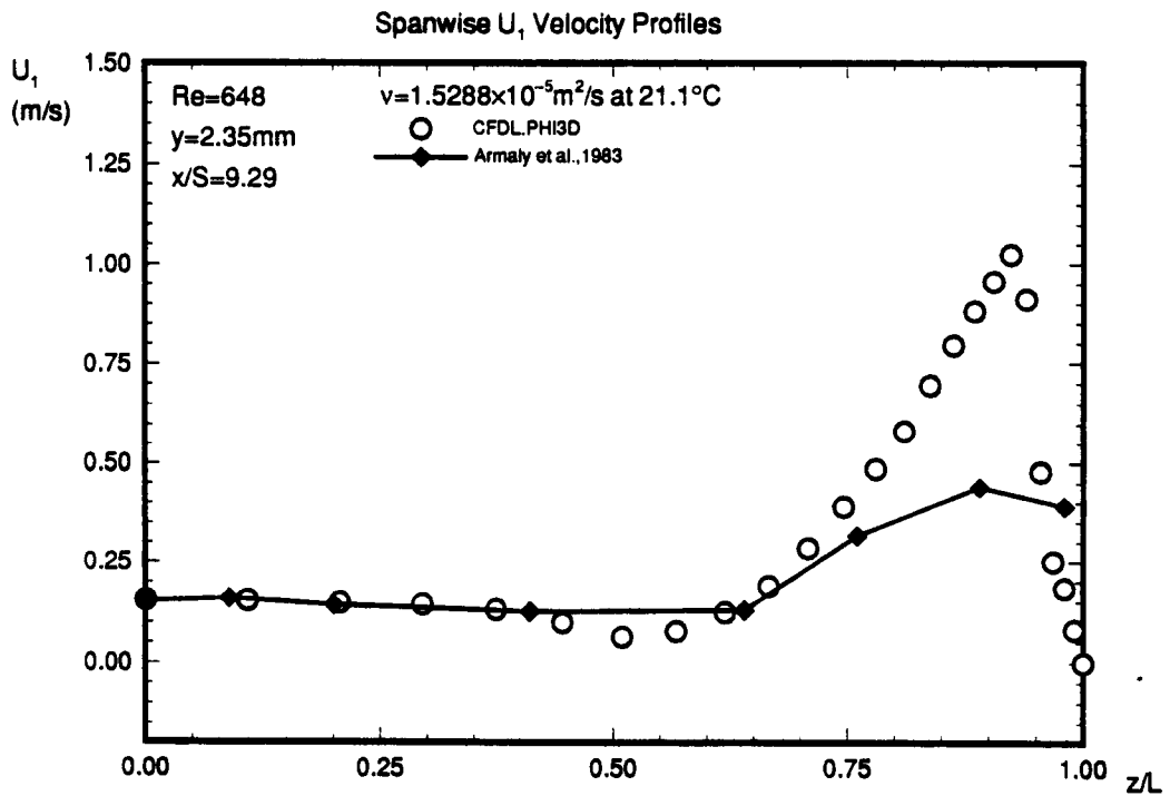
Figure 67. Comparison of CFD and experimental spanwise axial velocity profiles, y=2.35 \text{ mm} Re=648 .
