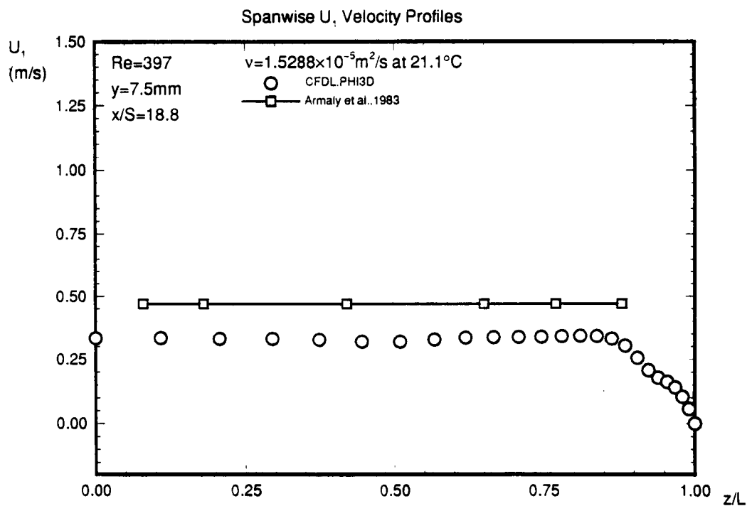
Fig. 64. (continued) Comparison of spanwise axial velocity distributions, Re=397 .
