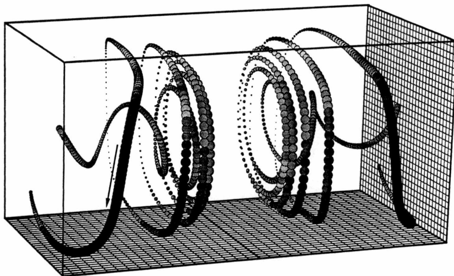
Figure 34. Particle tracks for Ra=10^4 Pr=0.1 .
