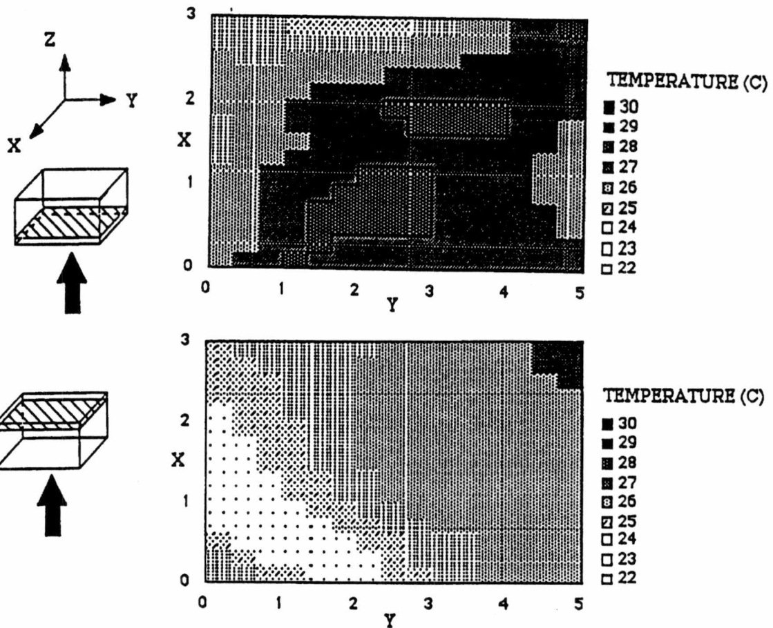
Figure 83. Measured room temperature distributions in horizontal planes, 50 ACH, Cantillo(1990).
