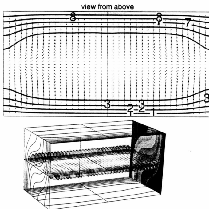
Figure 37. View of horizontal mid-plane Ra=10^4 Pr=100 : temperature \theta(0.1)1 .
