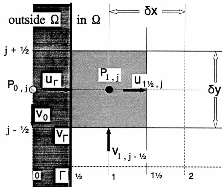
Figure 2. Layout of staggered mesh at boundary.
