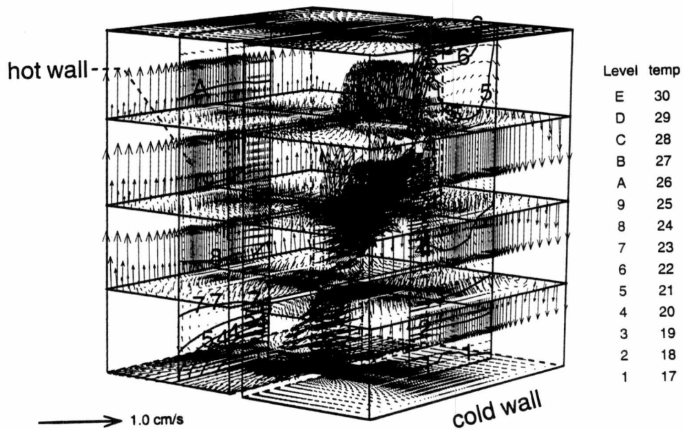
(a) temperature distribution on lateral cutting planes
