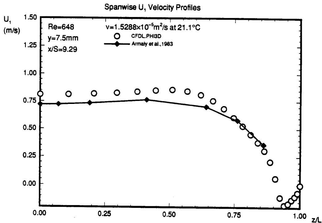
Figure 66. Comparison of CFD and experimental spanwise velocity profiles, y=7.5 \text{ mm} Re=648 .
