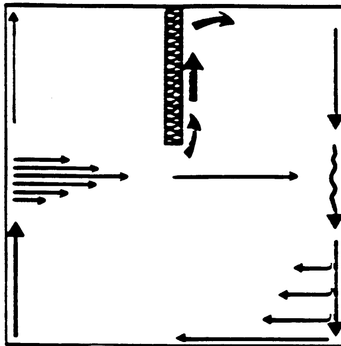
Figure 108. Flow visualization in the water cell, w/W=0.2 (Neymark, 1988).
