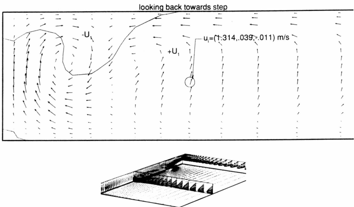
Figure 74. Flow field near the sidewall projected onto transverse planes, Re=800 .
