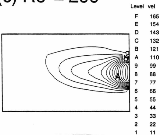
Figure 102. Air speed contours for 30 ACH, Ar=0.82 .
