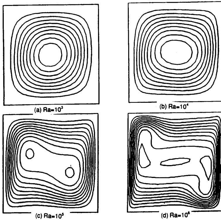
Figure 23. Contour maps of streamfunction, de Vahl Davis (1983).
