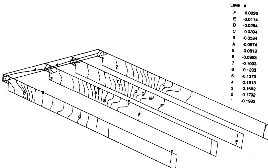
Figure 72. Pressure contours for Re=648 .
