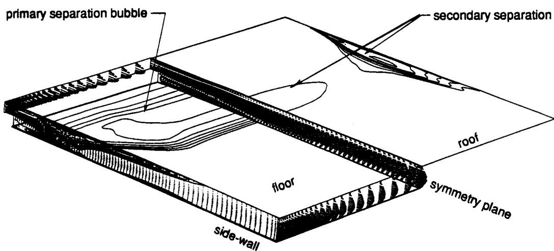
Figure 71. Separation region "footprints", Re=800 .
