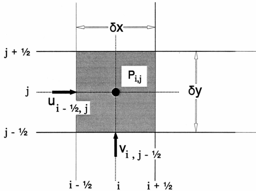
Figure 1. Layout of staggered mesh at interior cells.
