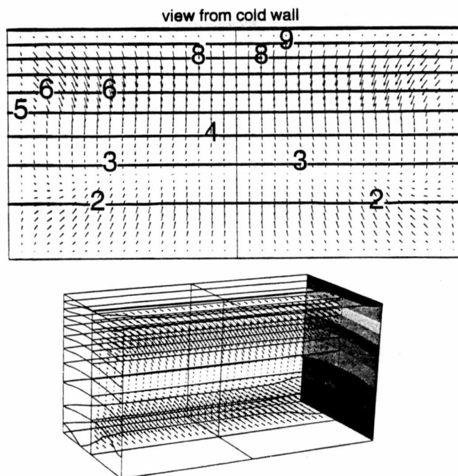
Figure 49. Vertical mid-plane Ra=1.5 \times 10^5 Pr=0.71 : press. -1.72 \times 10^{-6}(4.52 \times 10^{-7})2.80 \times 10^{-6} .
