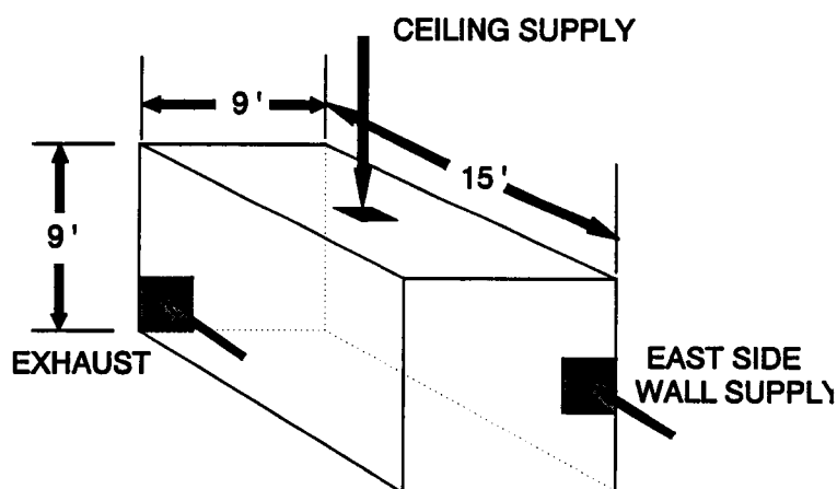
Figure 79. Schematic of U. Illinois room ventilation test facility.
