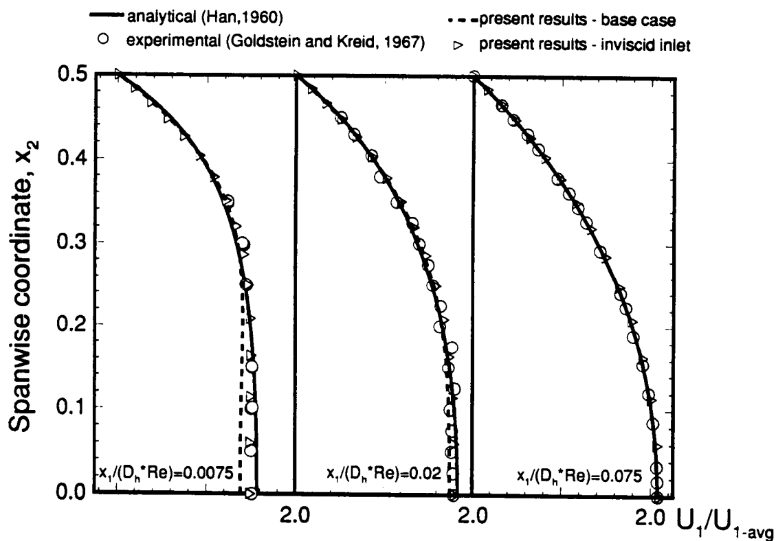
Figure 20. Developing flow in a square channel: spanwise u_1 profiles, Re=100 .
