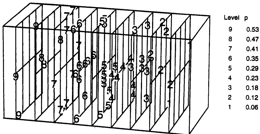
Figure 13. Fully-developed channel flow: pressure contours at Re=100 .
