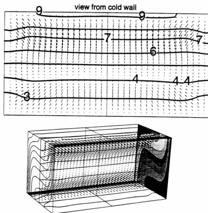
Figure 47. Vertical mid-plane Ra=1.5 \times 10^5 Pr=0.71 : temperature \theta(0.1)1 .
