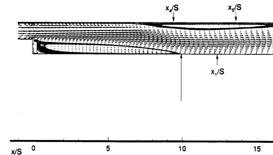
Figure 58. Present results for 2-dimensional simulations.
