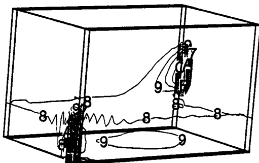
Figure 90. Total pressure for 15 ACH.
