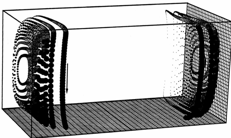
Figure 35. Particle tracks for Ra=10^4 Pr=100 .
