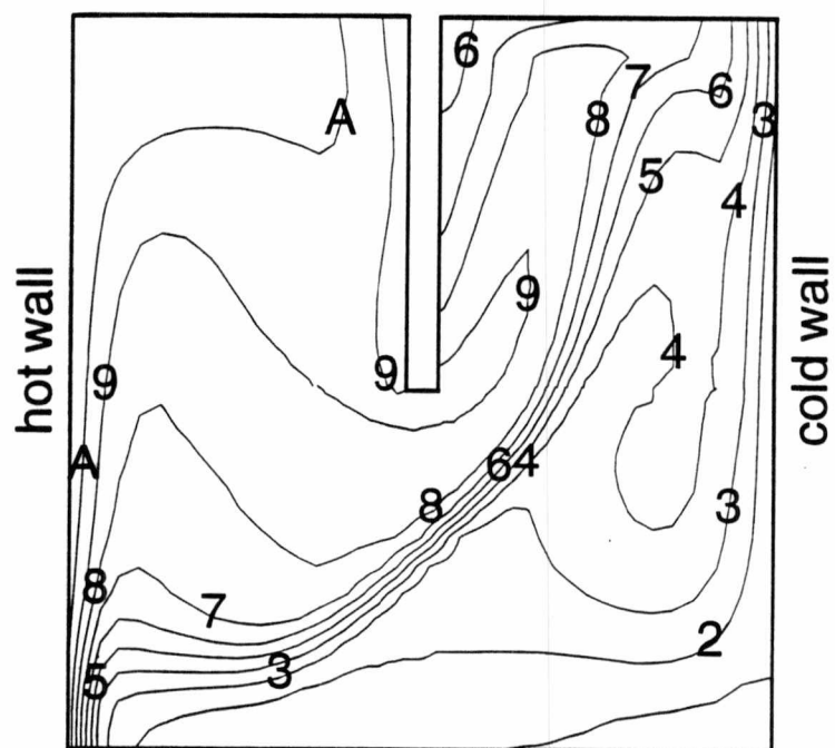
(b) temperature distribution on symmetry plane
