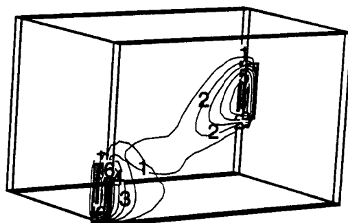
Figure 91. Isovels for 15 ACH.
