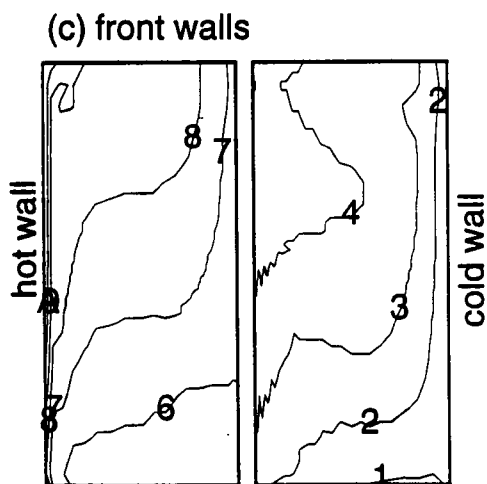
Figure 118. Isotherms on selected vertical planes - Ra=3.2 \times 10^{10} .
