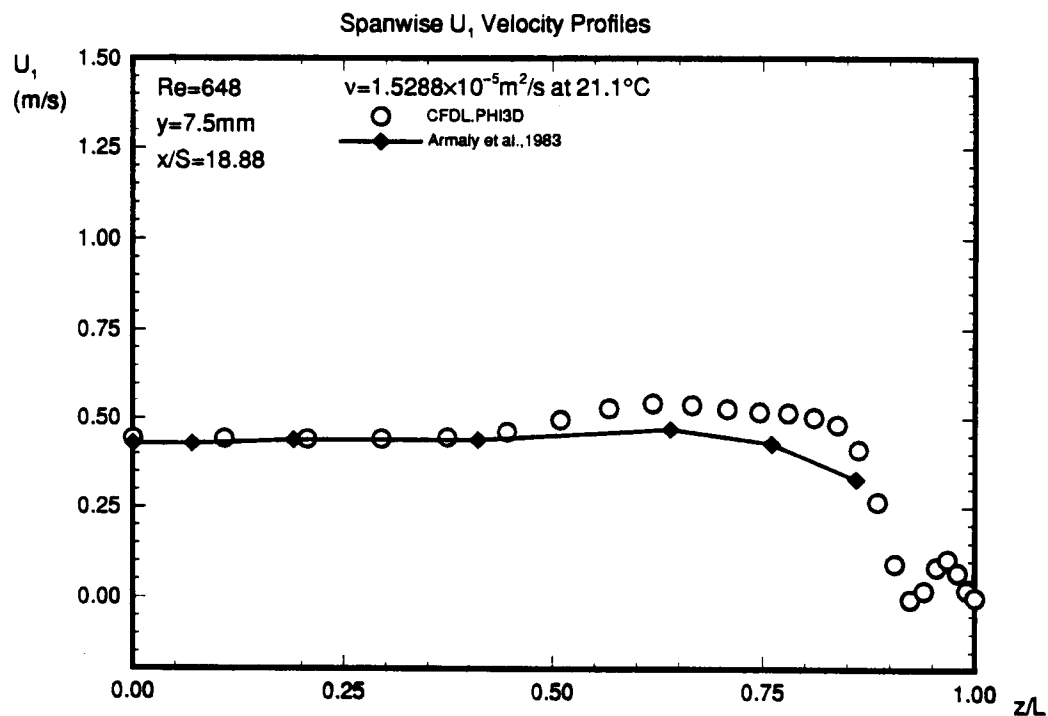
Fig. 66. (continued) Spanwise velocity profiles, Re=648 y = 7.5 mm.
