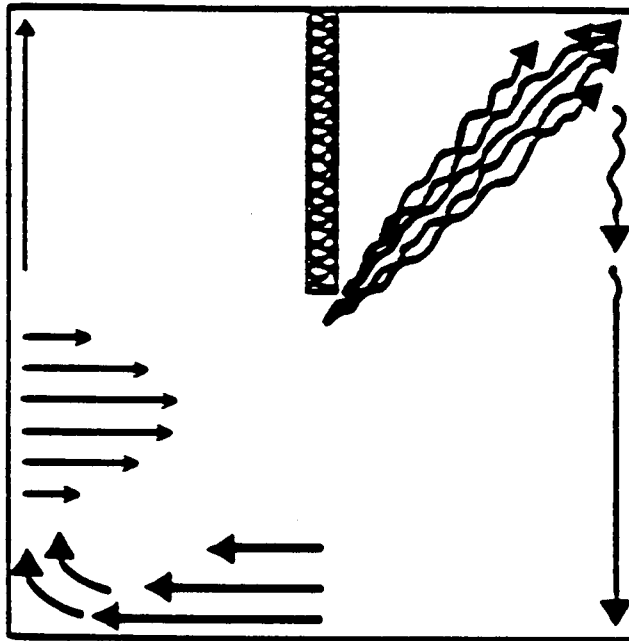
Figure 107. Flow visualization in the water cell, w/W=0.01 (Neymark, 1988).
