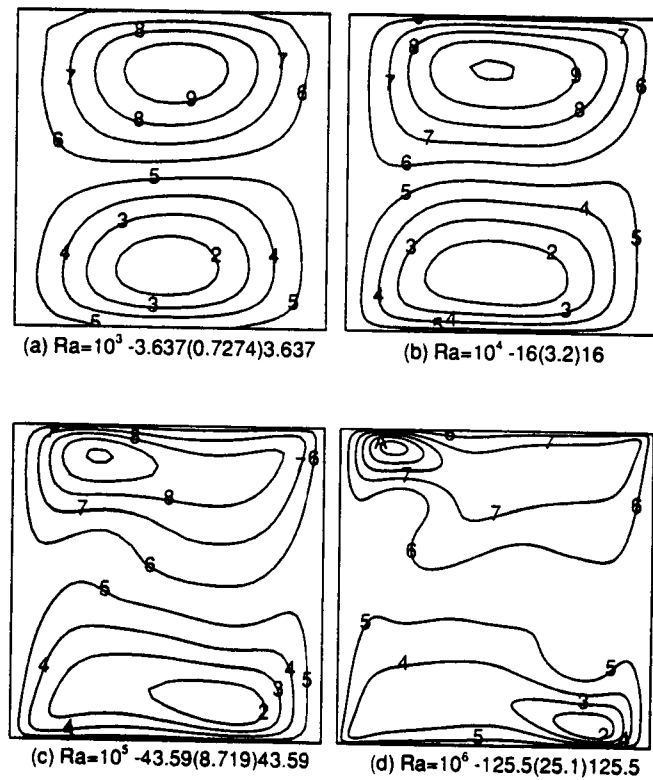
Figure 28. Contours of horizontal u_x velocity component, present data.
