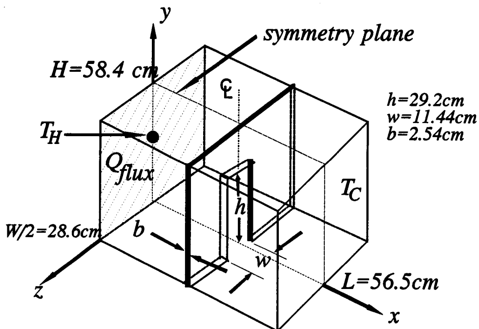
Figure 106. Geometry of small-scale water model.
