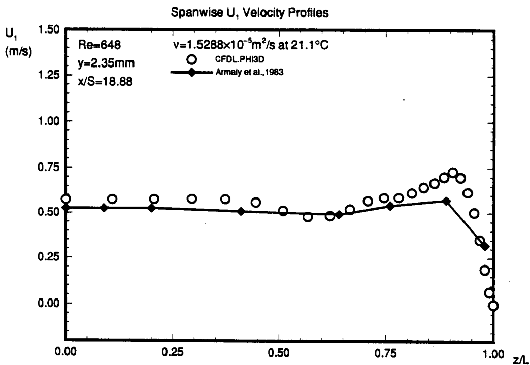
Fig. 67.(continued)Spanwise velocity profiles, Re=648 y=2.35\text{mm} .
