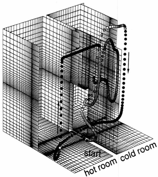
(b) side view of hot and cold zones
