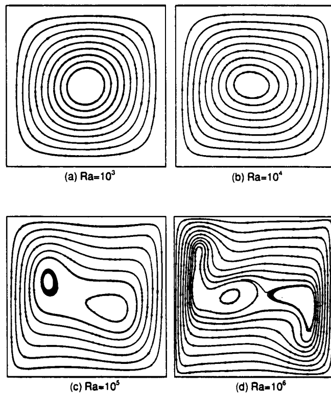
Figure 24. Streamlines computed by TECPLOT, present data.
