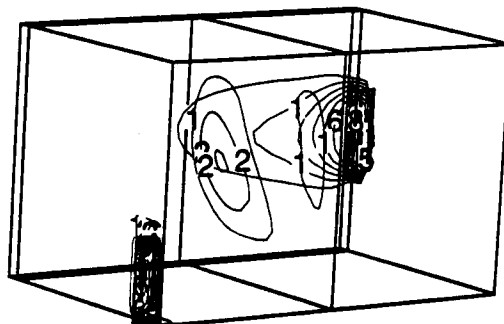
Figure 99. Isovels for 30 ACH.
