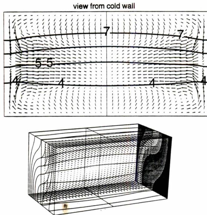
Figure 38. View of vertical mid-plane Ra=10^4 Pr=0.1 : temperature 0(0.1)1.
