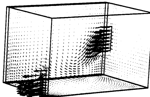
Figure 85. Velocity solutions for 15 ACH.
