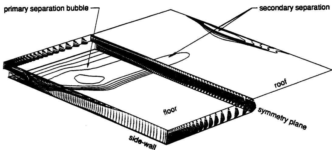
Figure 70. Separation region "footprints", Re=648 .
