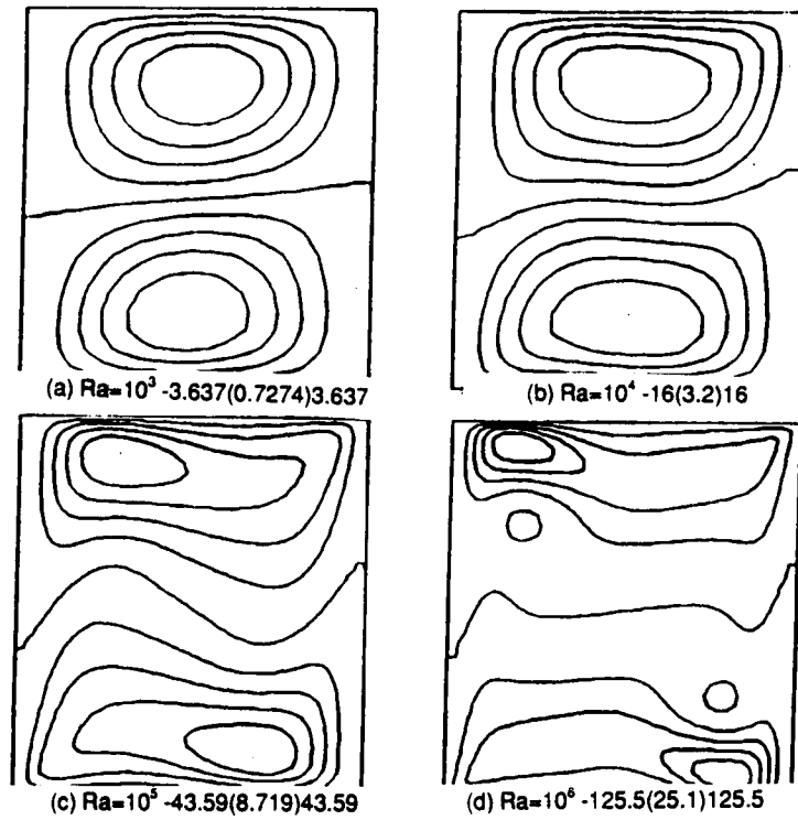
Figure 27. Contour horizontal u_x velocity component, de Vahl Davis (1983).
