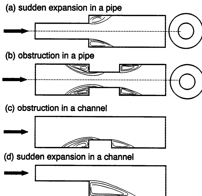
Figure 50. Test bed configurations for flow separation.
