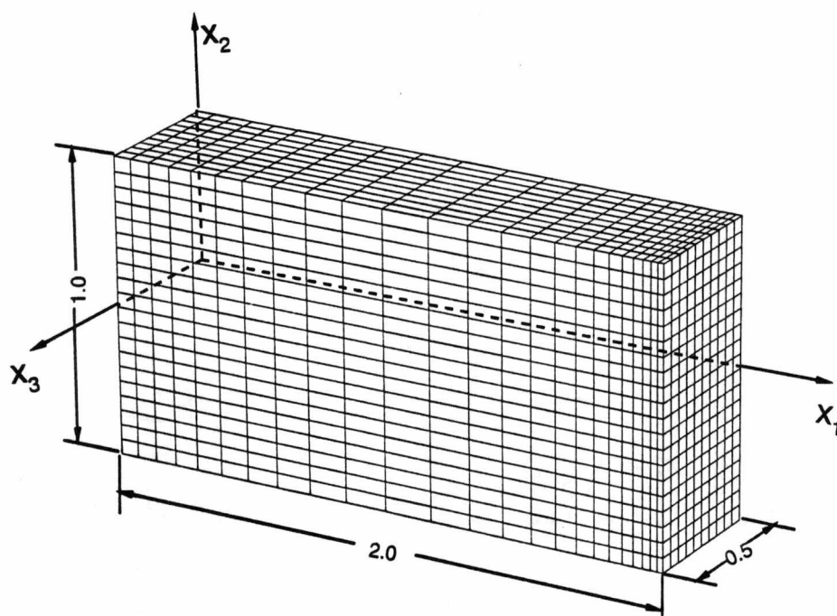
Figure 9. Fully-developed channel flow: mesh layout for M=24 \times 20 \times 10 .
