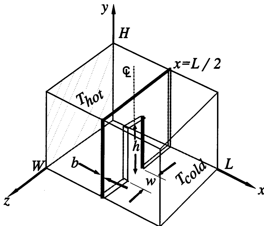
Fig. 105. Geometry for a partially-divided enclosure.
