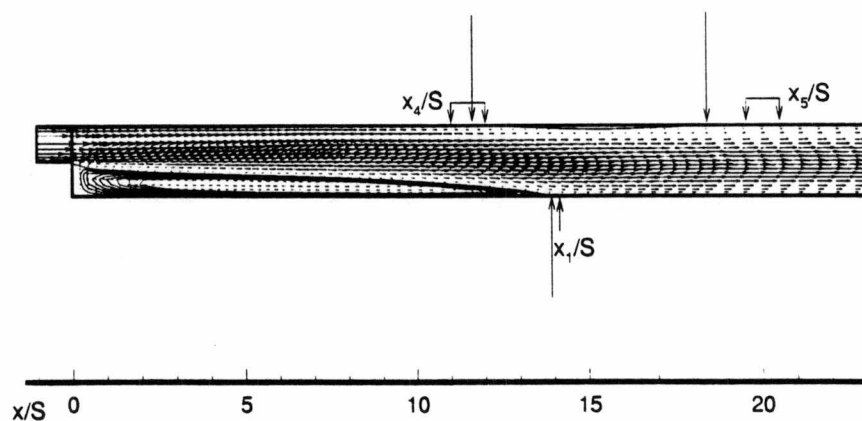
Figure 61. Present results of 3-dimensional model at symmetry plane.
