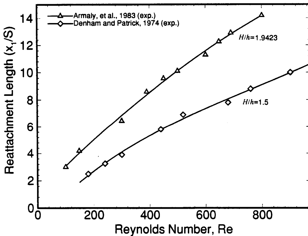
Figure 55. Experimental reattachment length data, x_r/S v. Re = UD/\nu .
