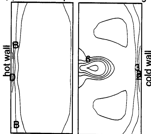
Figure 119. Isotherms on selected horizontal planes - Ra=3.2 \times 10^{10} .
