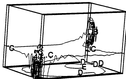
Figure 89. Isobars for 15 ACH.
