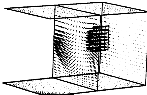
Figure 95. Transverse plane for 30 ACH.
