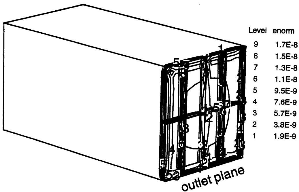
Figure 14. Fully-developed channel flow: \|\Phi\|_E distribution at Re=100 .
