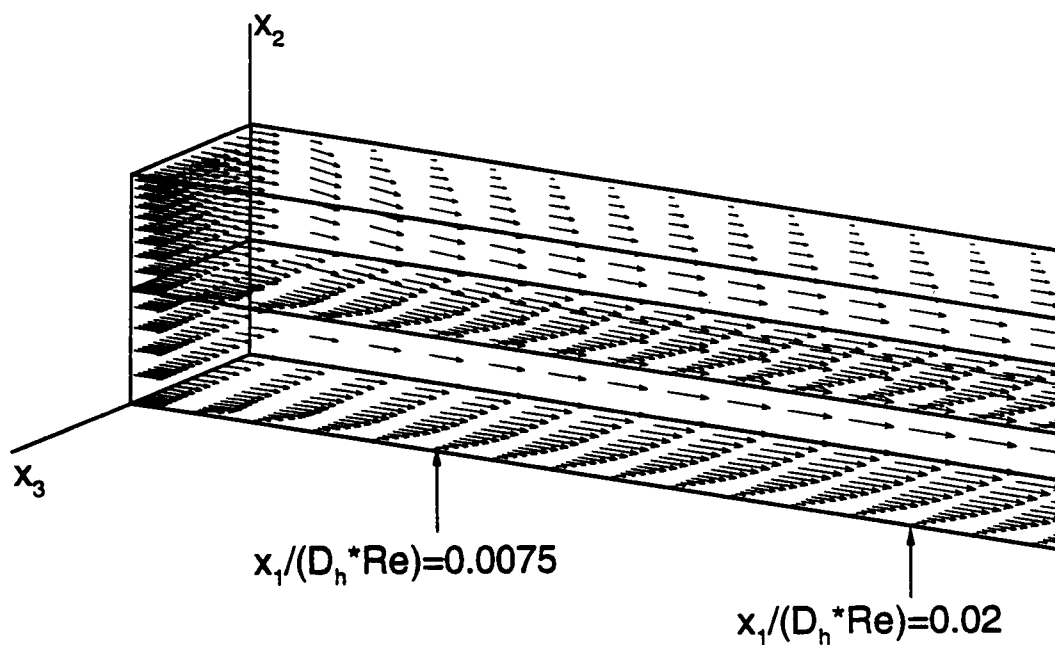
Figure 17. Developing flow in a channel: velocity vector field near entrance, Re=100 .
