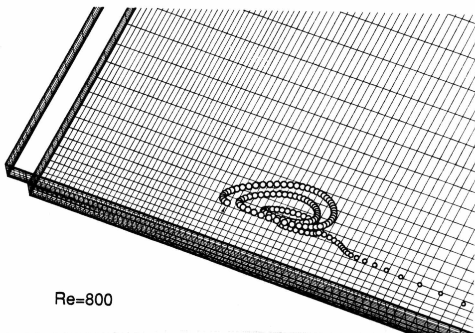
Figure 78. Lagrangian particle track, release point near vertical-axis vortex structure at roof, Re=800.
