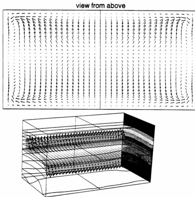
Figure 48. Horizontal mid-plane Ra=1.5 \times 10^5 Pr=0.71 : press. -1.72 \times 10^{-6}(4.52 \times 10^{-7})2.80 \times 10^{-6} .
