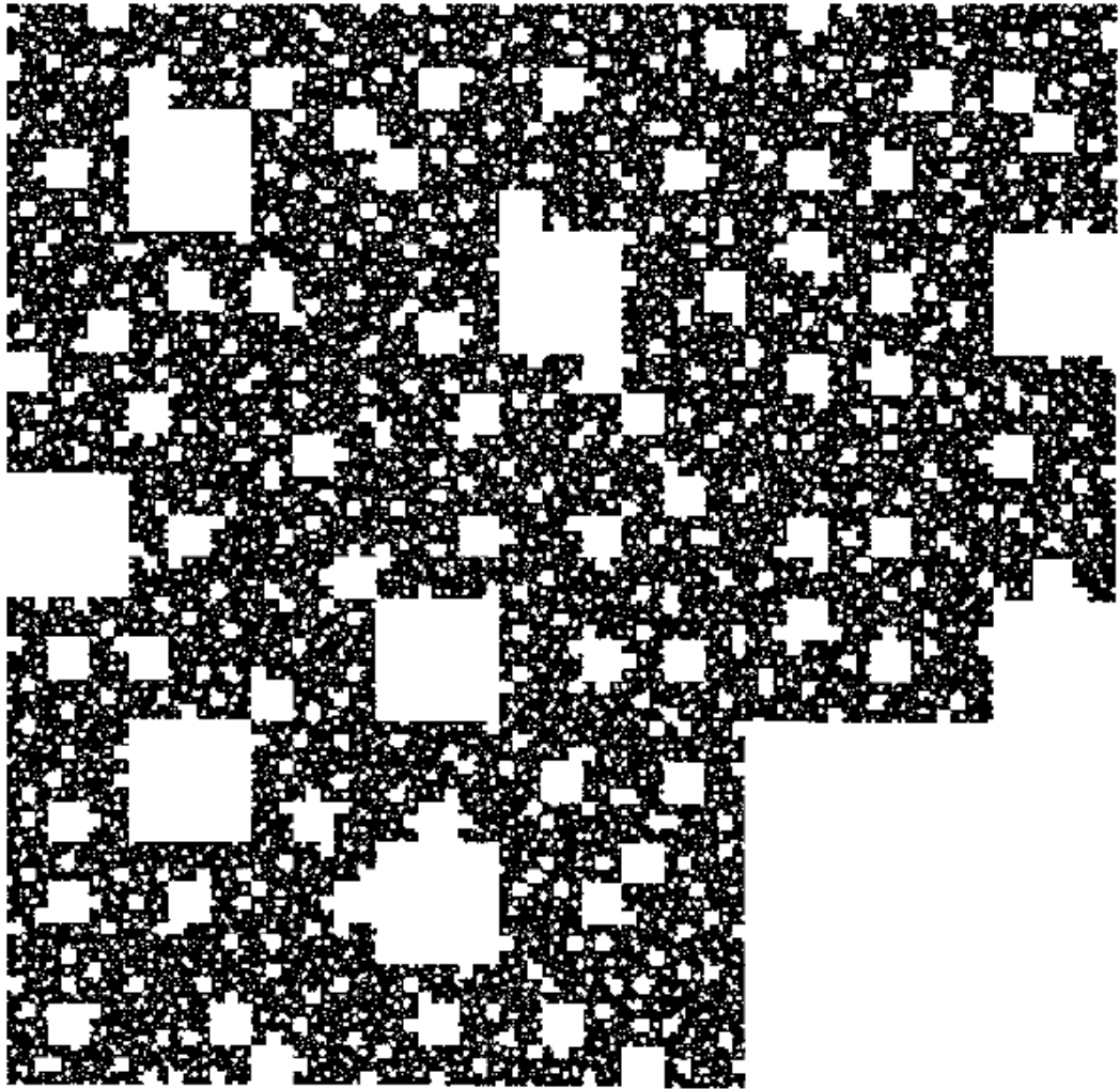
Figure 4.3 Random Sierpinski Carpet. D_f=1.89 Reprint Courtesy Sukop et al. [4d]
