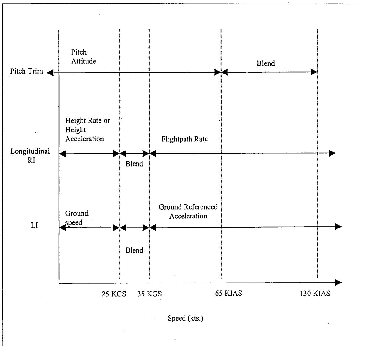
FIGURE A-21 UNIFIED CONTROL MODE
