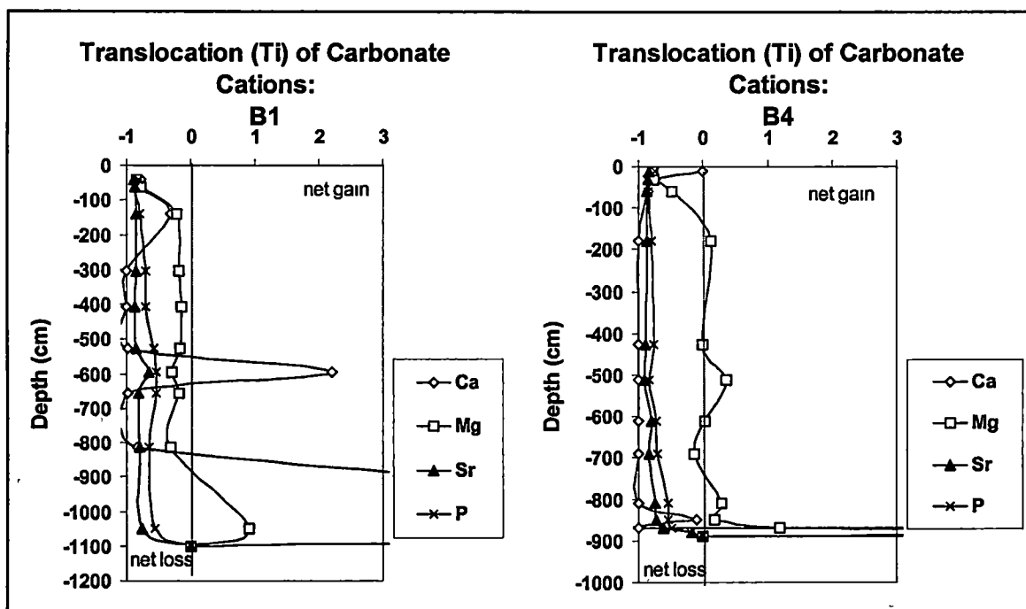
Figure 21: Transport functions (translocation) for carbonate elements in boreholes 1 and 4 calculated using immobile Ti. Negative values represent net loss of constituent relative to parent material with -1 equivalent to 100% loss, and +1 is 100% net gain.
