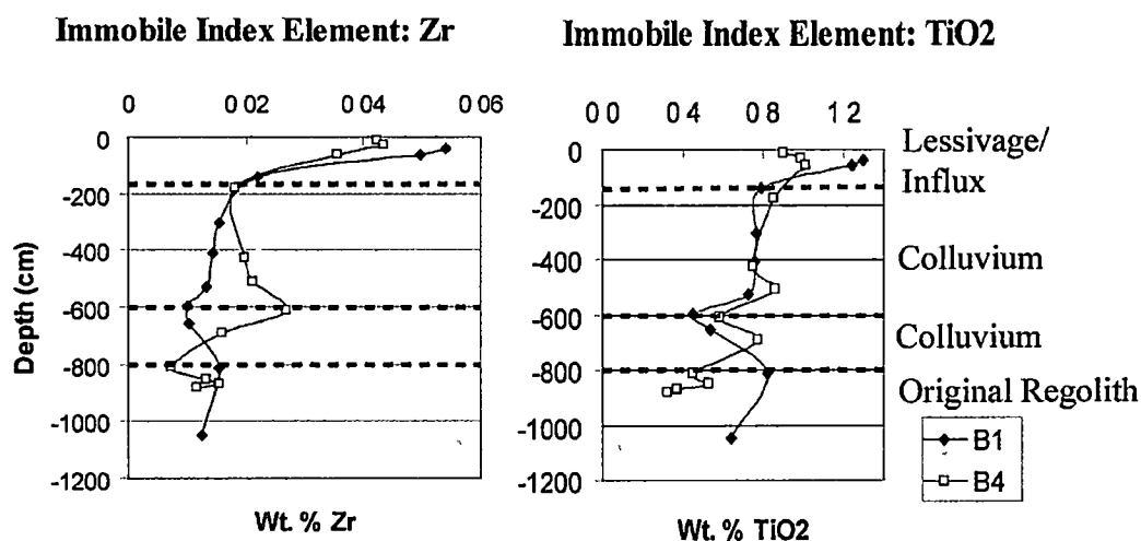
Figure 13: Distributions of immobile elements Zr and \text{TiO}_2 vs. depth for boreholes 1 and 4 and interpretations for origins of weathered materials. Note that the concentration of \text{TiO}_2 shows less variation with depth.
