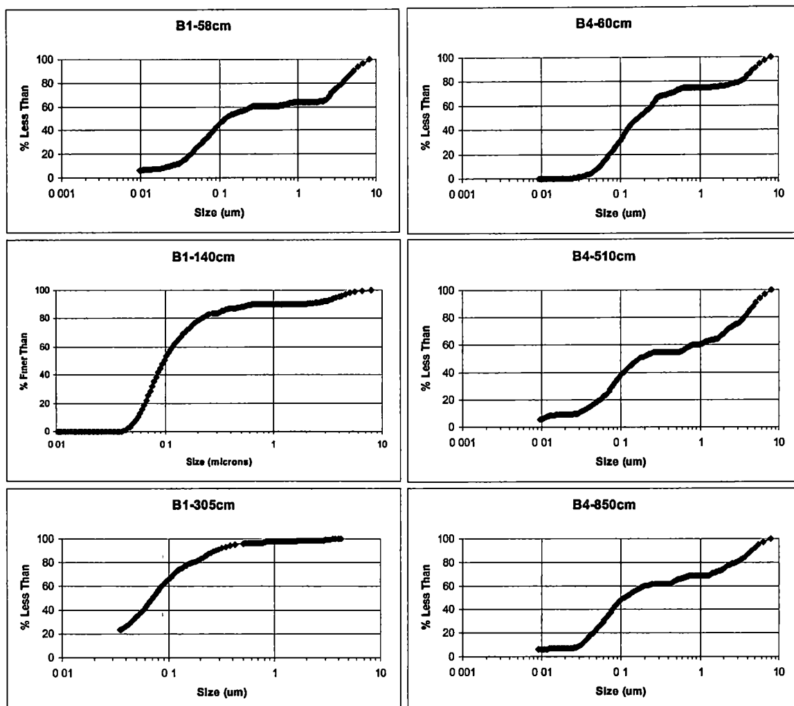
Figure 12: Examples of detailed cumulative clay distribution curves for boreholes 1 and 4. Note the subtle/weak fine silt and pedogenic clay bimodal distribution.
