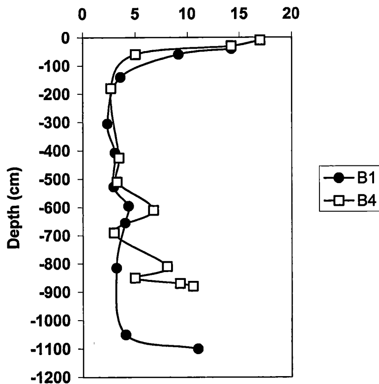
Figure 17: Whole-rock XRF data for Silicon / Sequioxides ratios exemplifying hydration-driven weathering reactions in boreholes 1 and 4.
