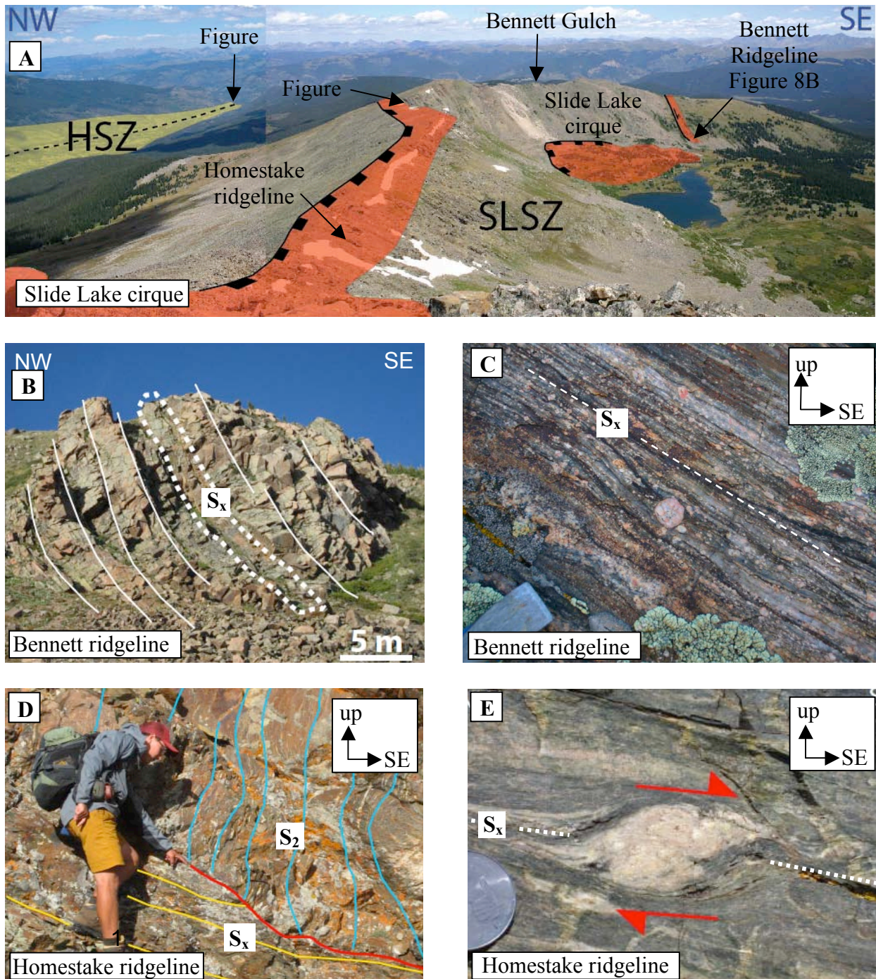
Figure 8. Field observations of the SLSZ. (A) View towards the northeast along the Continental Divide; three major splays (highlighted red) of the SLSZ. (B) Bennett ridgeline outcrop, mylonite splay dashed and parallel to the surrounding foliation (C) Bennett ridgeline mylonite. (D) Fabric truncation between the steep fabric ( S_2 ) within the hanging wall of the upper splay and the subhorizontal fabric ( S_x ) of the SLSZ. (E) Porphyroclasts within quartz-calcite-biotite mylonite from the upper splay, top-down-to-the-southeast motion.
