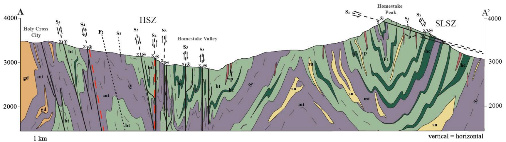
Figure 6. Geologic cross section of the field area (A-A'). Figure shows the multiple generations of foliation exposed in the field area: S 1 early melt present foliation; S 2 /F 2 upright folds; S 3 mylonite; S 4 ultramylonite and pseudotachylite (red-dashed line); and S x SLSZ fabric. Sense of shear denoted by arrows for vertical motion and "x" and "o" for lateral displacement. See Figure 2 and Plate 1 for explanation.
