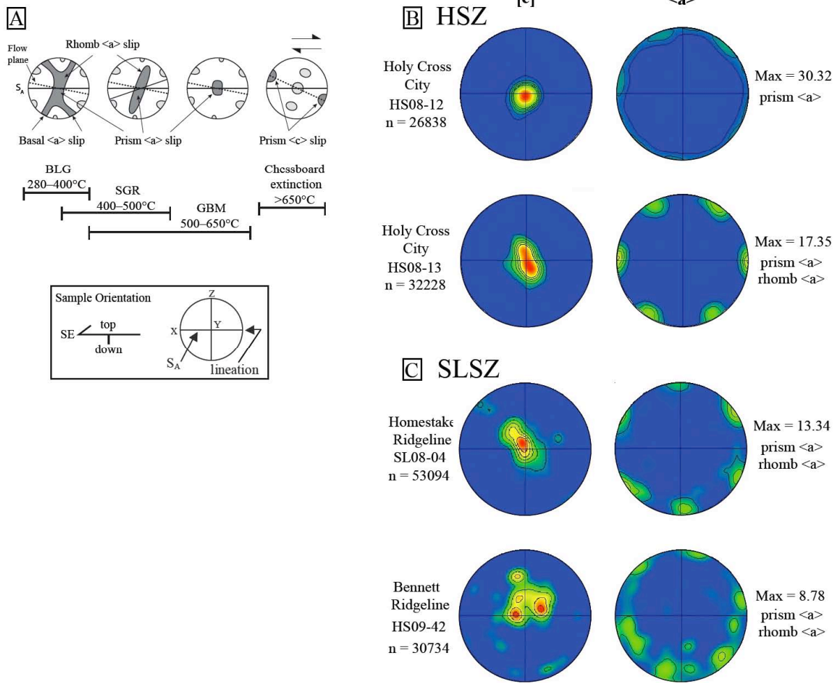
Figure 12. (A) Pole diagrams showing quartz LPO patterns for the [c] axes and <a> axes with increasing temperature for non-coaxial, plane strain deformation (after Stipp et al., 2002b; Passchier and Trouw, 2005; Langille et al., 2010a). (B) EBSD generated lattice-preferred orientations for HSZ (qtz+fsp) mylonite (HS08-12, HS08-13) displaying patterns characteristic of plane strain and prism <a> slip and (C) SLSZ sample SL08-04 displaying prism <a> slip and plane strain patterns and HS09-42 displaying non-plane strain conditions with possible prism <a> and rhomb <a> slip.
