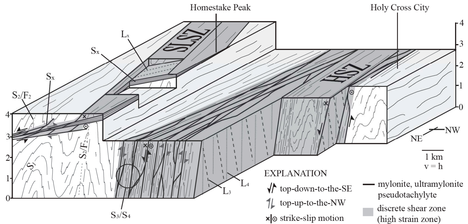
Fig. 17. Block diagram of the SLSZ and HSZ viewed to the south. Lineation-foliation relationships and shear sense are displayed within the figure. Black arrows represent top-down-to-the-SE, gray arrows represent top-up-to-the-NW sense of shear. Note orientation and style of SLSZ deformation. Zones of mylonite, ultramylonite, pseudotachylyte, and high strain domains highlighted in dark gray.
