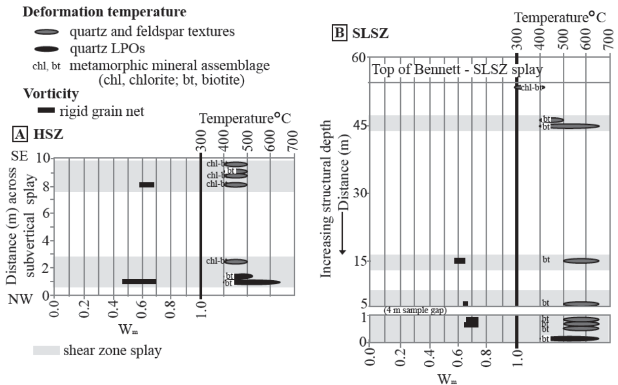
Figure 16. Deformation temperature and vorticity results from (A) HSZ Holy Cross City transect and (B) SLSZ Bennett ridgeline transect. Each rectangle and ellipse represents one sample. Data can be found in Appendix I and IV.
