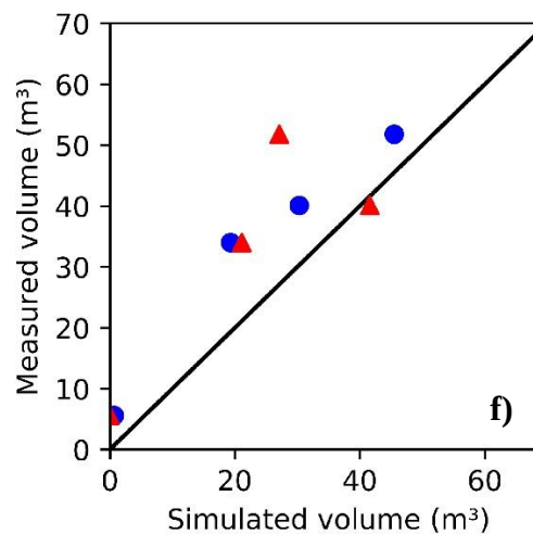
Figure 3.5. Measured and modeled drainage and overflow volumes from both DRAINMOD-Urban and SWMM under three simulations: uncalibrated, volume-calibrated and hydrograph-calibrated.
