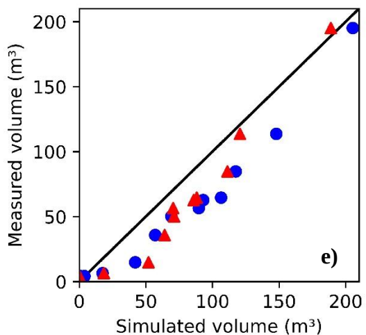
Figure 3.5. Measured and modeled drainage and overflow volumes from both DRAINMOD-Urban and SWMM under three simulations: uncalibrated, volume-calibrated and hydrograph-calibrated.
