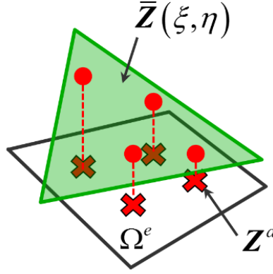
Figure 2-1. Elemental projection of elastic rotation \mathbf{Z}
