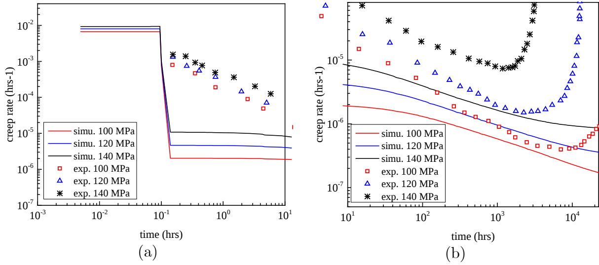
Figure 3-4. Macroscopic cell strain rate (/h) versus model time (h) for cell model without grain boundaries as a function of remote applied stress. (a) early portion of the creep response; (b) later portion of the creep response.
