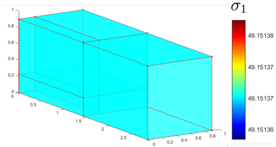
Figure 6-5. Contour plot of the first principle stress.
