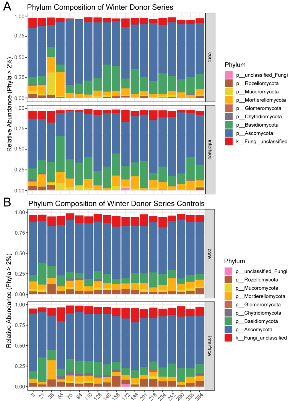
Figure 3.15: Phylum composition of winter trial soils. Relative abundances of phyla in cores and interfaces are shown for (A) impacted soils and (B) controls.
