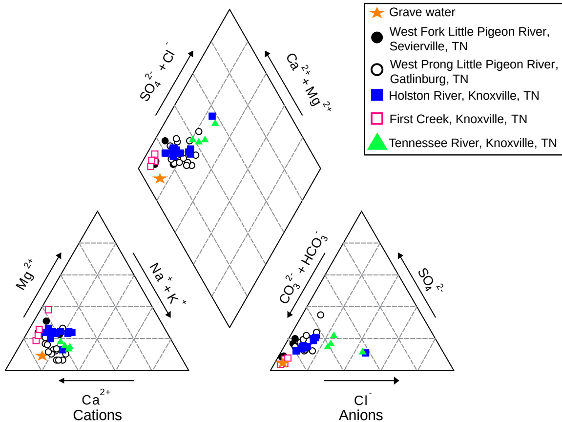
Figure 1.7: Piper diagram for grave water and nearby surface water geochemistry. Water samples from five East Tennessee rivers and the grave water are geochemically similar, and are predominantly \text{Ca-Na-K-HCO}_3^- type waters. Surface water geochemistry was obtained through the USGS (Water for the Nation, https://waterdata.usgs.gov/nwis ), selecting samples from nearby rivers (less than 50 miles away), with complete water geochemistry provided (including pH, temperature, total dissolved solids, bicarbonate), and ionic charge balance of \pm 17\% . The resulting dataset included 40 surface samples plus the grave water.
