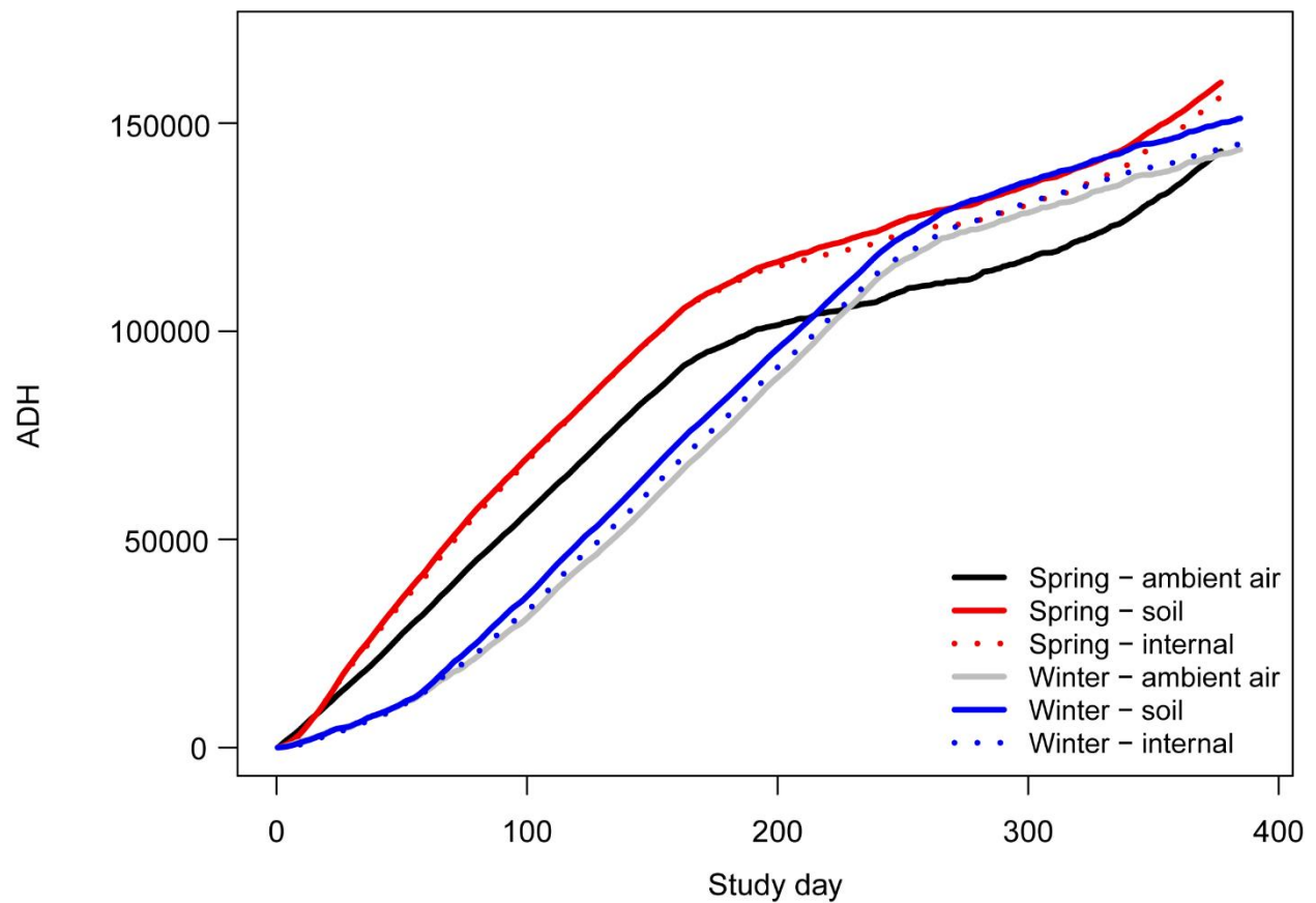
Figure 3.2. Accumulated degree hours (ADH) for environmental temperature probes shown by study day for spring and winter donor trials. Cumulative temperatures for internal and soil probes diverged from cumulative ambient air temperatures during the spring study partially due to insect-thermogenesis (red and black lines). In the absence of insect activity, this trend was reduced in the winter study.
