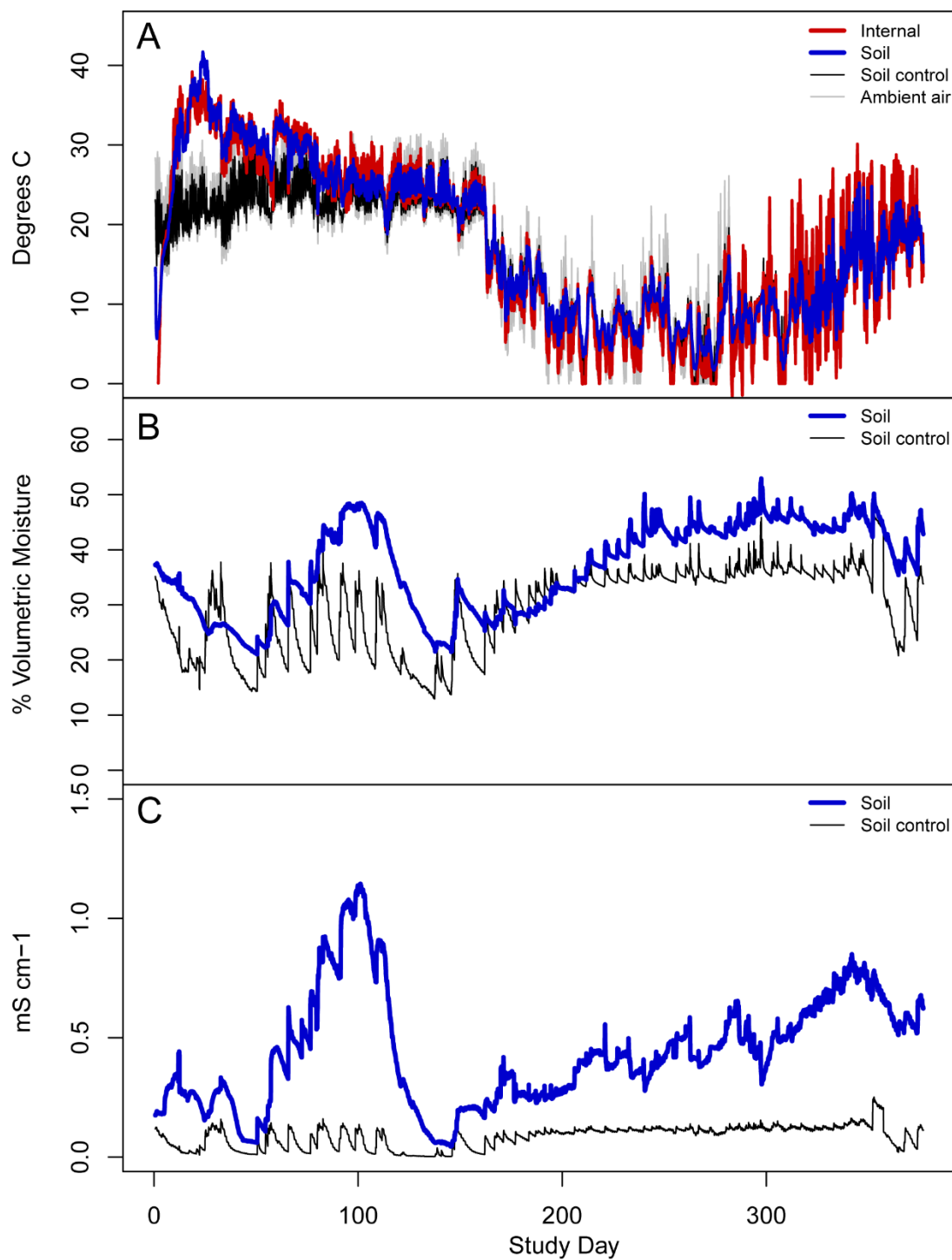
Figure 3.1: Soil sensor data from spring donor series. Temperature (A), soil moisture (B), and soil electrical conductivity (C) are shown by study day. Controls are shown in black and soil data shown in blue. For temperature data, ambient air is shown in grey, and donor internal temperatures are shown in red.
