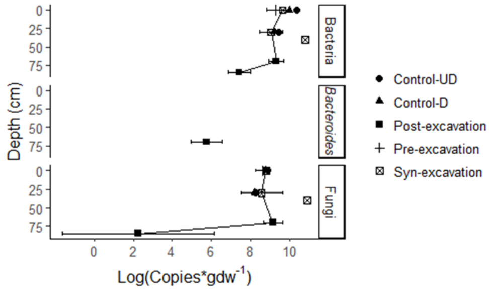
Figure 1.9: Gene copy abundances of Total 16S rRNA (Bacteria), Bacteroides 16S rRNA ( Bacteroides ), and ITS (Fungi) within the grave. Bacteroides were below detection in all but the 70-75 cm samples.
