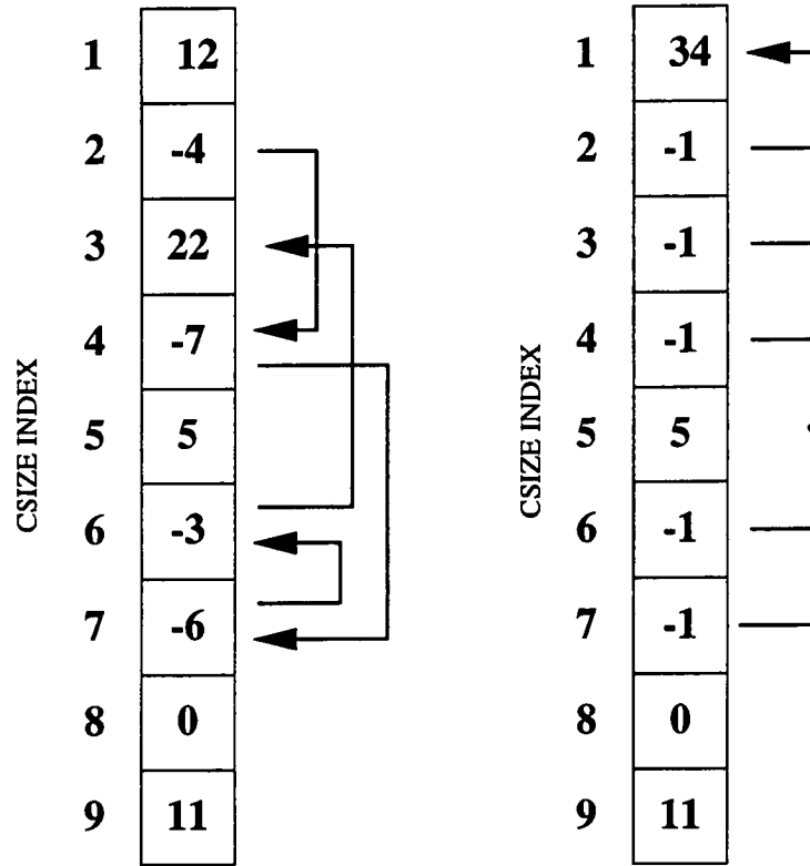
Figure 2.5: Example of search path compression in the csize array before (left) and after (right) a merge operation. The operation merged the temporary cluster labeled 2 into the temporary cluster labeled 1. This operation followed a 5-step pointer path ( 2 \rightarrow 4 \rightarrow 7 \rightarrow 6 \rightarrow 3 ) to determine that temporary cluster labeled 2 was actually temporary cluster labeled 3 and contains 22 pixels.
