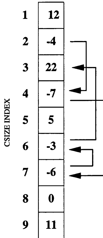
Figure 2.2: The csize working array illustrating either a positive or negative value for each index in the array. Positive values are a count of the pixels in the cluster labeled with the array index value and negative values are pointers to other indexes in the array. Negative indexes can follow a non-circular, recursive path for a finite number of steps.
