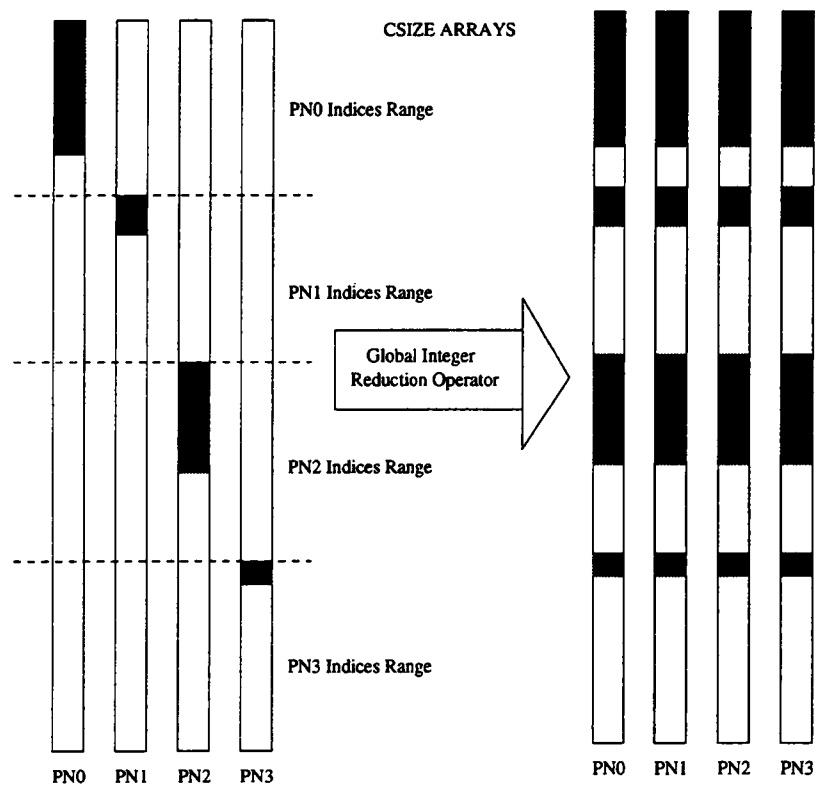
Figure 3.1: Illustration of index ranges in the csizes array on a 4-PN system and the results of a global integer reduction operation (GIRO).
