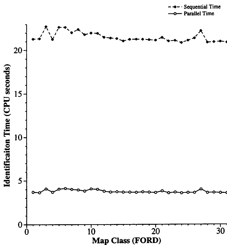
Figure 4.2: Comparison of parallel and sequential cluster identification times for 31 map classes of the FORD map. All times are elapsed CPU seconds.
