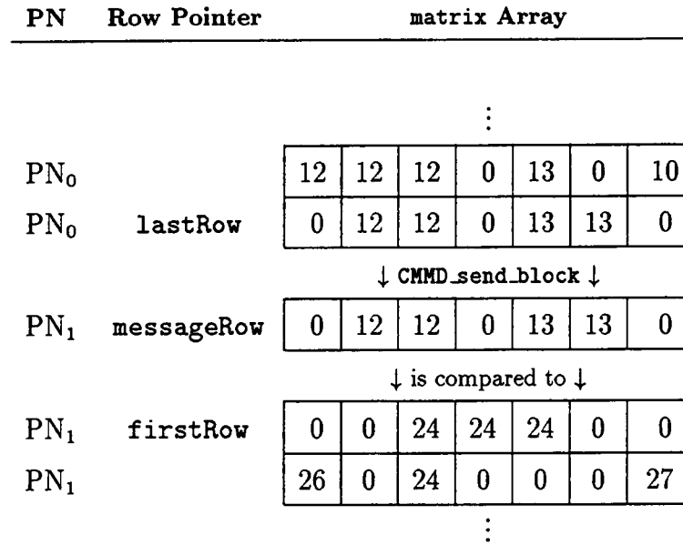
Figure 3.2: Illustration of the merge-clusters ordered pair generation. LastRow is passed from PN 0 and received by PN 1 into messageRow . messageRow is then compared to firstRow to determine overlapping clusters.
