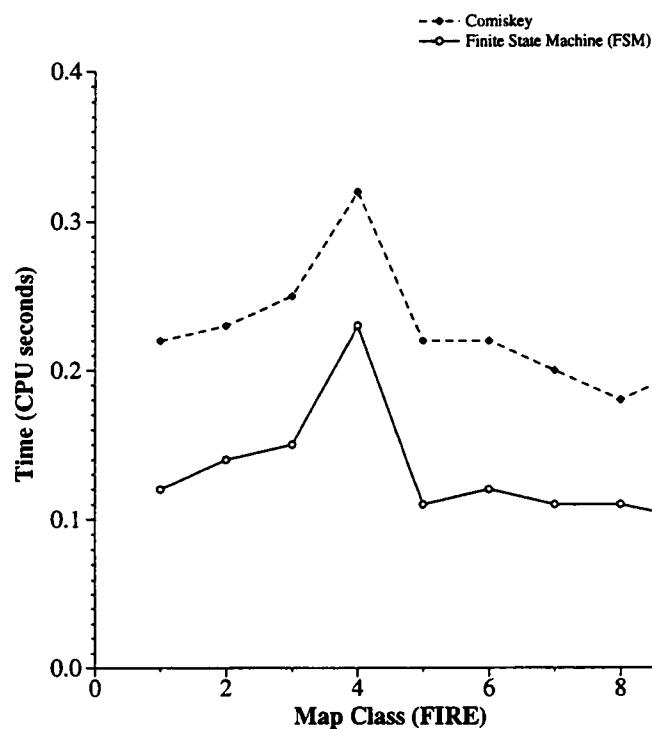
Figure 4.1: Cluster identification time for Comiskey's implementation vs. the FSM implementation. All times are in CPU seconds.
