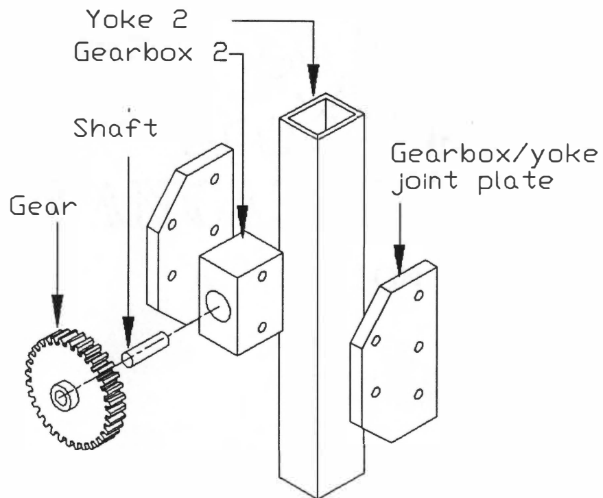
Figure 4.7 - Attachment of gear box 2 to yoke.
