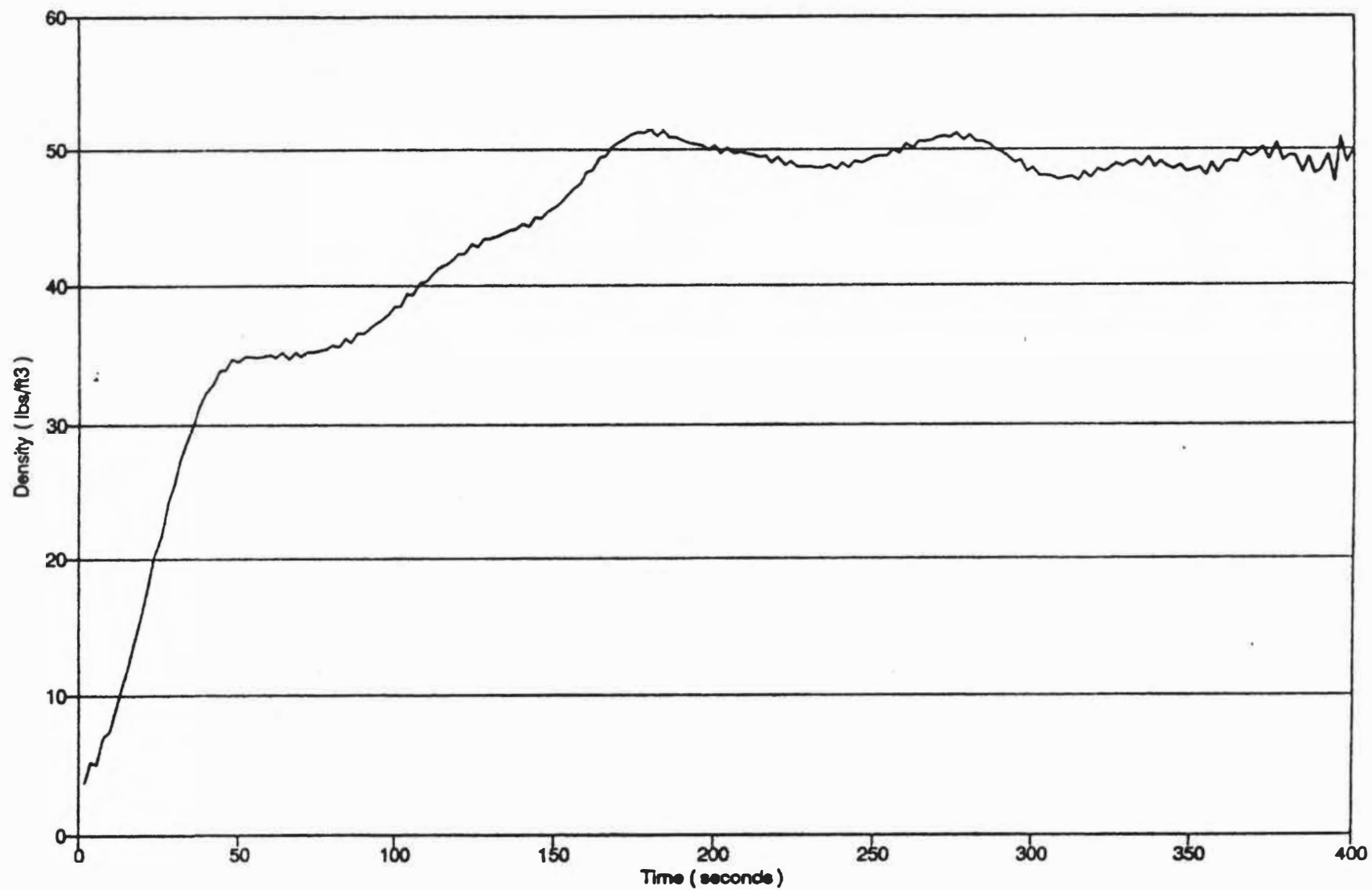
Figure 5.12 - Density during press cycle (sample:11 - width:6"), smoothed plot.
