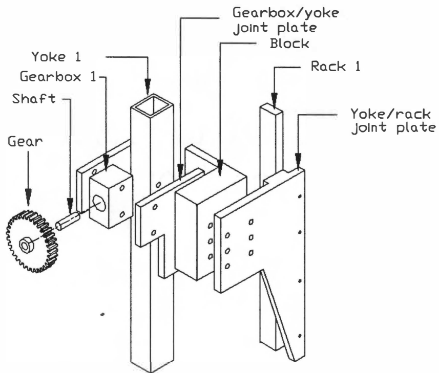
Figure 4.6 - Attachment of gear box 1 to yoke and rack.
