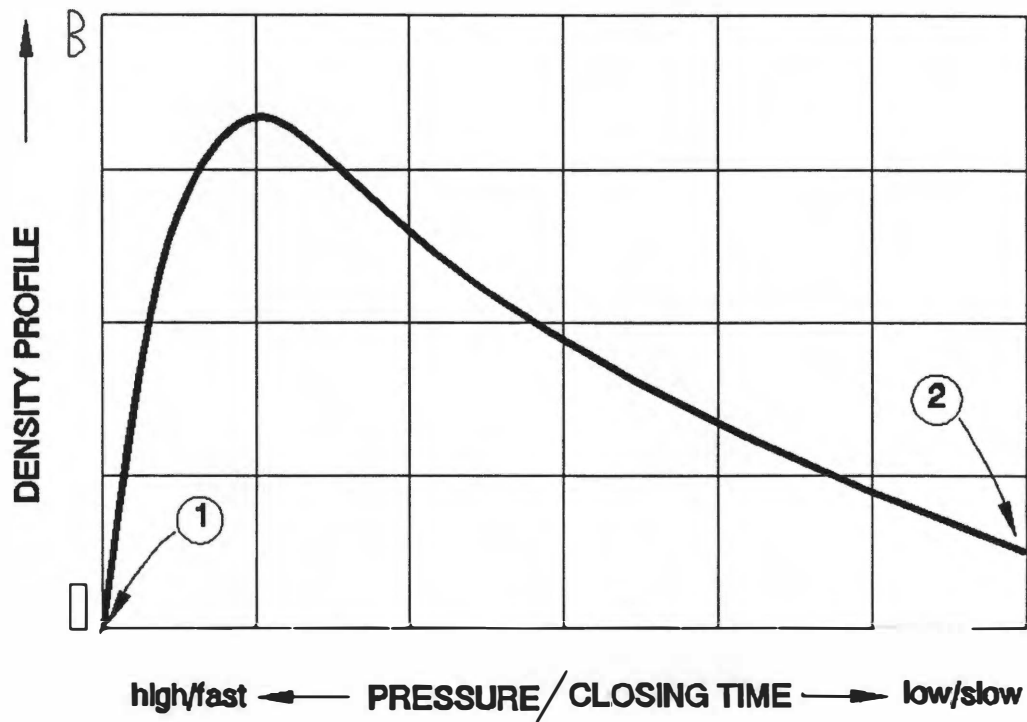
Figure 2.2 - Schematic illustration of the relationship between pressure, closing time, and density distribution over the cross-section of medium density fiberboard ( Adapted from: Suchsland and Woodson 1975).
