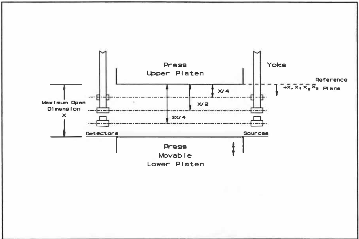
Figure 3.1 - Initial (at start of pressing operation) positions of press, and desired positioning of three radiation sources and detectors for measuring instantaneous density "in-situ" of a wood particle mat during pressing.
