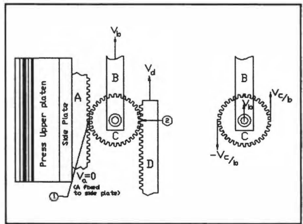
Figure 3.2 - Kinematics of rack-pinion drive.
