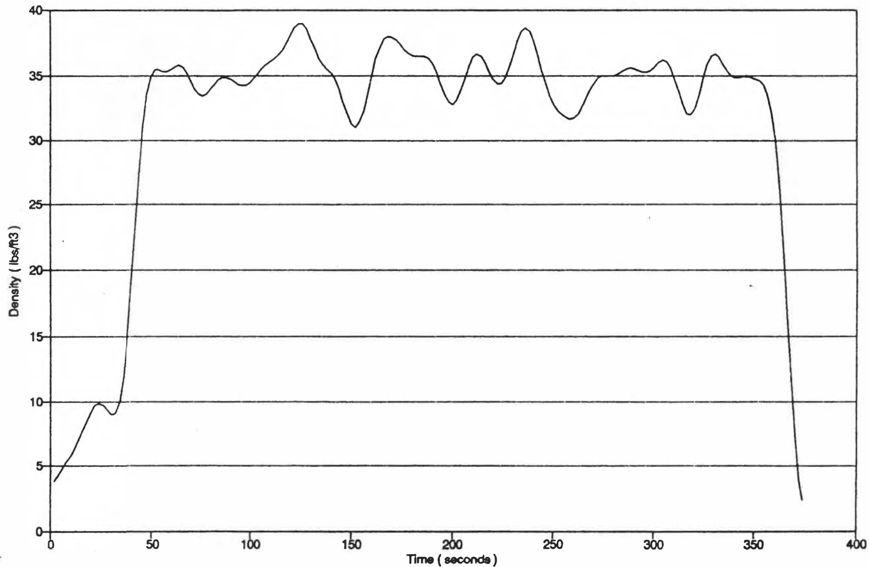
Figure 5.10 - Density during press cycle (sample:8 - width:2"), smoothed plot.
