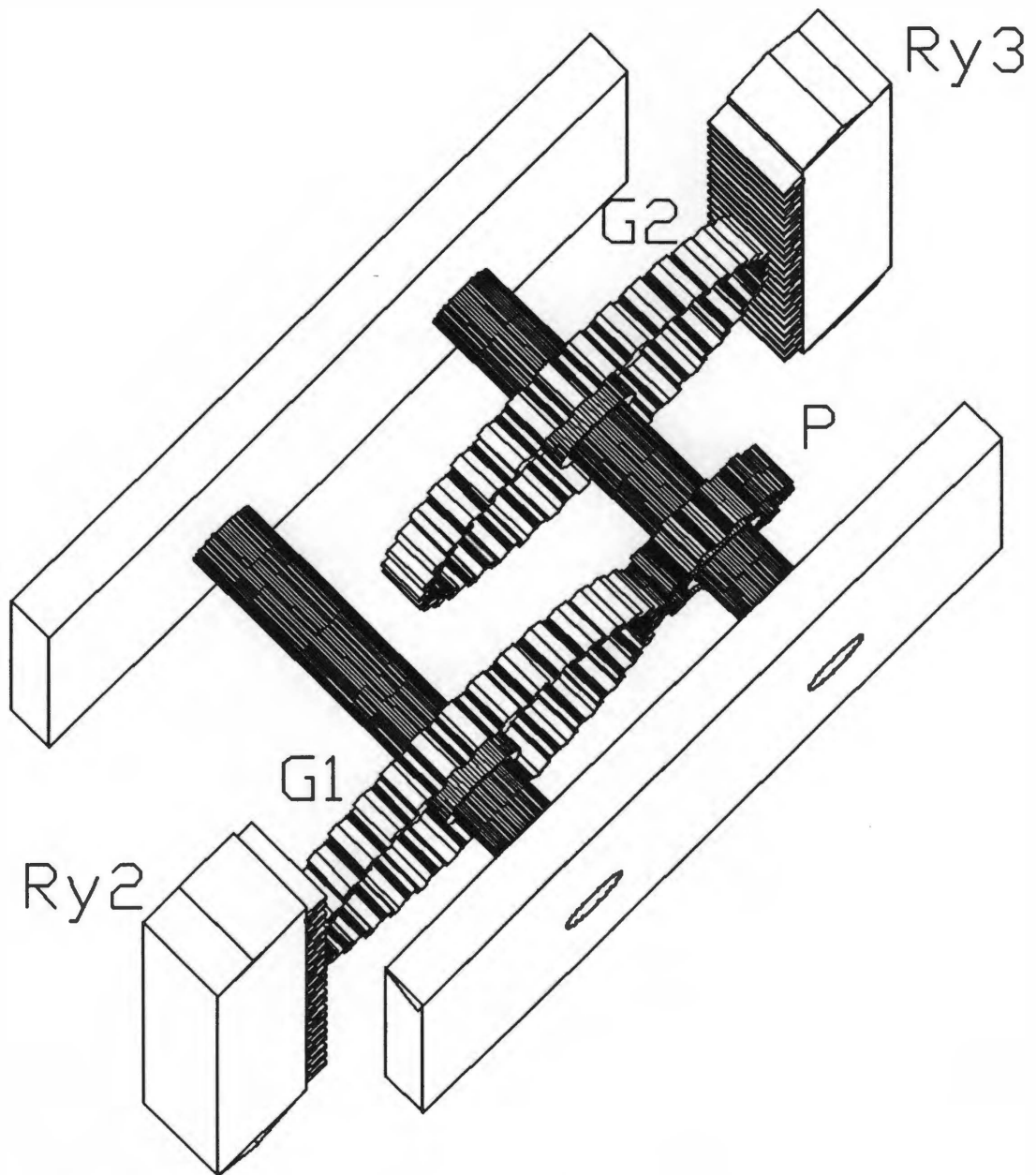
Figure 4.3 - Pictorial view of the speed multiplier mechanism.
