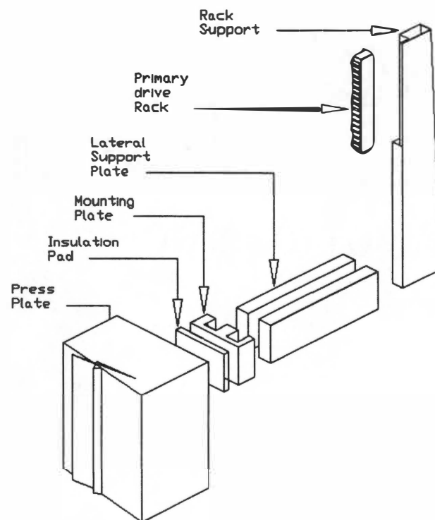
Figure 4. 8 - Primary drive components (right side shown, left side opposite).
