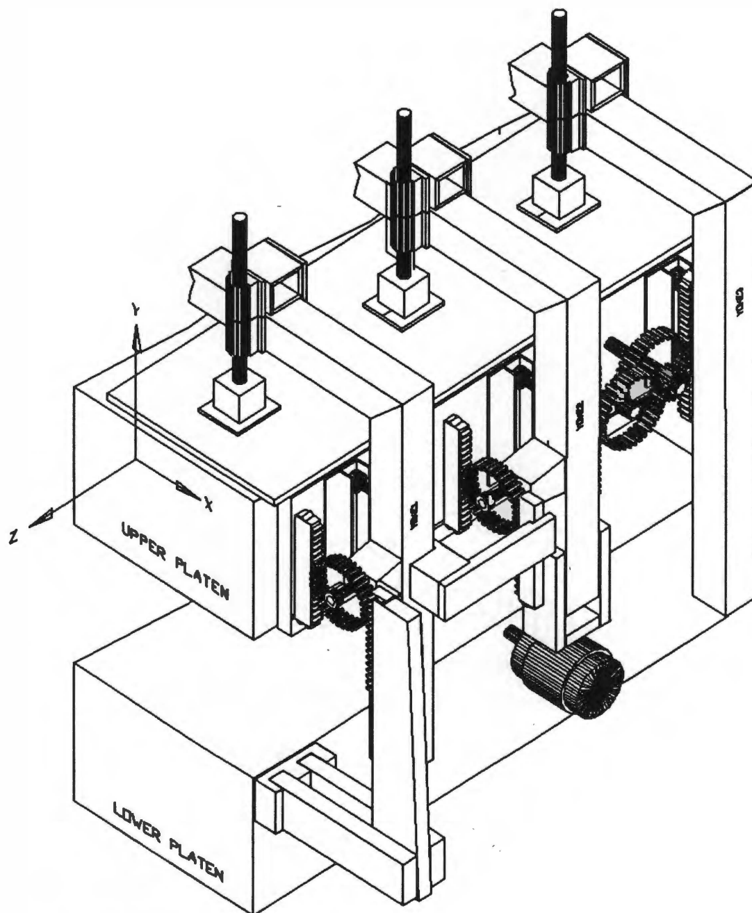
Figure 3.5 - Mechanical device on the press
