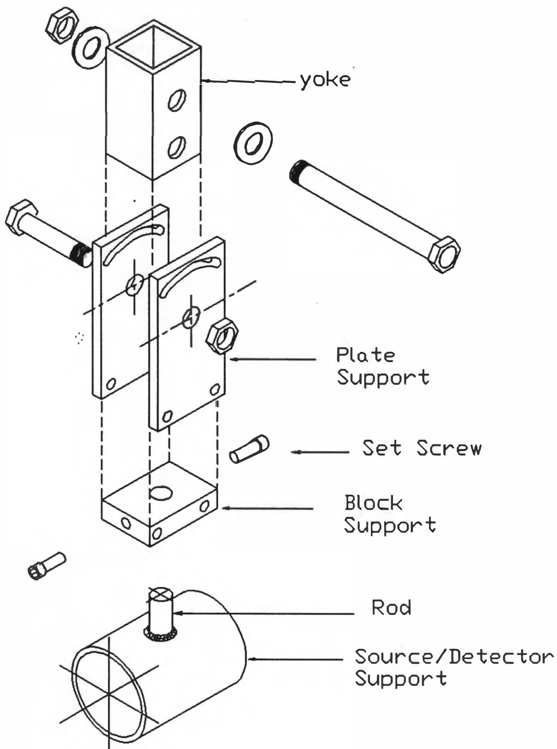
Figure 4.2 - View of the detector/source attachment assembly.
