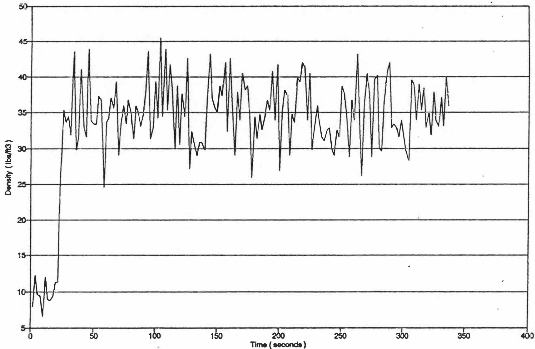
Figure 5.5 - Density during press cycle (sample:8 - width:2").
