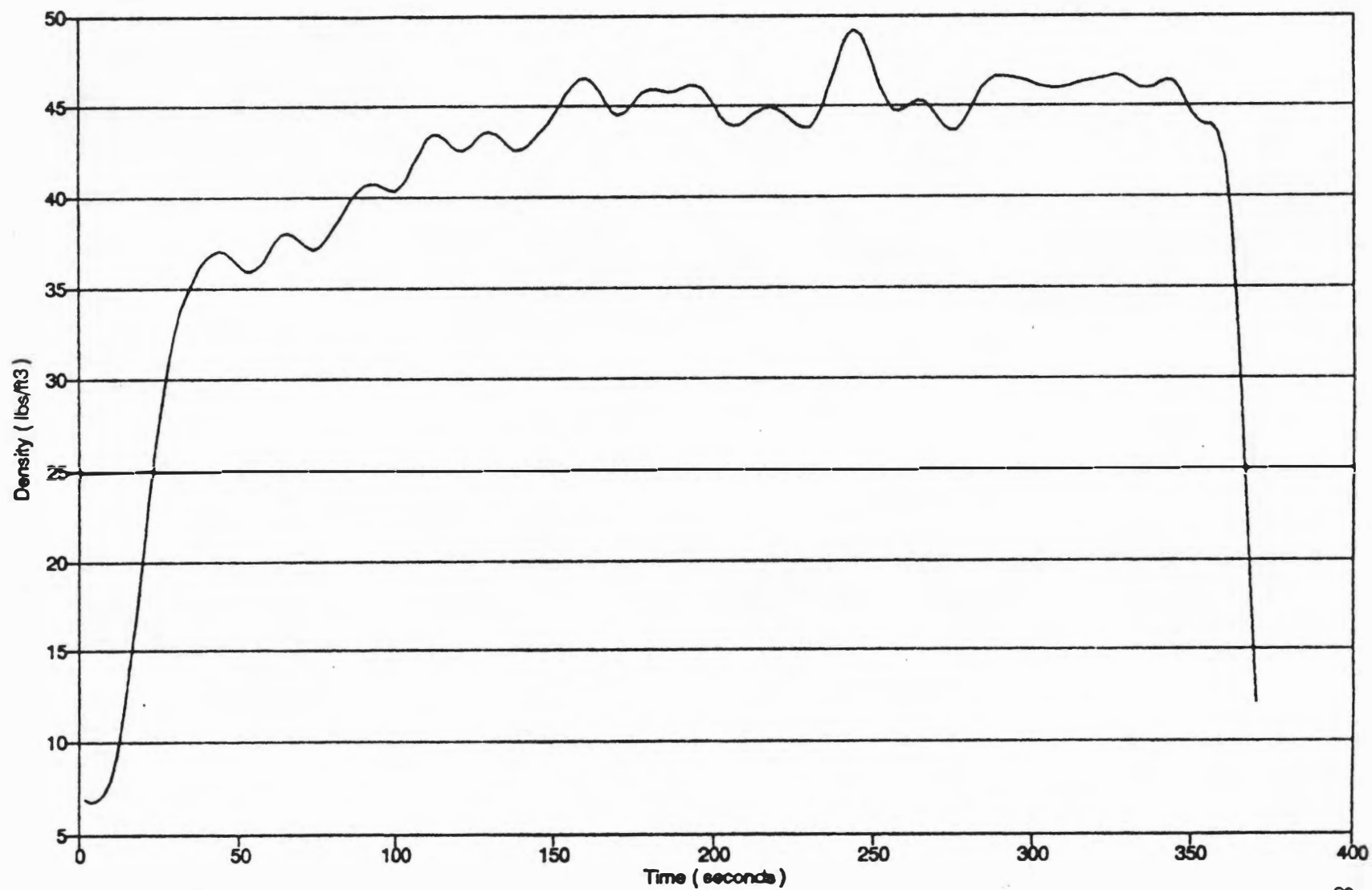
Figure 5.13 - Density during press cycle (sample:12 - width:8"), smoothed plot.
