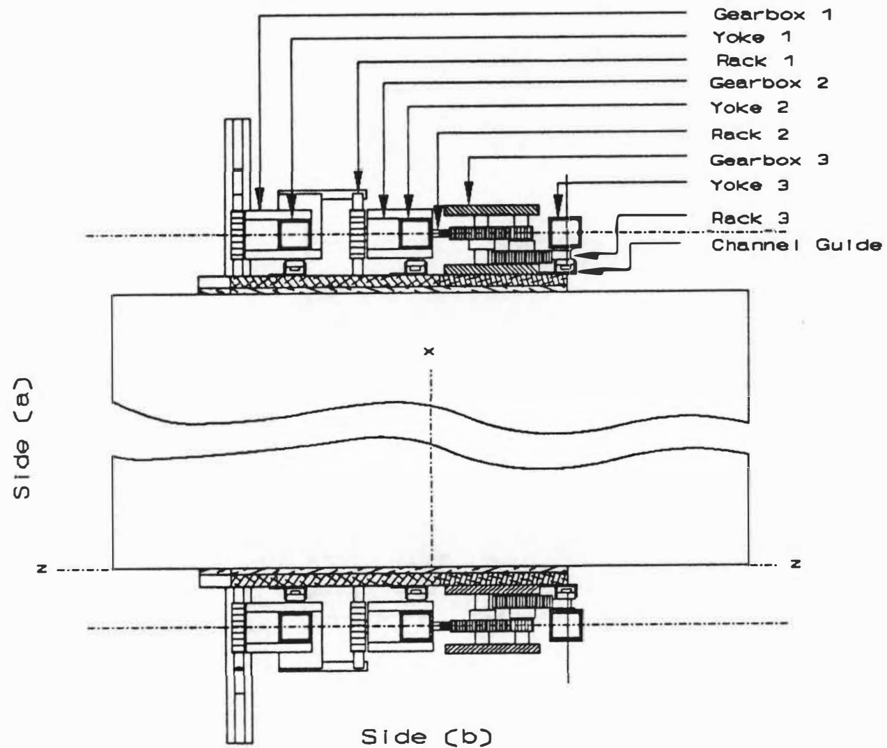
Figure 3.4 - Section A-A of the mechanical device.
