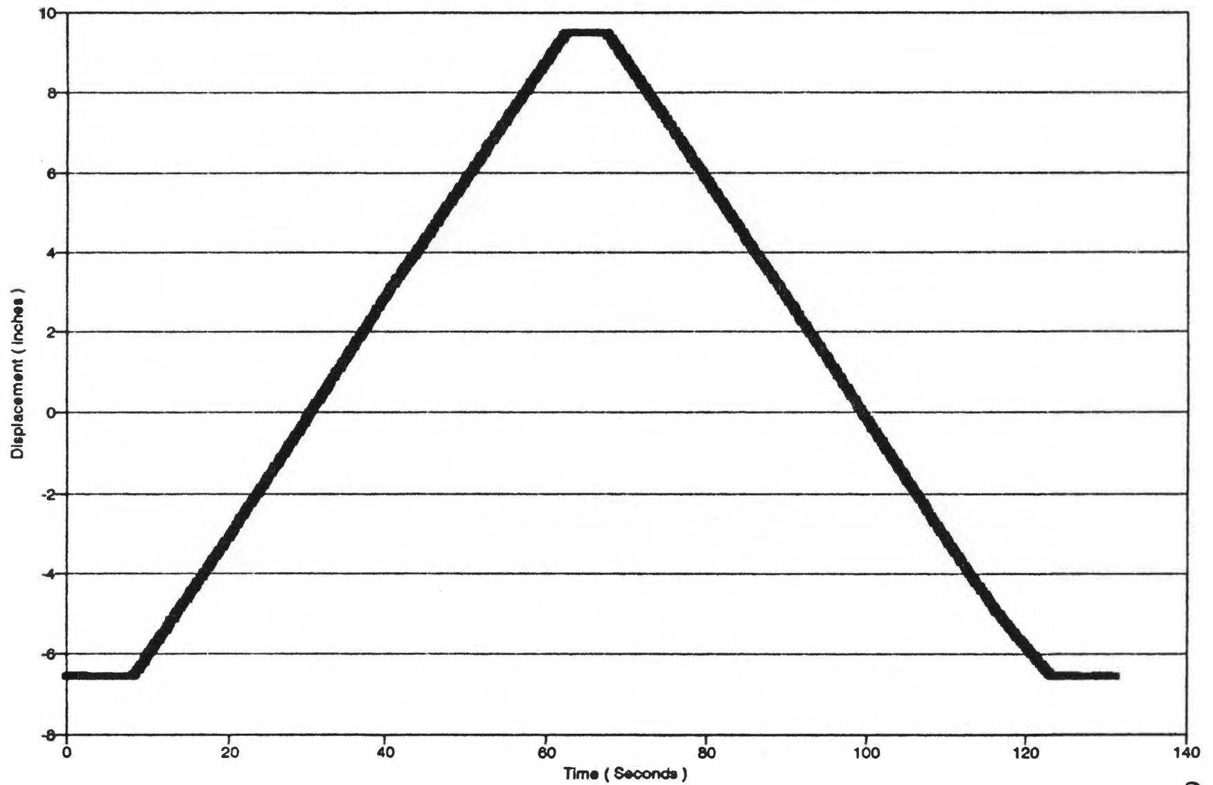
Figure 5.1 - Yoke displacement during press time.
