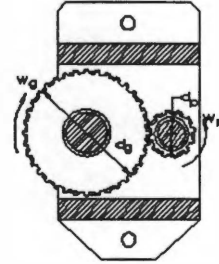
Figure 4.4 - View of the gears of the speed multiplier mechanism.
