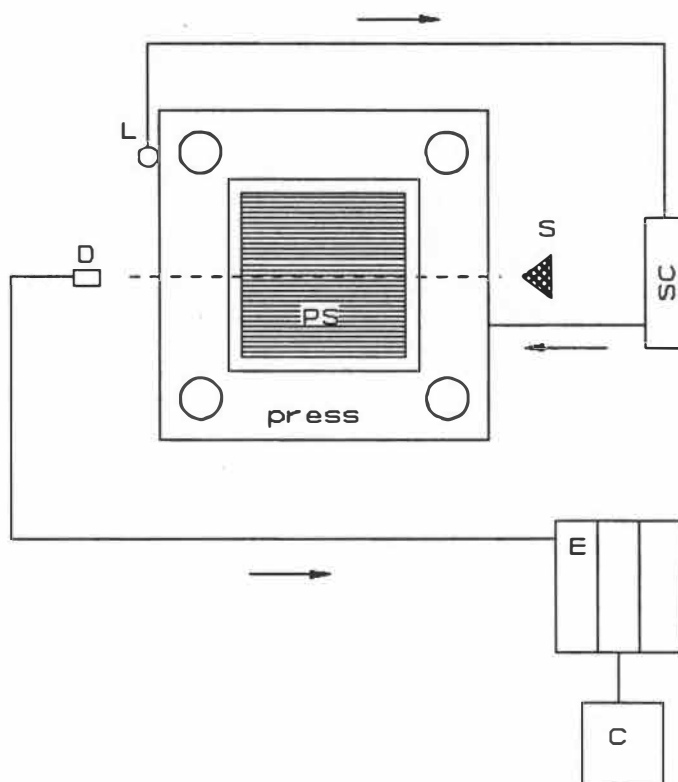
Figure 5.3 - Schematic representation of the gamma densitometer apparatus. SC) press digital servo controller; PS) sample; L) LVDT; S) source; D) photoscintillation detector; E) electronics for gamma detection; C) PC microcomputer.
