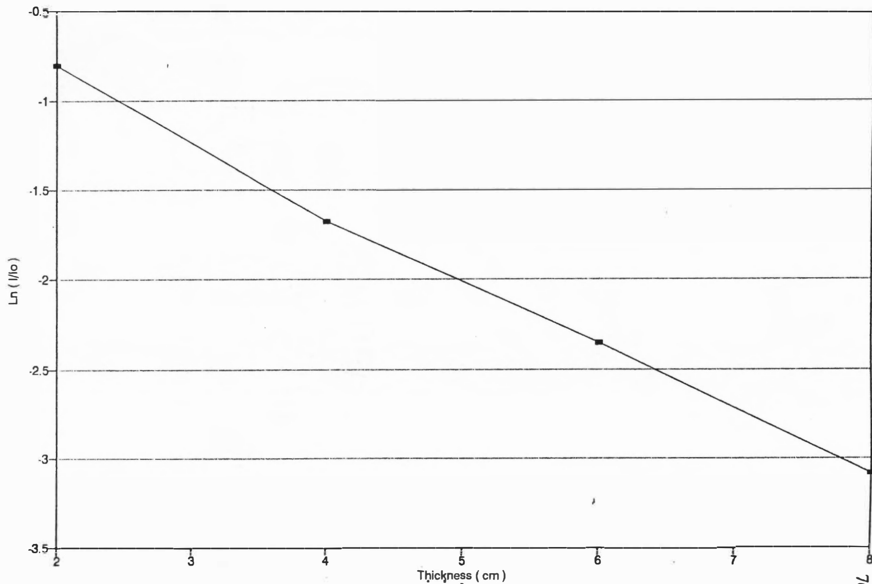
Figure 5.4 - Calibration test (four thicknesses of Oak).
