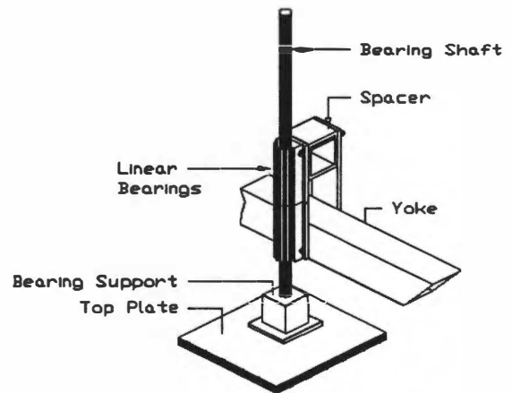
Figure 4.1 - View of the linear bearings positioning yoke at two positions symmetrically placed on top of press.
