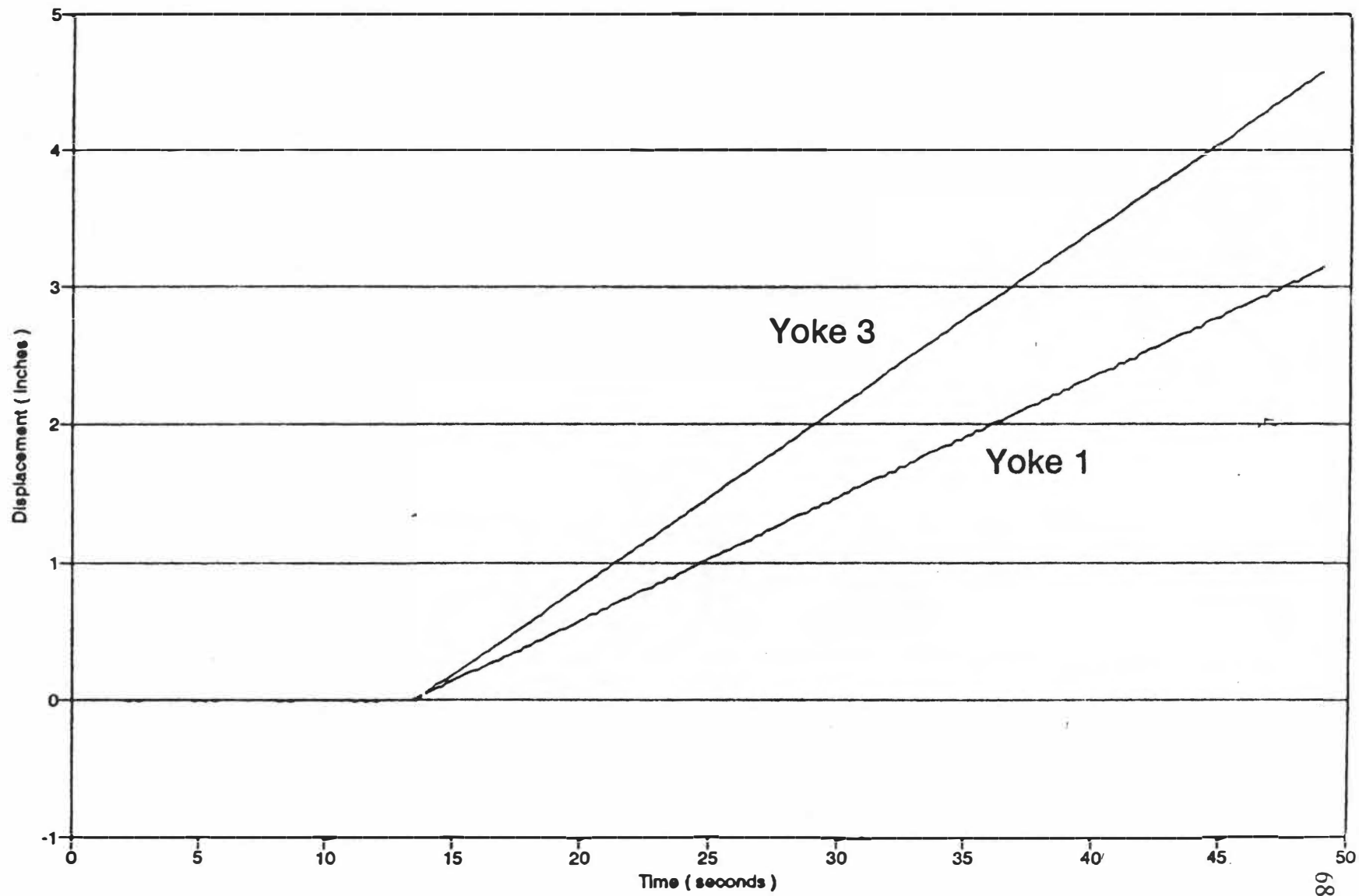
Figure 5.2 - Displacement yoke 1 and yoke 3 (press closing portion).
