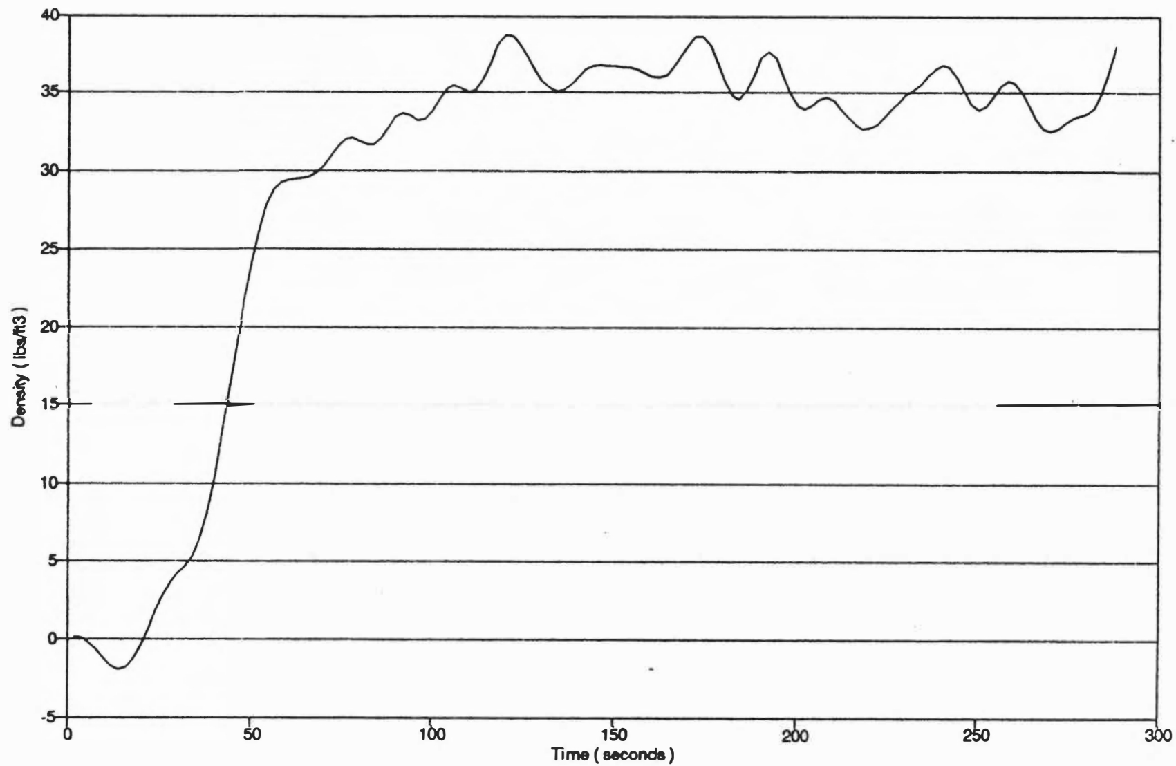
Figure 5.14 - Density during press cycle (sample:13 - width:12"), smoothed plot.
