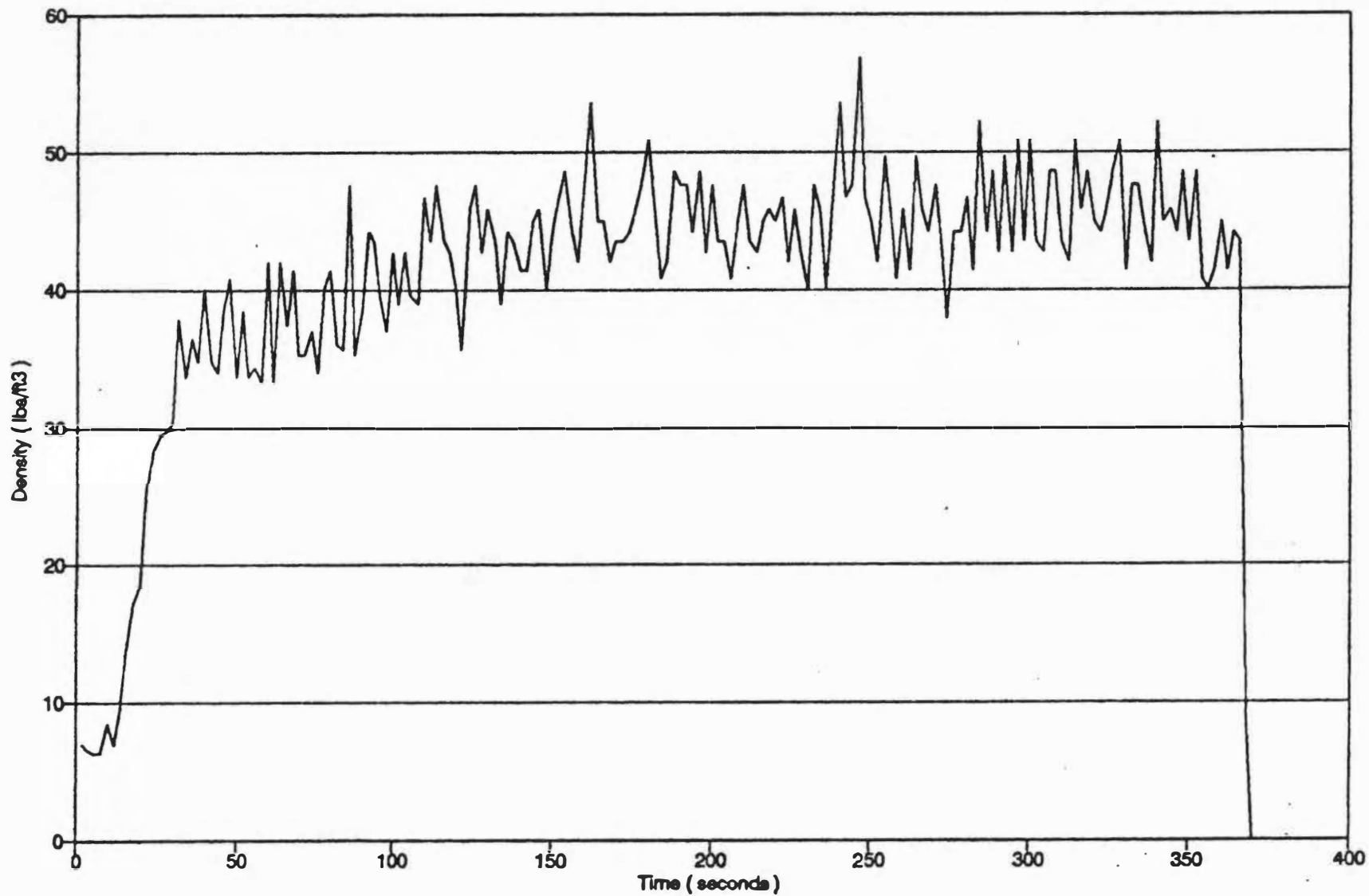
Figure 5.8 - Density during press cycle (sample:12 - width:8").
