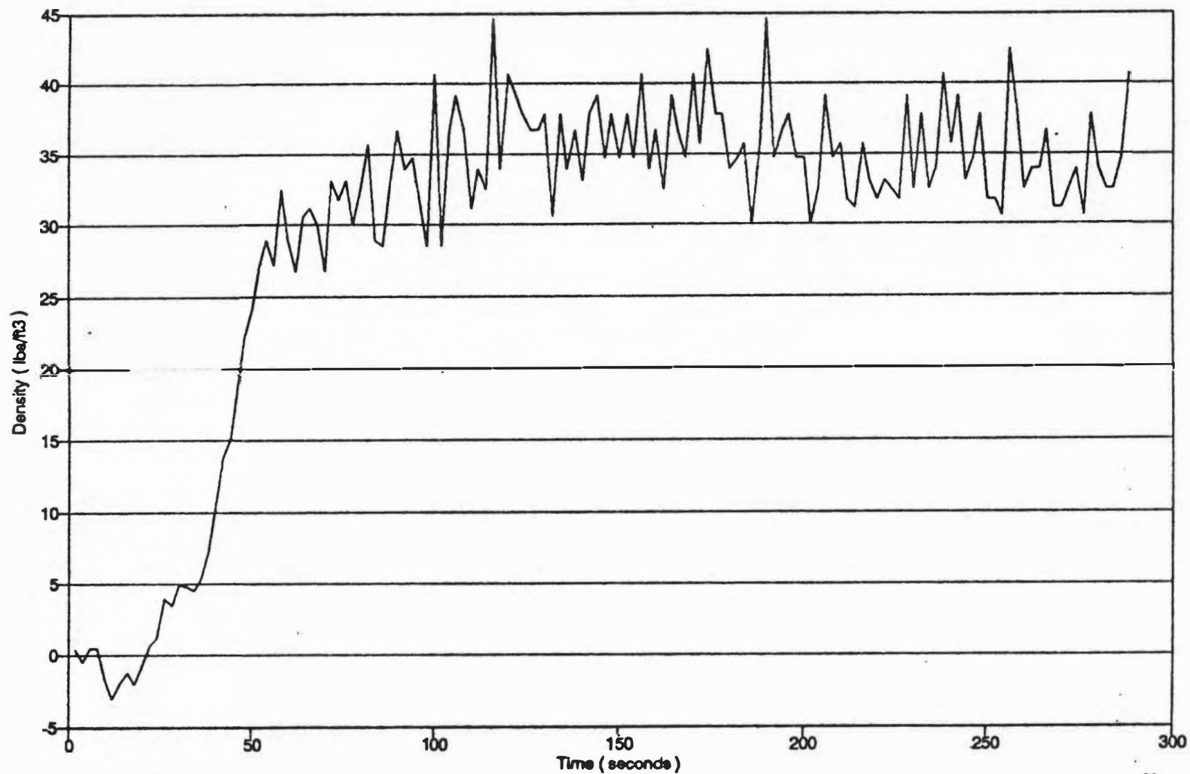
Figure 5.9 - Density during press cycle (sample:13 - width:12").
