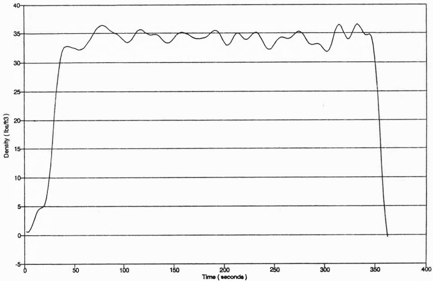
Figure 5.11 - Density during press cycle (sample:9 - width:4"), smoothed plot.
