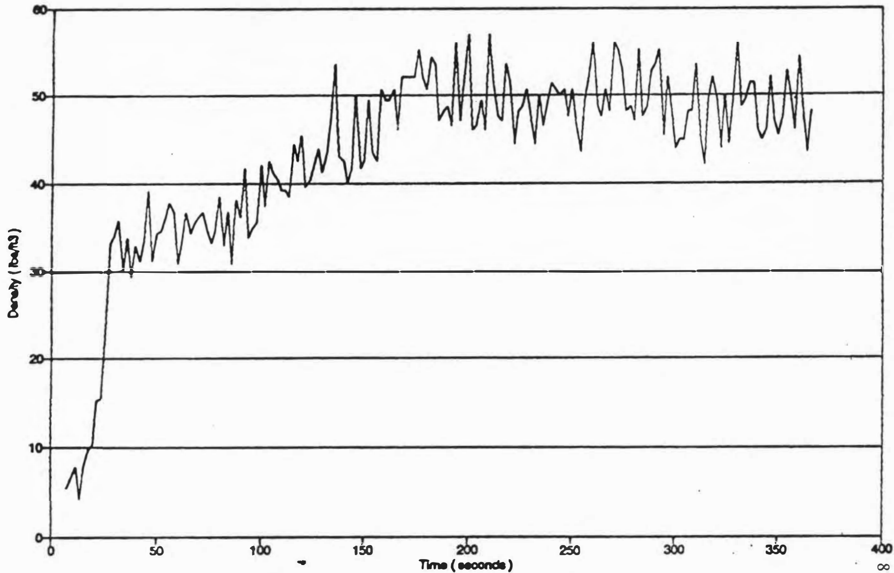
Figure 5.7 - Density during press cycle (sample:11 - width:6").
