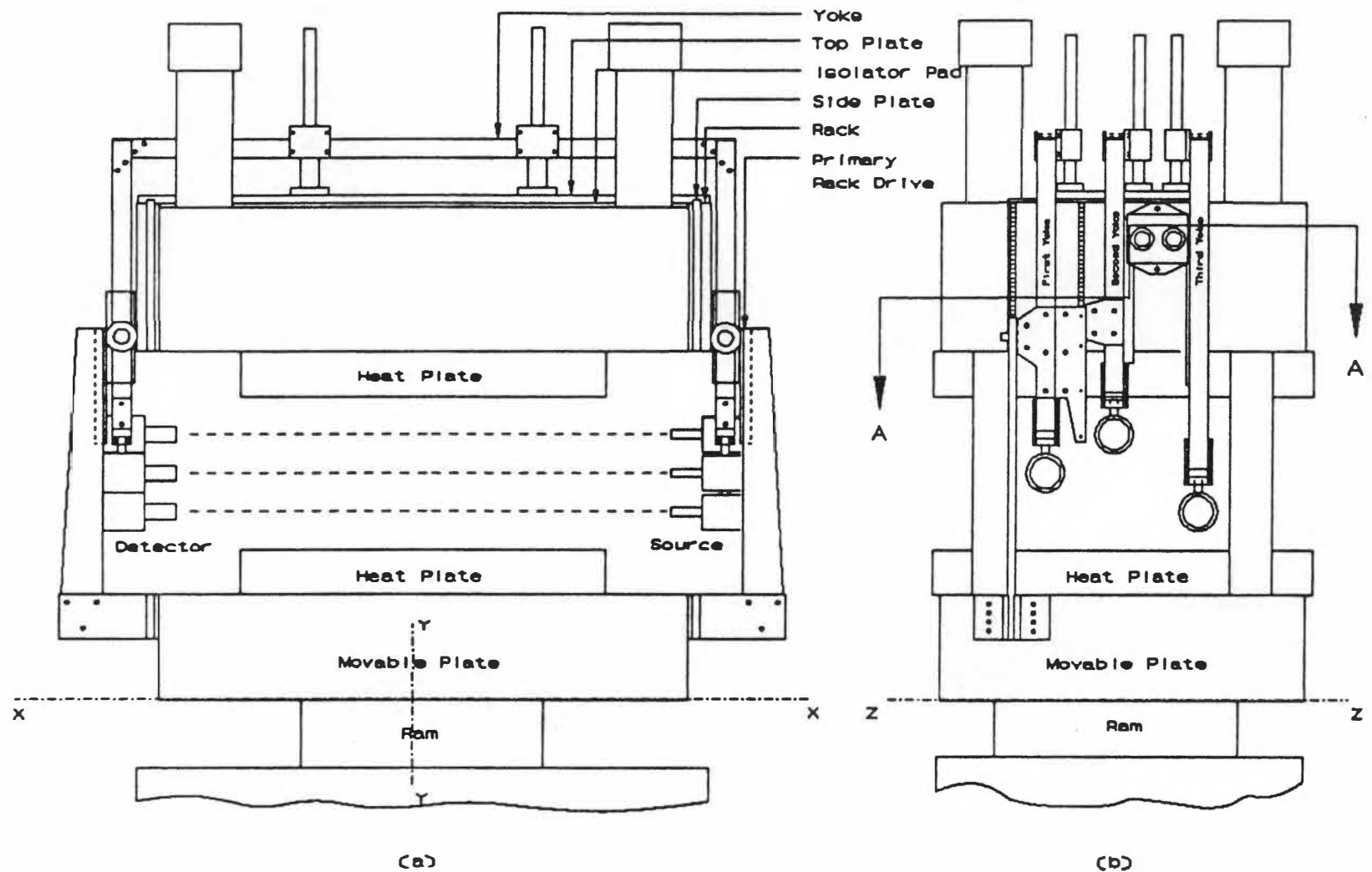
Figure 3.3 - Front View (a) and Side View (b) of yoke-translation device for translocation of sources and detectors in fixed horizontal planes relative to the mat height.
