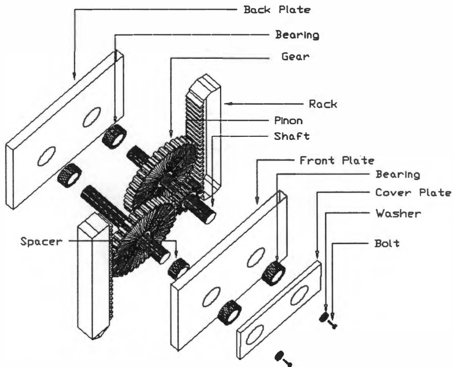
Figure 4.5 - Step-up gear, housing, shaft assembly.
