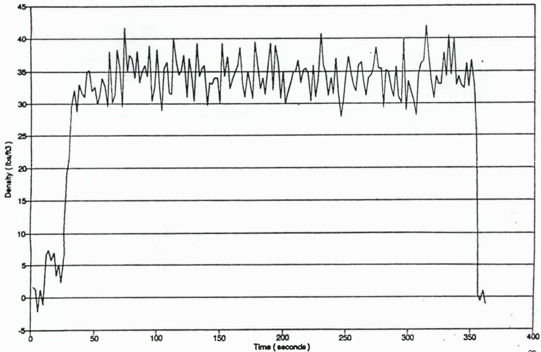
Figure 5.6 - Density during press cycle (sample:9 - width:4").
