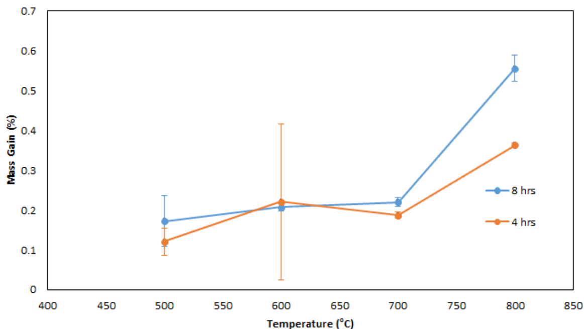
Fig. 8: The oxidation mass gain with temperature plot for SCR samples treated for both 8 and 4 hours, where the error bars represent one standard deviation.
