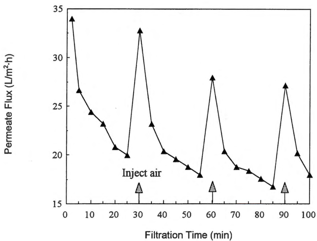
Figure 17. The effect of intermittent mixing of air bubbles into FBS1 biomass solution (37% Air, Initial C_B = 0.34 g/L, Flow Rate = 8.0 L/min).
