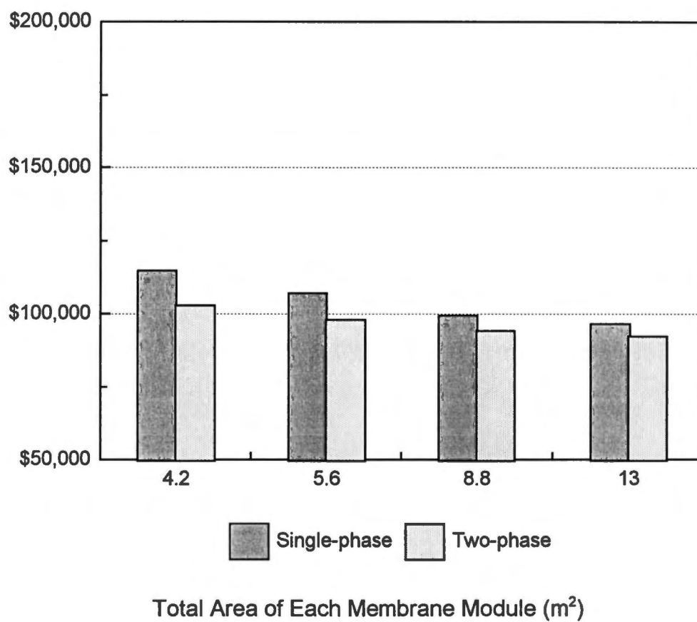
Figure 28. Annual operating costs for a scaled-up microfiltration (The capacity of cheese manufacturing plant = 189 m³/week).
