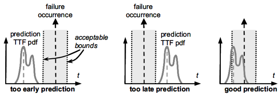
Figure 2-2 TTF predictions [68]
