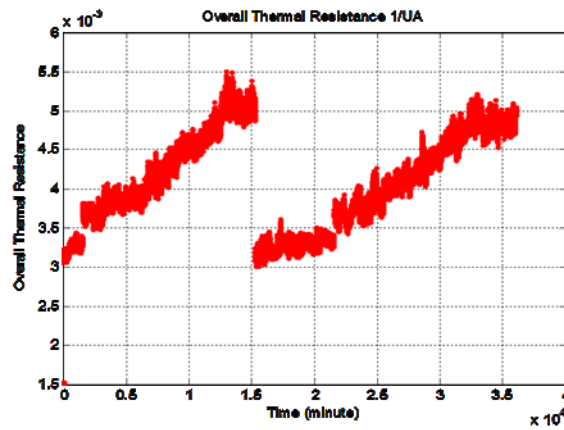
Figure 3-2 Degrdation in heat exchangers before and after cleaning
