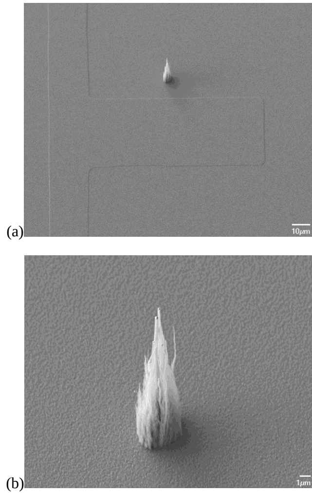
Figure 4-28. SEM images after VACNF growth test on Cr/W/SiO 2 /Si wafer structure. Prior to W film deposition, wafer contact holes were patterned
