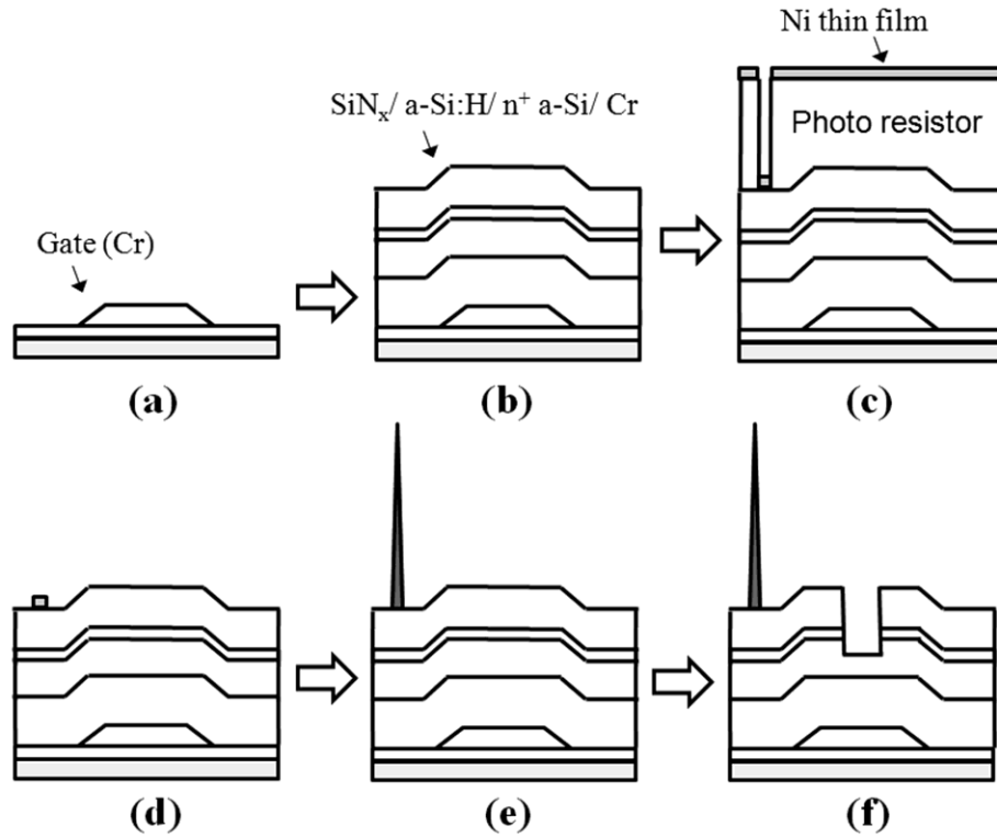
Figure 4-13. Schematic illustrating the processing sequence for the TFT-VACNF integration. (a) Cr film deposition and patterned for gate electrode, (b) \text{a-SiN}_x , \text{a-Si:H} , and \text{n}^+ \text{a-Si} deposition in situ using PECVD following Cr film for source-drain electrode deposited, (c) nickel dot patterns are formed on source-drain electrodes using conventional photo-lithography and Ni deposition by evaporation (d) the lift off process. (e) illustrates the VACNF growth on the nickel catalyst on the uniform chromium layer which is (f) subsequently patterned followed by the active layer back-channel etch process
