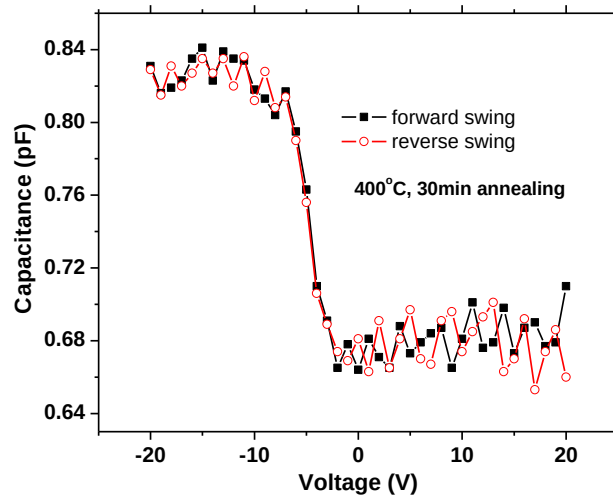
Figure 2-14. C-V characteristics of Low stress \text{SiN}_x layer (a) as-deposited, and (b) annealed at 400°C during 30min.
