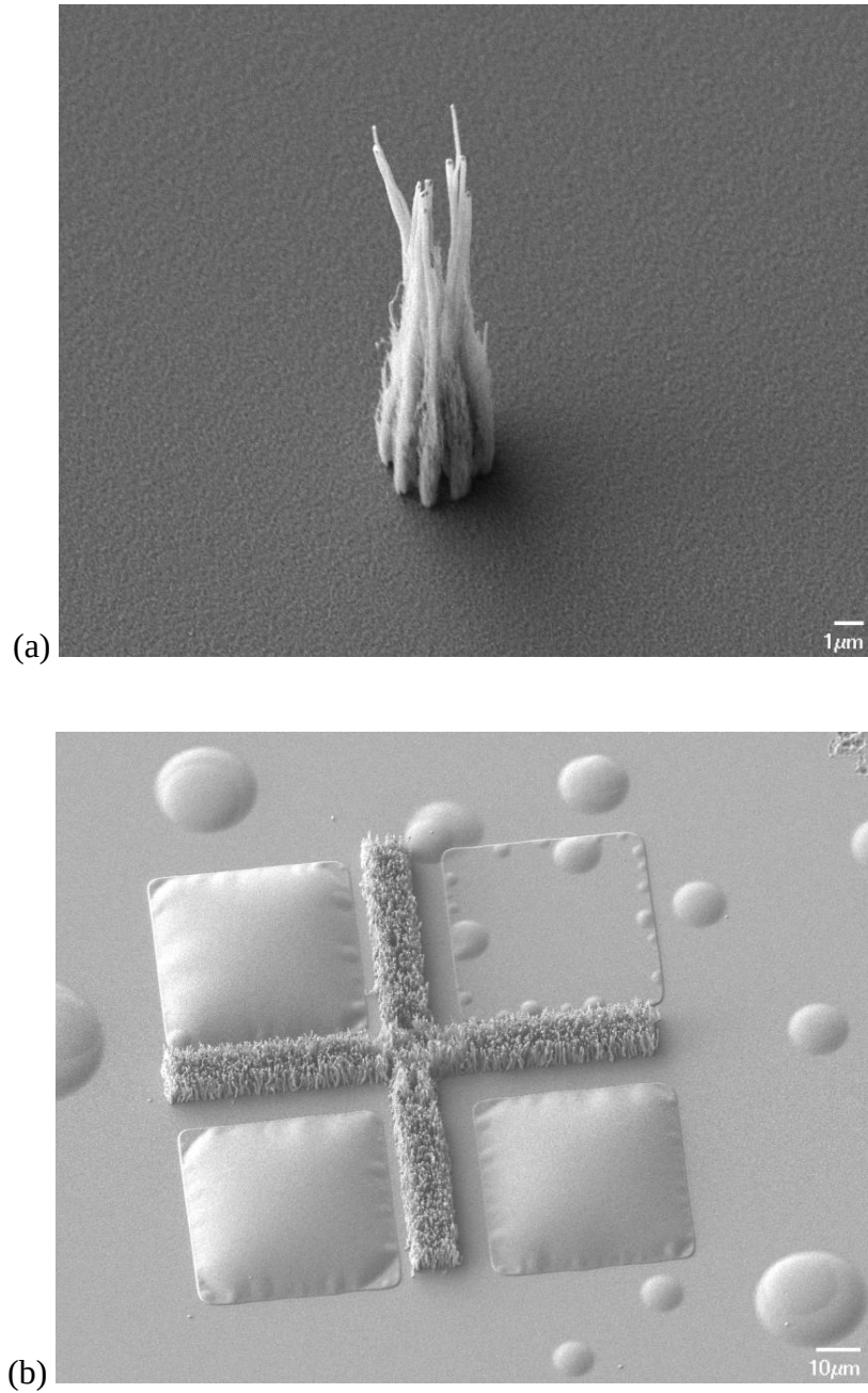
Figure 4-6. a)SEM image of showing an \sim 20 microns tall VACNF successfully grown using the through via patterns, and b)SEM image showing bubbles which lift the chromium source and drain electrode for VACNF growth on the region near the alignment marks
