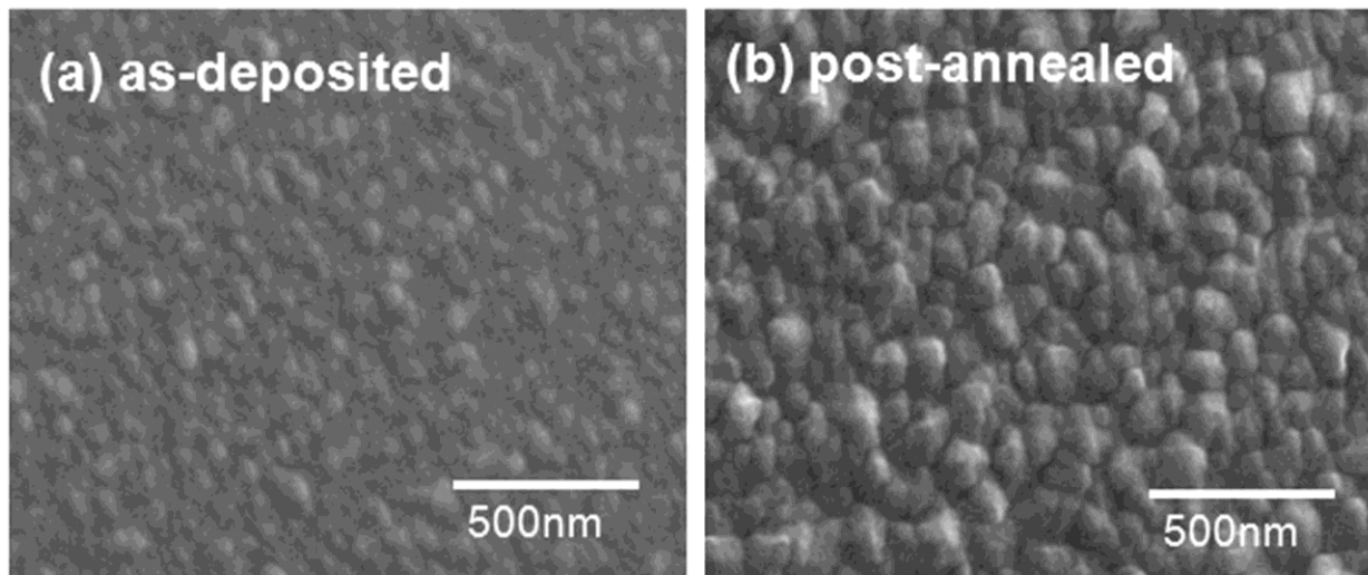
Figure 2-19. SEM images of (a) as-deposited poly-Si (625°C, LPCVD), and (b) post-annealed (800°C, 30min soak) poly-Si
