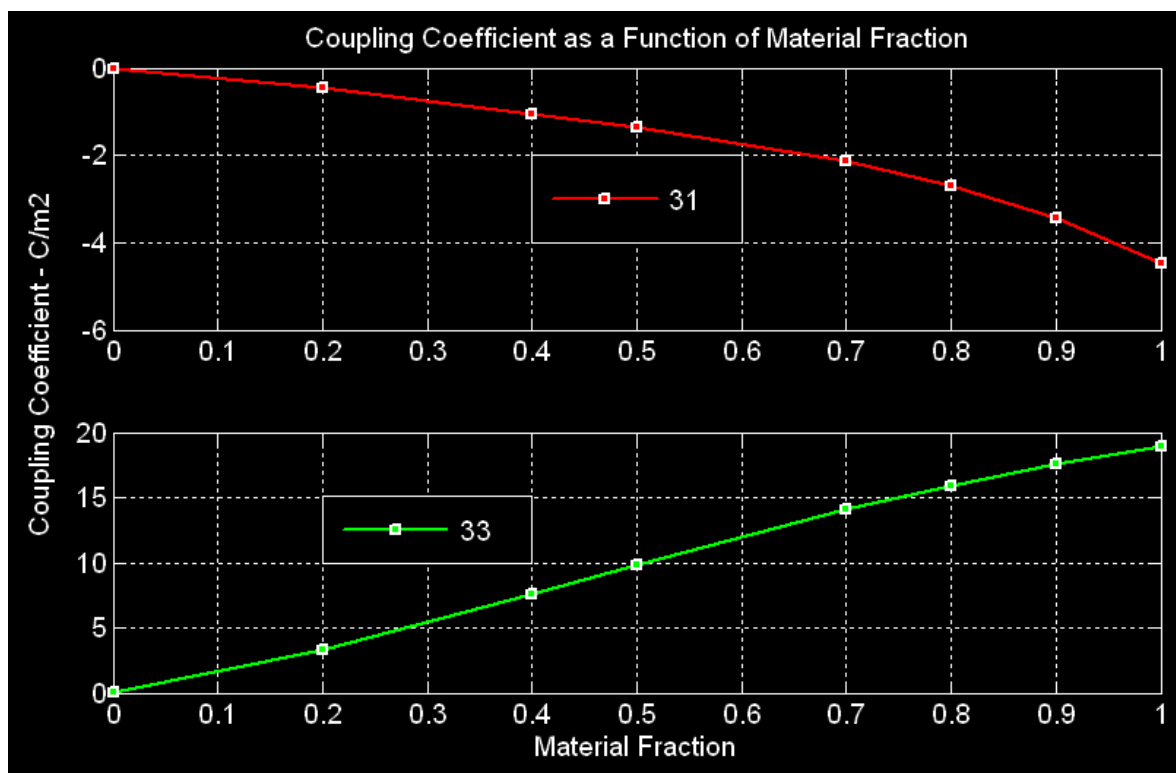
Figure 3.10: Variation of Coupling Coefficients w.r.t. Material Fraction
