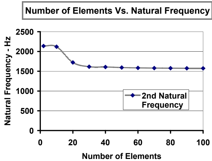
Figure 4.3: Convergence study for the 2nd Natural Frequency Vs.
