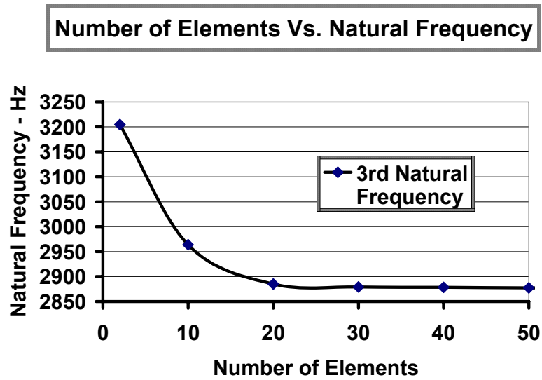
Figure 4.4: Convergence study for the 3rd Natural Frequency Vs.
