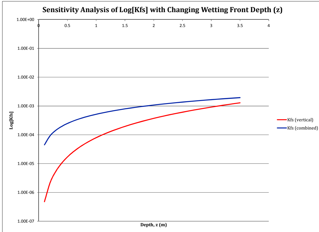
Figure A4: Sensitivity analysis graph of Log [ K_{fs} ] with changing wetting front depth (z) for the Schwartzman and Zur (1987) vertical and combined equations. The range in changing depth values and constant values of width, volume, and outflow discharge rates are detailed in Table A2.
