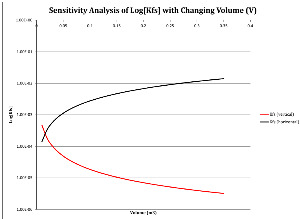
Figure A6: Sensitivity analysis graph of \text{Log}[K_{fs}] with changing cumulative infiltration volume (V) for the Schwartzman and Zur (1987) vertical and horizontal equations.
