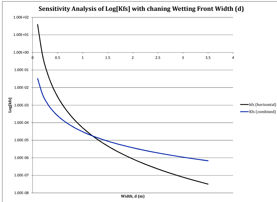
Figure A2: Sensitivity analysis graph of Log [K_{fs}] with changing wetting front width (d) for Schwartzman and Zur (1987) horizontal and combined equations. The range in changing width values and constant values of depth, volume, and outflow discharge rates are detailed in Table A1.
