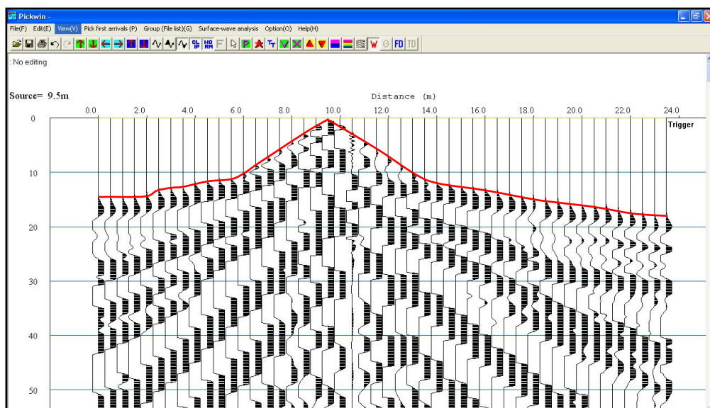
Figure 9: Seismic record example containing first-arrival picks (in red) on a single shot-point using SeisImager Pickwin95 TM software
