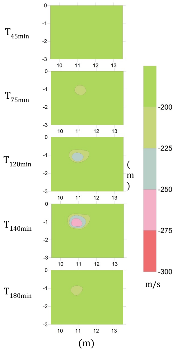
Figure 24: Discrete P -wave velocity profiles centered on the area of infiltration for the first constant flux applicator experiment with the velocity interval constrained to be from -300 m/s to -200 m/s and a contour interval of 25 m/s. A trend analysis has been applied to each of the profiles.
