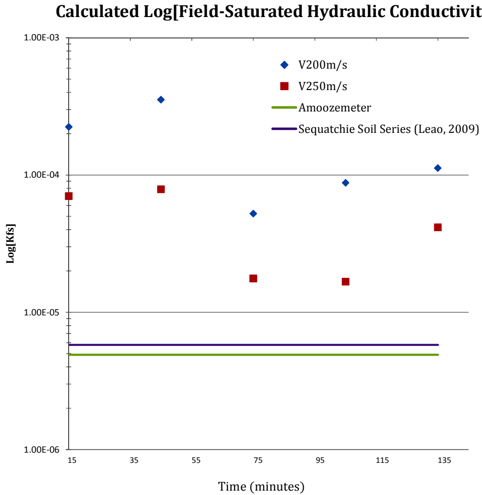
Figure 37: Log [Kfs] plotted versus time from the Sequatchie series, Amoozemeter method, and the TLSFT infiltration method where dimensions are measured from 250 m/s and 200 m/s velocity
