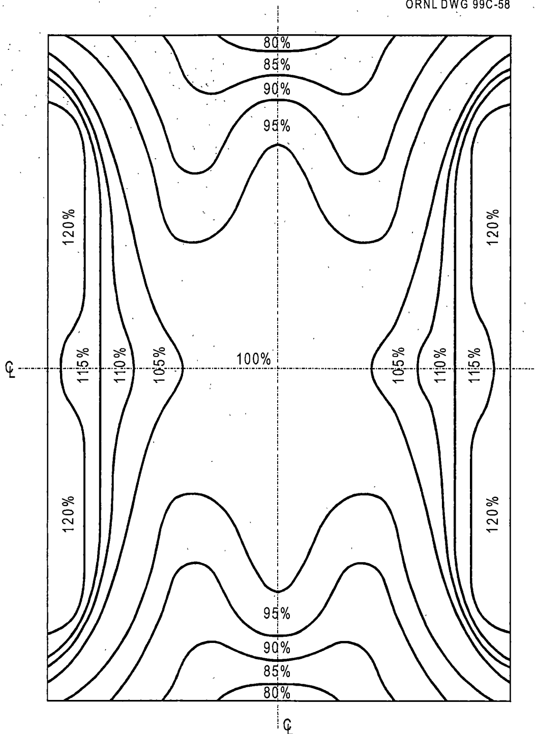
Fig. 3.3. Exposure rate profile for ORNL ^{60}\text{Co} irradiation chamber. (Reported 100% exposure rate on December 9, 1977, was 1.85 \times 10^6 R/h) (after Shepherd 1977).
