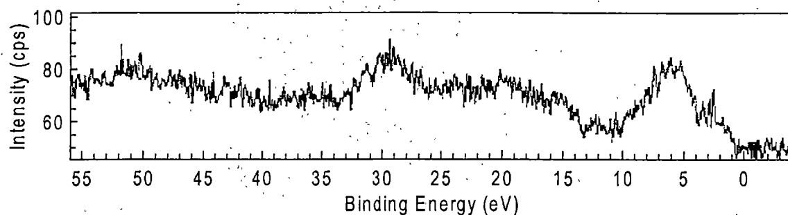
Fig. 4.10. XPS valence spectrum for sample S-1.
