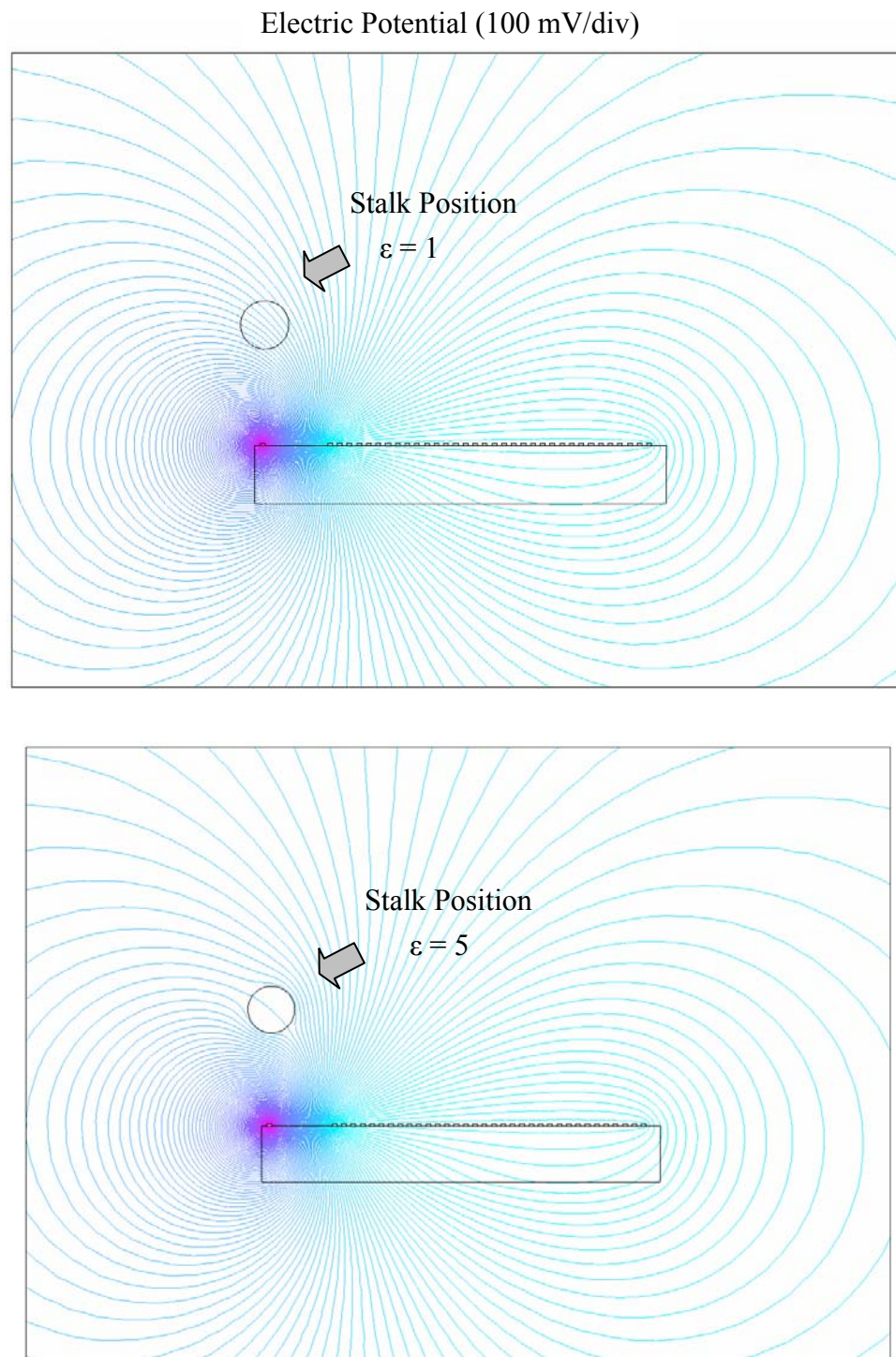
Figure 26. Semi-interdigital sensor pattern electrical potential lines with and without a stalk
