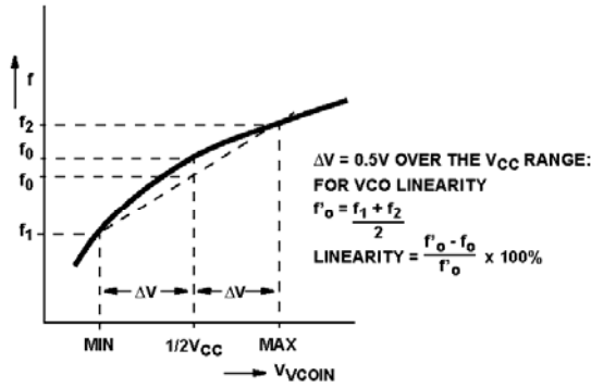
FIGURE 33. DEFINITION OF VCO FREQUENCY LINEARITY
