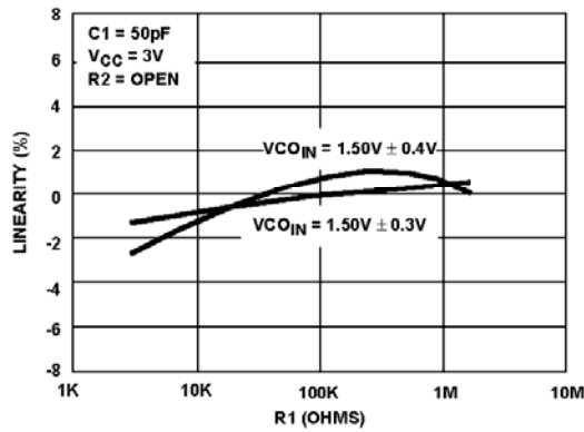
FIGURE 35. HC4046A VCO LINEARITY vs R1 ( V_{CC} = 3V )
