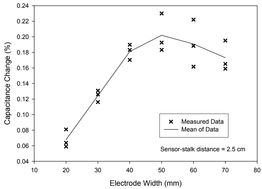
Figure 30. Modeled and measured change for different ground electrode widths
