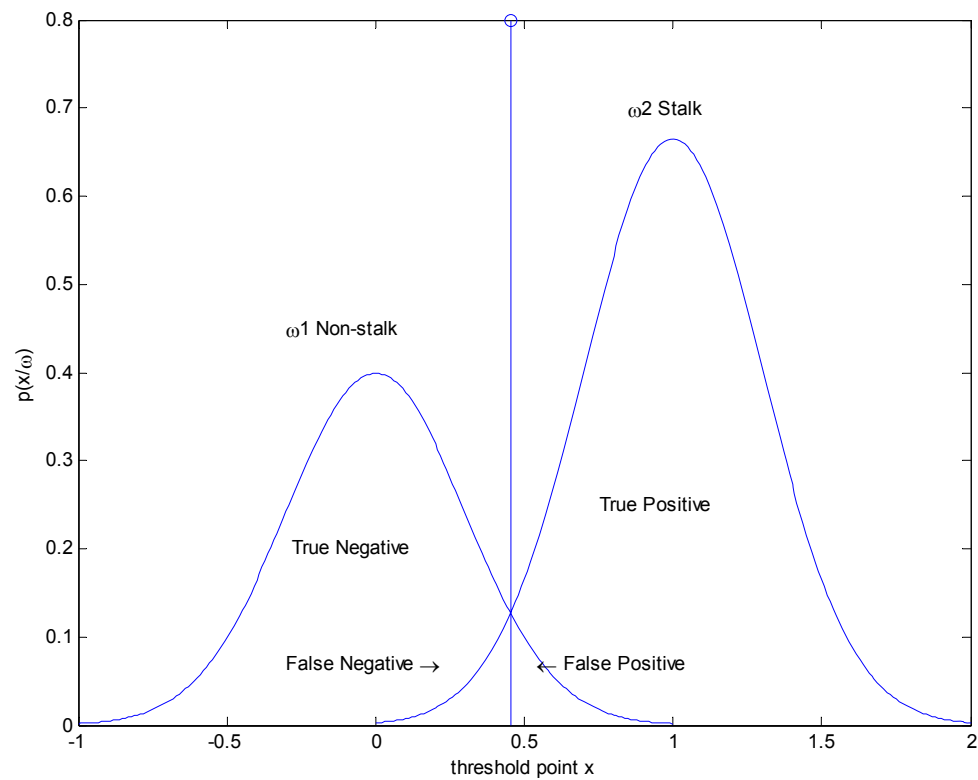
Figure 90. Illustration of classification into two categories
