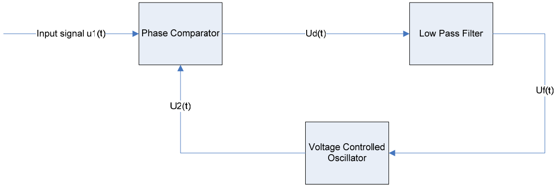
Figure 43. Phase-locked loop functional schematic
