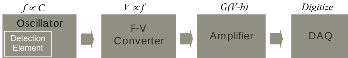
Figure 33. Functional diagram of sensor circuitry and data acquisition system
