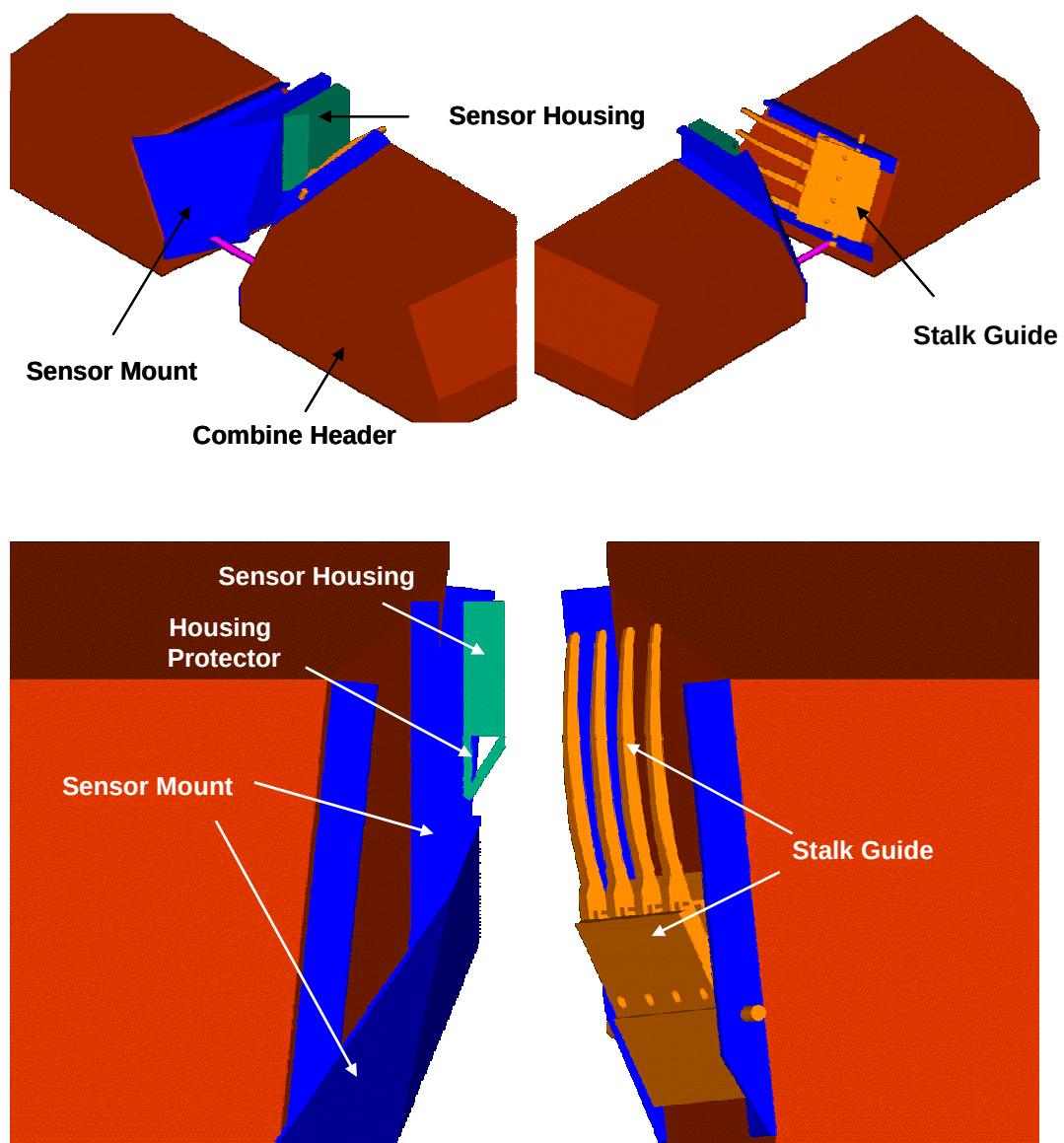
Figure 56. Sensor mounting fixture.
