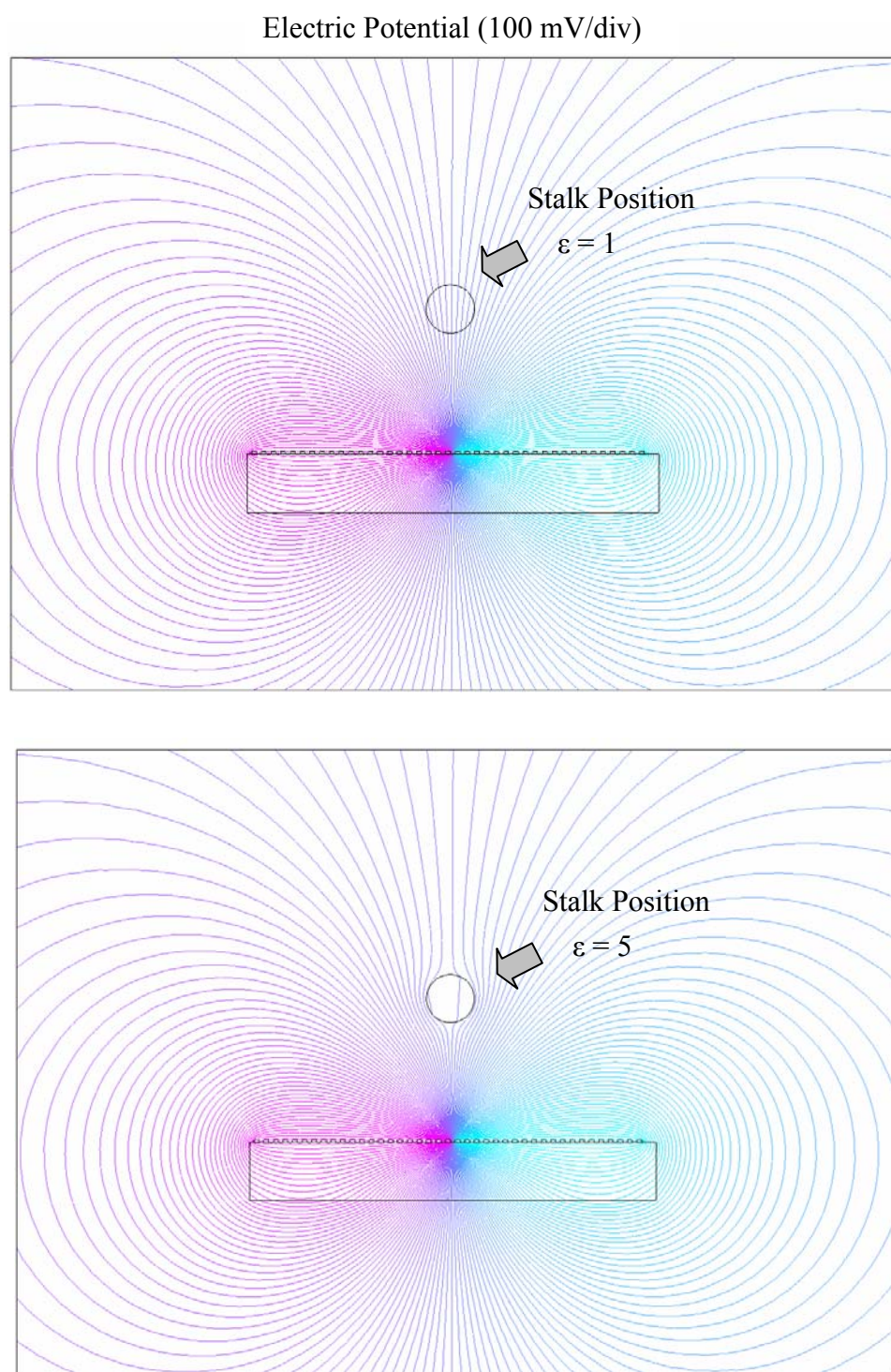
Figure 22. Polarized interdigital model electrical potential lines
