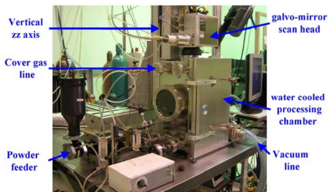
Figure 3 – The prototype tower nozzle SFF system.
