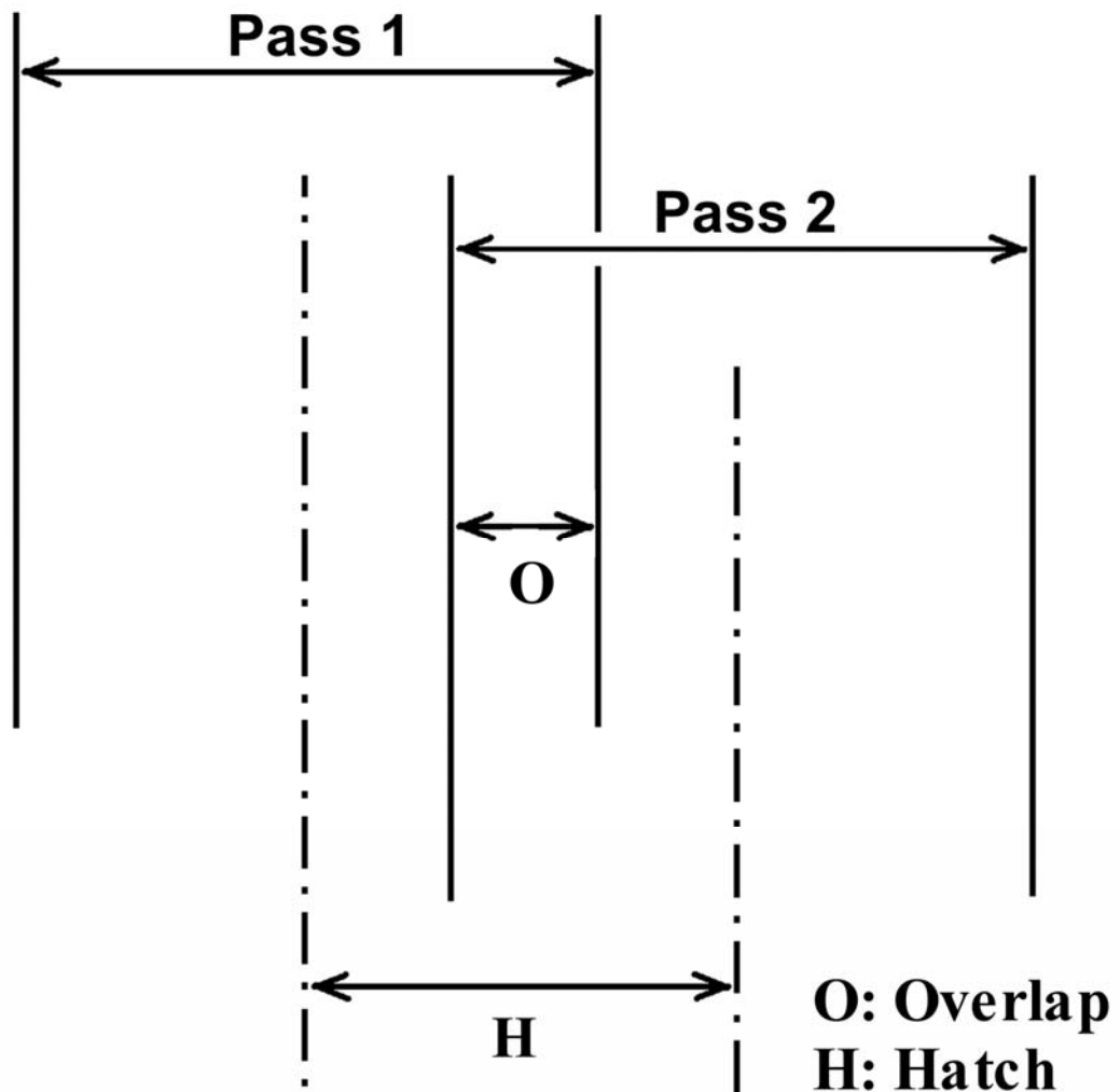
Figure 3.3. The “hatch” is defined as the distance between the centerlines of laser beam in subsequent passes as shown in this sketch.
