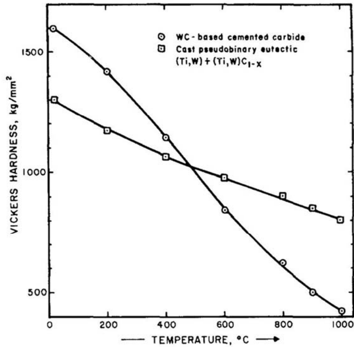
Figure 12 – Vickers hardness as a function of temperature for commercial WC cemented carbide material and cast eutectic (W,Ti) – (Ti,W)C cermelt. Source: [16].
