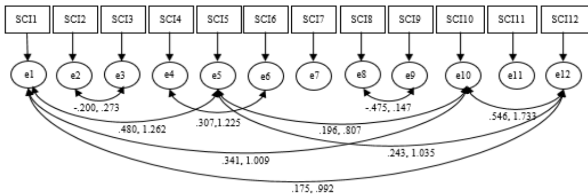
Figure 7. Bootstrap bias corrected 95% CIs for the urban model error covariances.
