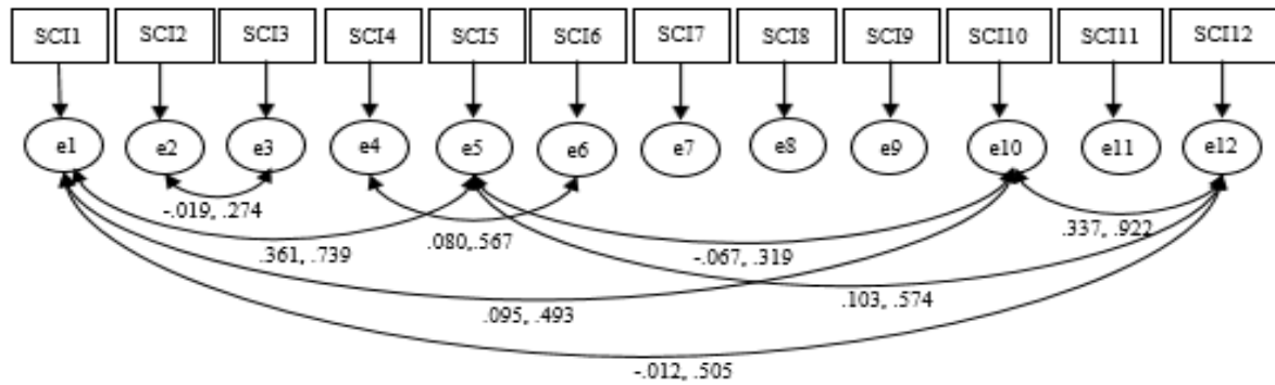
Figure 6. Bootstrap bias corrected 95% CIs for the suburban model error covariances.
