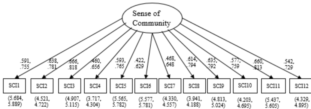
Figure 4. Bootstrap bias corrected 95% CIs for the standardized factor loadings and intercepts for the urban one factor model with correlated error variances.
