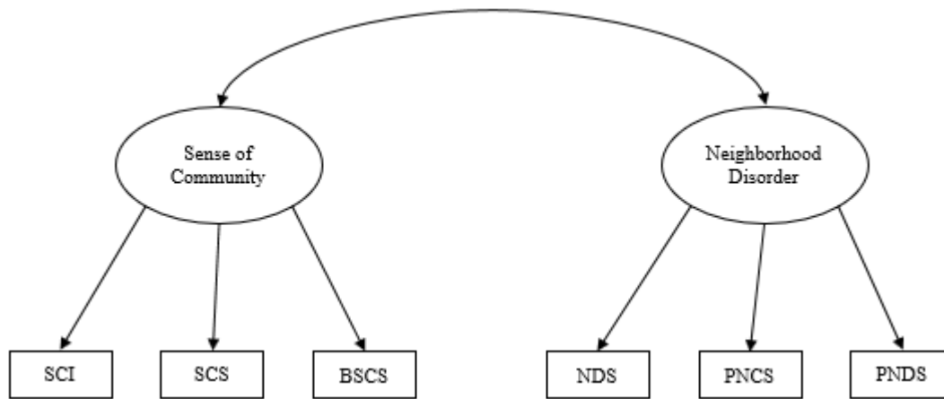
Figure 8. Simple Confirmatory Factor Analysis testing convergent and divergent validity of the SCI
