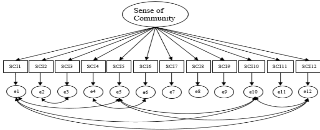
Figure 1. Single factor model of Sense of Community Index with correlated error covariances.
