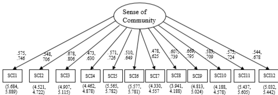
Figure 2. Bootstrap bias corrected 95% CIs for the standardized factor loadings and intercepts for the rural one factor model with correlated error variances.
