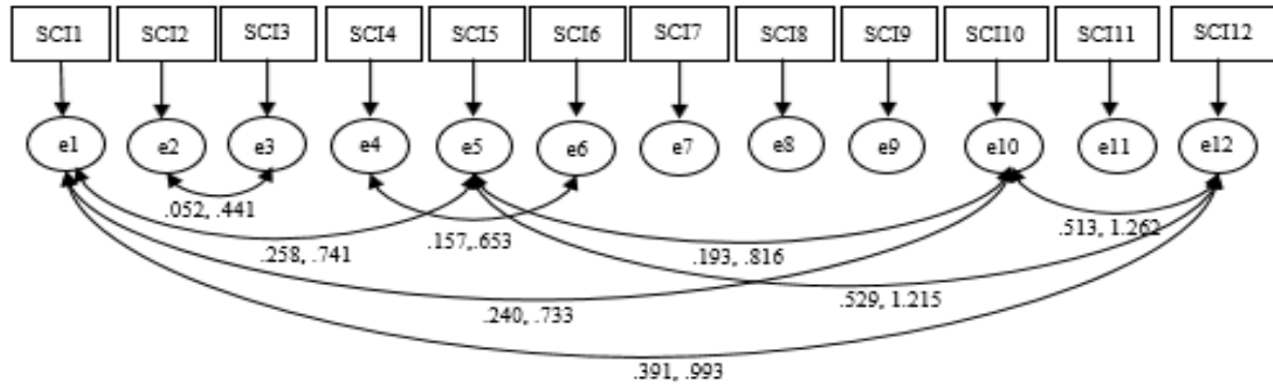
Figure 5. Bootstrap bias corrected 95% CIs for the rural model error covariances.
