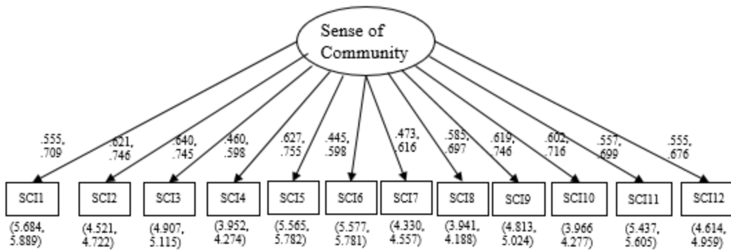
Figure 3. Bootstrap bias corrected 95% CIs for the standardized factor loadings and intercepts for the suburban one factor model with correlated error variances.
