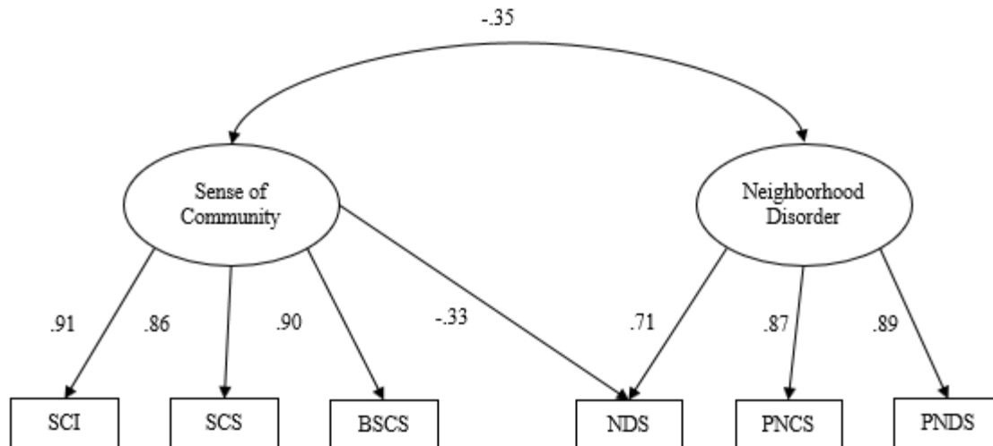
Figure 10. Standardized factor loadings of simple Confirmatory Factor Analysis to test convergent and divergent validity of the SCI.
