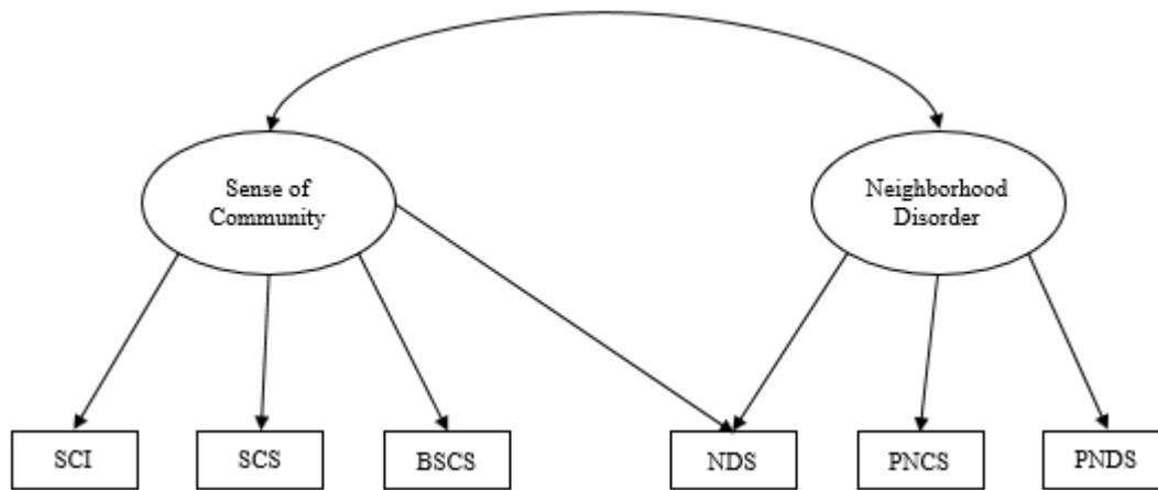
Figure 9. Simple Confirmatory Factor Analysis to test convergent and divergent validity of the SCI with added path between the sense of community latent construct and the NDS.
