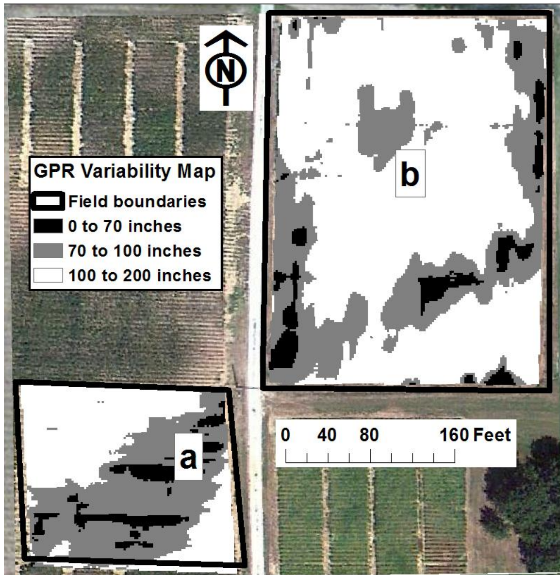
Figure 3: Depth to sand variability indicated by GPR data
