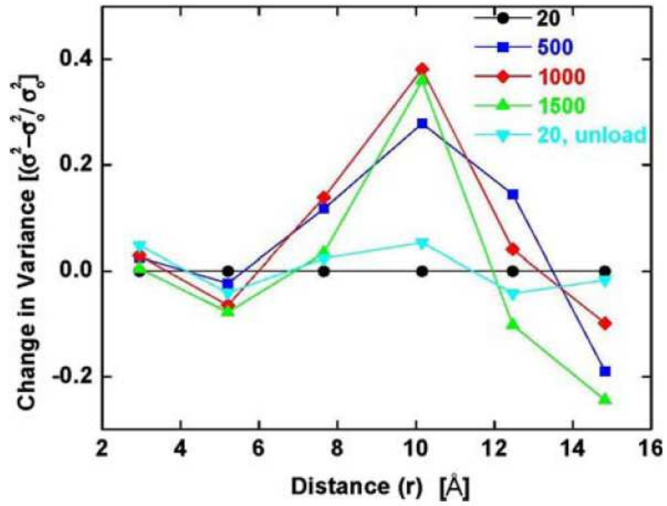
Figure 4-30. Change in variance from the center of mass measurements as a function of distance r measured on \text{Zr}_{57}\text{Nb}_5\text{Cu}_{15.4}\text{Ni}_{12.6}\text{Al}_{10} bulk metallic glass.
