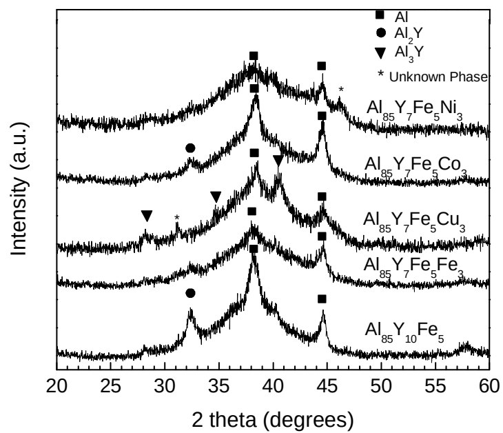
Figure 4-1. X-ray diffraction patterns of ball-milled Al 85 Y 10 Fe 5 and Al 85 Y 7 Fe 5 TM 3 (TM = Ni, Co, Cu, and Fe).
