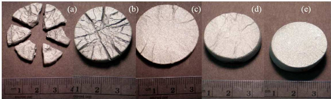
Figure 4-23. Photographs of consolidated Al 79 Y 7 Fe 8 Ni 3 Ti 2 Nd 1 samples after forging: (a) 100% MA alloy forged at 420°C, (b) 85% MA + 15% CG alloy forged at 420°C, (c) 70% MA + 30% CG alloy forged at 420°C, (d) 100% MA alloy forged at 445°C, and (e) 70% MA + 30% CG alloy forged at 445°C. (scale in centimeters)
