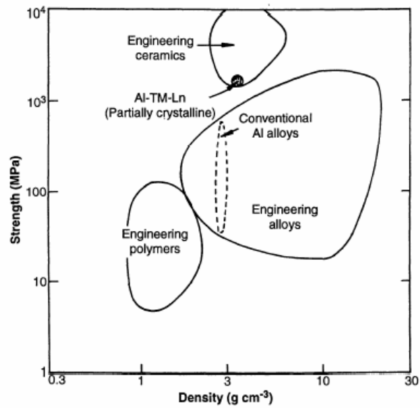
Figure 1-1. Schematic showing the strength-density relationship for various engineering materials [44].
