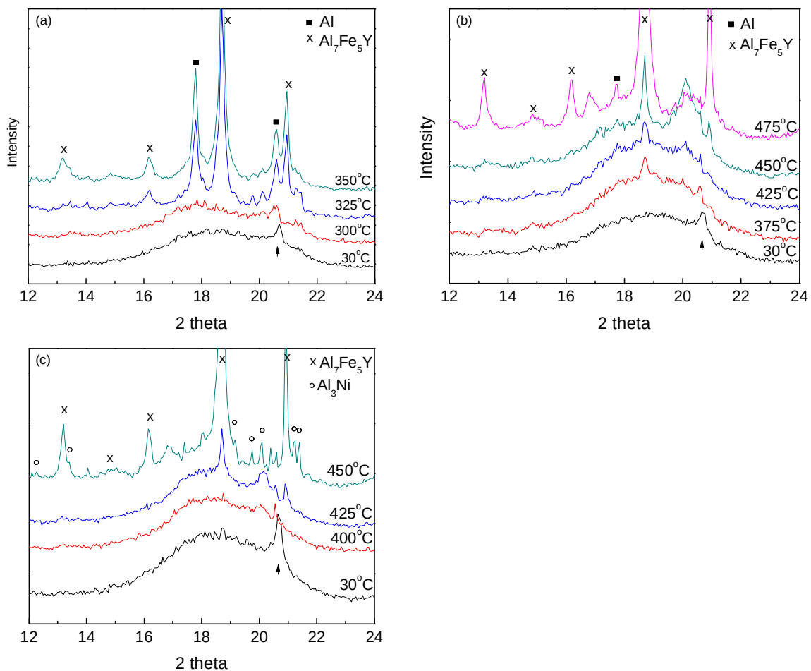
Figure 4-22. Selected in-situ synchrotron XRD patterns for (a) \text{Al}_{85}\text{Y}_7\text{Fe}_8 at 30°C, 300°C, 325°C, and 350°C; (b) \text{Al}_{83}\text{Y}_7\text{Fe}_8\text{Ti}_2 at 30°C, 375°C, 425°C, 450°C, and 475°C; and (c) \text{Al}_{79}\text{Y}_7\text{Fe}_8\text{Ni}_3\text{Ti}_2\text{Nd}_1 at 30°C, 400°C, 425°C, and 450°C. An Fe phase (marked with an arrow) is present in all of the as-milled alloys.
