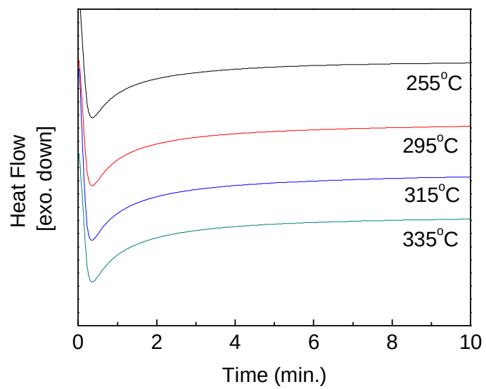
Figure 4-13. Isothermal DSC traces of \text{Al}_{85}\text{Y}_7\text{Fe}_8 performed at different temperatures.
