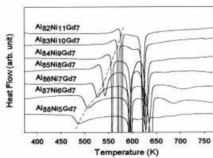
Figure 2-28. DSC curves of \text{Al}_{93-x}\text{Ni}_x\text{Gd}_7 amorphous alloys. The dashed line corresponds to the primary crystallization [24].
