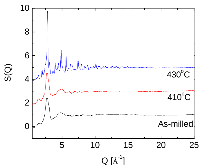
Figure 4-16. Structure factor data of \text{Al}_{83}\text{Y}_7\text{Fe}_8\text{Ti}_2 as-milled and annealed at 410^\circ\text{C} and 430^\circ\text{C} .
