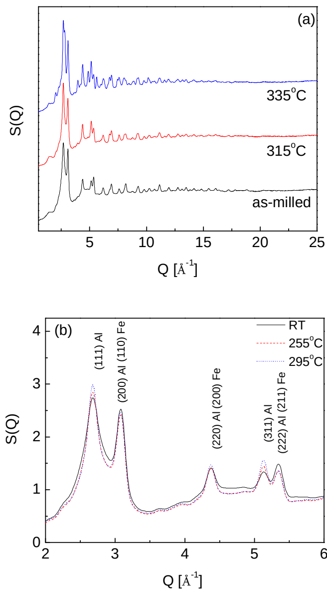
Figure 4-15. (a) Structure factor data of \text{Al}_{85}\text{Y}_7\text{Fe}_8 as-milled and annealed at 315°C and 335°C and (b) in the region of 2 – 6 \text{\AA}^{-1} in the as-milled condition and annealed at 255°C and 295°C.
