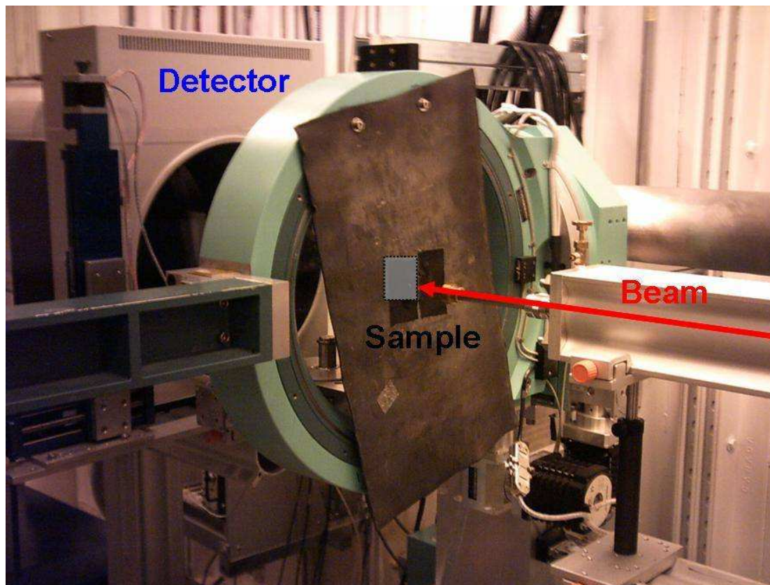
Figure 3-1. 6-ID-C synchrotron x-ray beamline at the Advanced Photon Source showing the direction of the x-ray beam, the sample location, and the detector.
