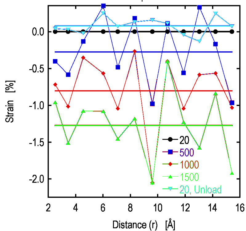
Figure 4-28a. Intercept strain data calculated from G(r) as a function distance, r for \text{Zr}_{57}\text{Nb}_5\text{Cu}_{15.4}\text{Ni}_{12.6}\text{Al}_{10} .
