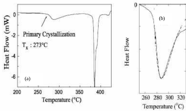
Figure 2-27. (a) DSC curve for \text{Al}_{88}\text{Y}_7\text{Fe}_5 melt-spun ribbon sample. The primary crystallization occurs at 273^\circ\text{C} and corresponds to the formation of fcc nanocrystalline aluminum phase. (b) Close-up view of the primary crystallization [102].
