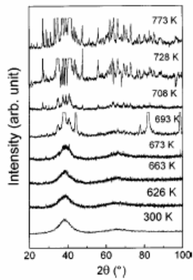
Figure 2-8. X-ray diffraction pattern of \text{Zr}_{41}\text{Ti}_{14}\text{Cu}_{12.5}\text{Be}_{22.5} BMG after annealing at different temperatures [70].
