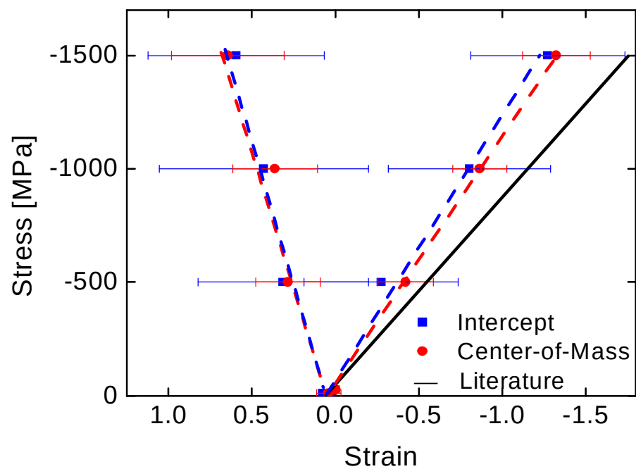
Figure 4-29. Stress vs. strain curve for \text{Zr}_{57}\text{Nb}_5\text{Cu}_{15.4}\text{Ni}_{12.6}\text{Al}_{10} calculated on SMARTS from average local strains in G (r) by the intercept method and the center of mass method.
