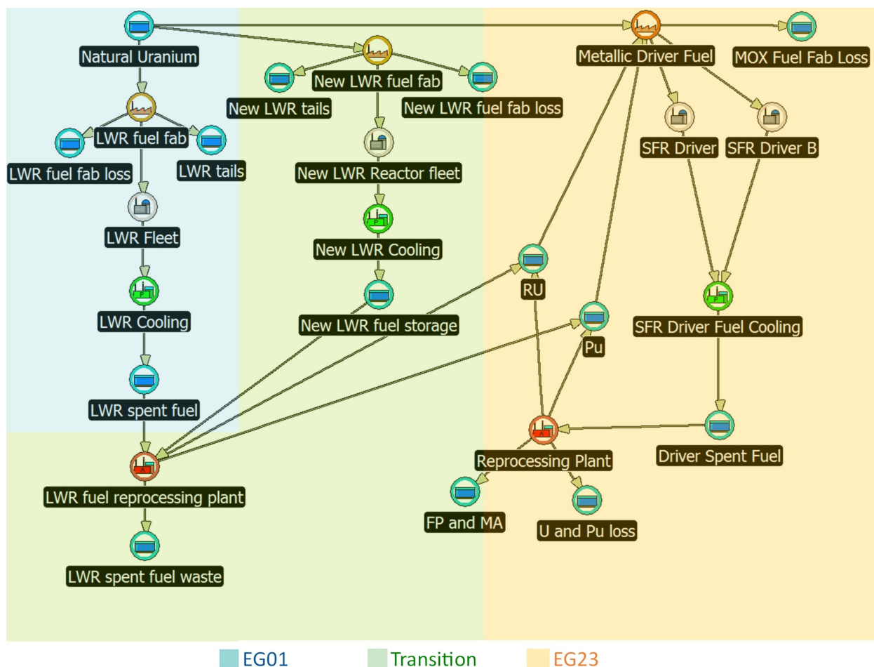
Figure 3.16: Illustration of mass flows through the EG01-EG23 transition scenario in ORION
