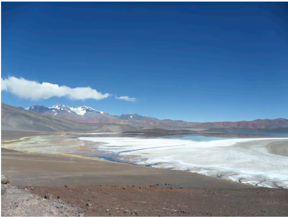
Figure 18: The southern margin of Laguna Negra where microbialites are found.
