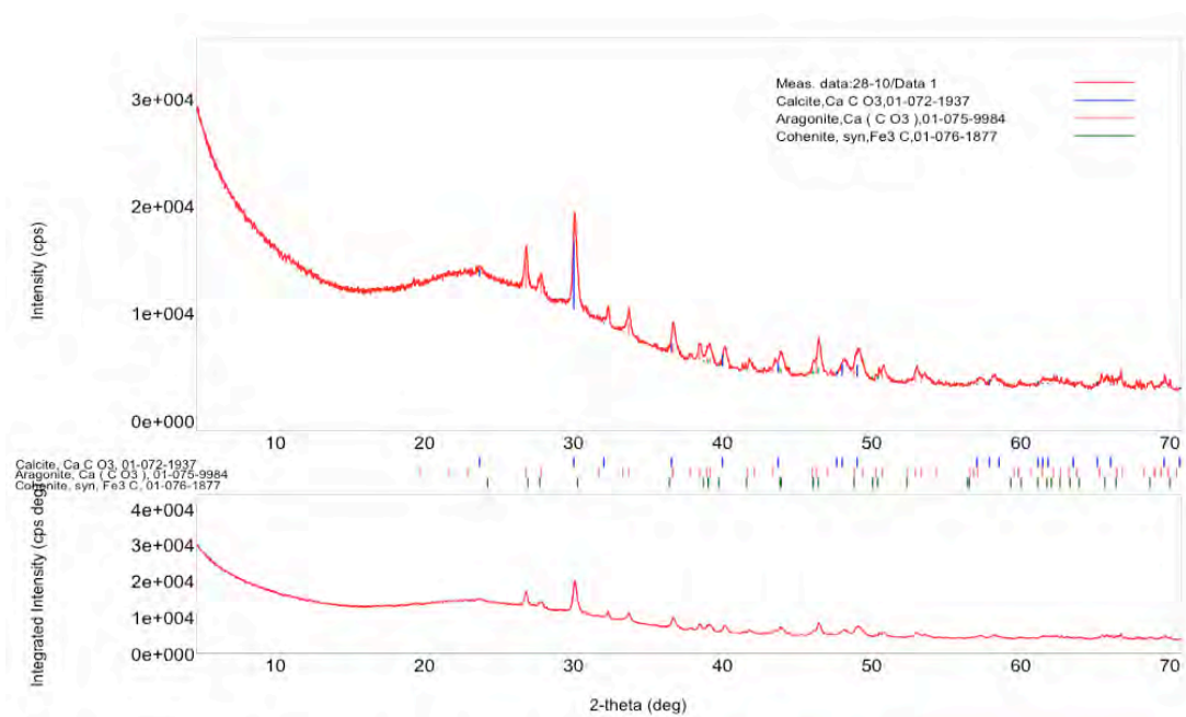
Figure 44: XRD spectra for lamina 10 of microbialite LN-13-28.
