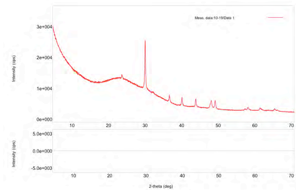
Figure 42: XRD spectra for lamina 19 of microbialite LN-13-10.
