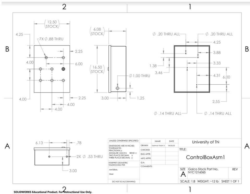
Figure 14. Hole Drawing
