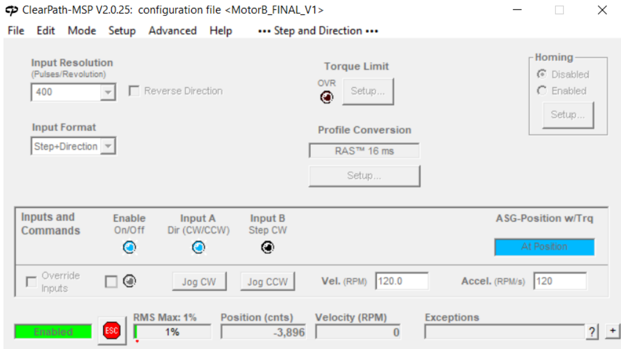
Figure 16. Screen Capture of the settings of “Motor B” (West Motor) in MSP.
