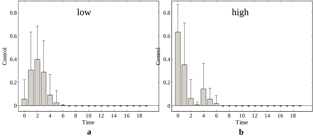
Figure 2.18: Summary statistics for the optimal control for the model with predation. Bar height represents the average value for the optimal control at each year, and the error bar is the standard deviation. Starting conditions for the control at: (a) low densities , and (b) high densities. With parameters in Table 2.3
