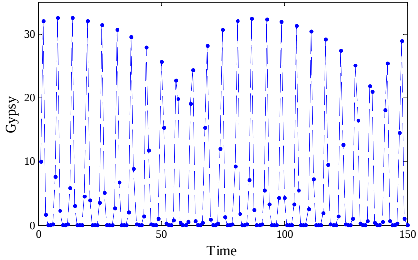
Figure 2.1: Gypsy moth population from host-pathogen model. With long-period, large-amplitude cycles in gypsy moth densities.
