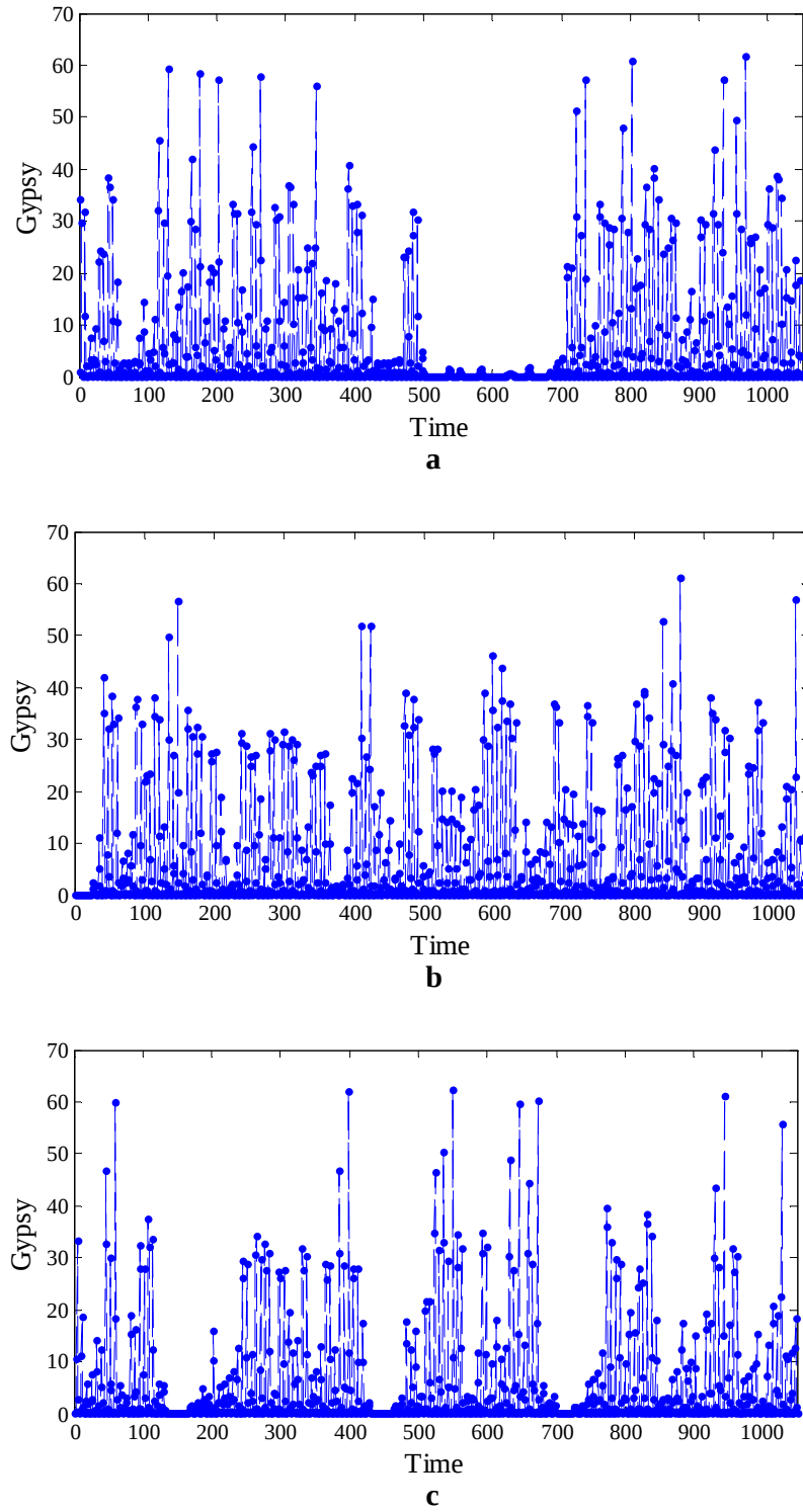
Figure 2.15: Gypsy moth population in the model with predation and with no control, for varying initial conditions. a. N_0 = 10 and Z_0 = 1 . b. N_0 = 100 and Z_0 = 100 . c. N_0 = 1000 and Z_0 = 1 , with other parameters in Table 2.3
