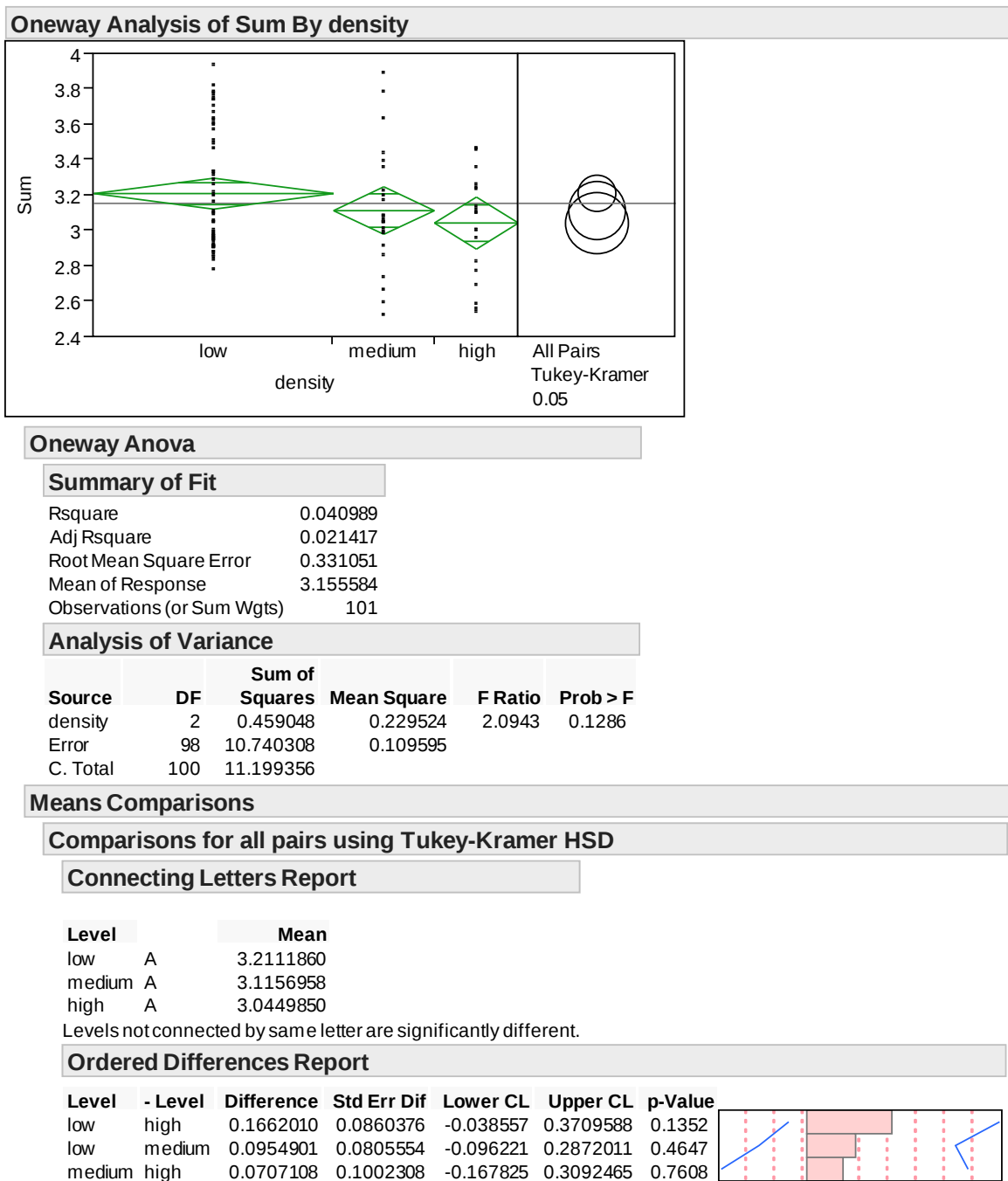
Figure A.12: Statistical analysis of the sum of the controls for different starting densities in the host-pathogen model
