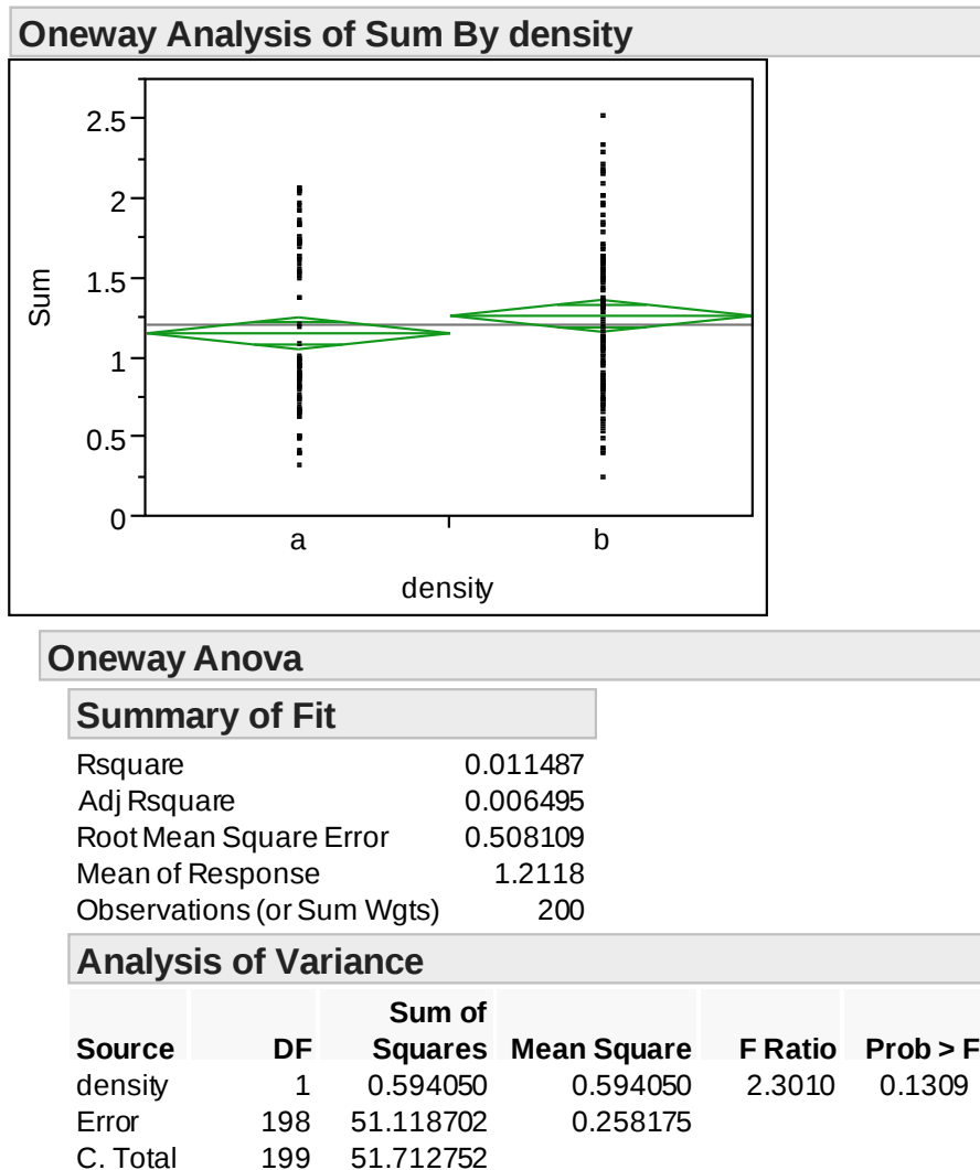
Figure A.16: Statistical analysis of the sum of the controls for different starting densities in the model with predation
