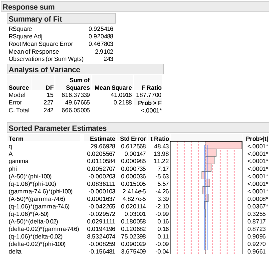
Figure A.7: Statistical analysis for the factorial experiment with the sum of controls over a period of 20 years as a response variable
