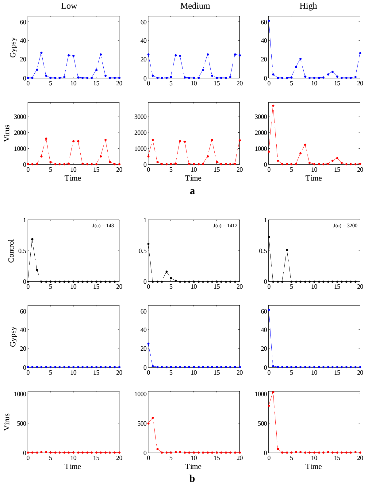
Figure A.22: Variation for starting point, low, medium and high densities of gypsy moth in the model with predation. a. Dynamics without control. b. Dynamics with control. With parameters in Table 2.3
