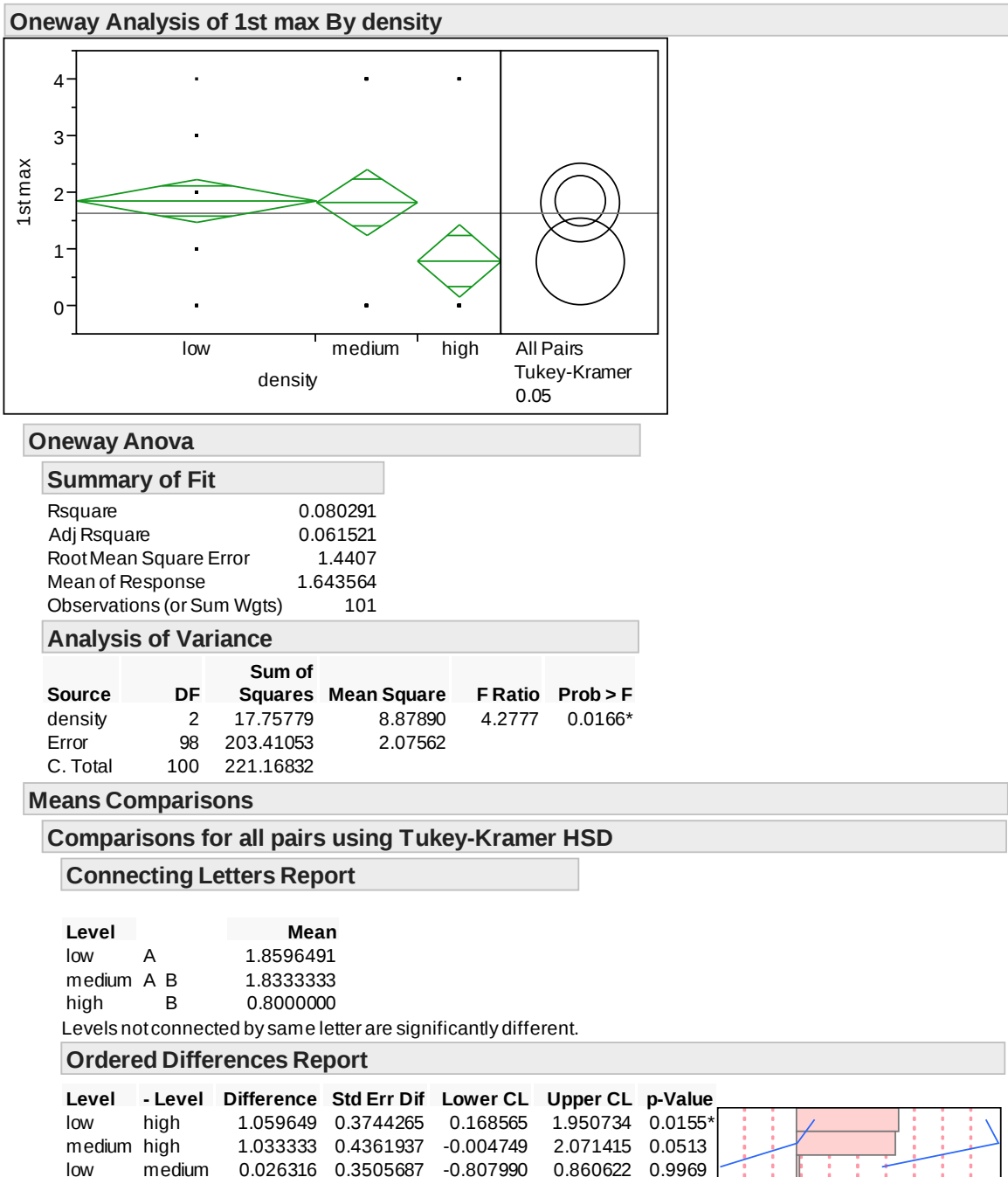
Figure A.13: Statistical analysis of the time of the maximum control for different starting densities in the host-pathogen model
