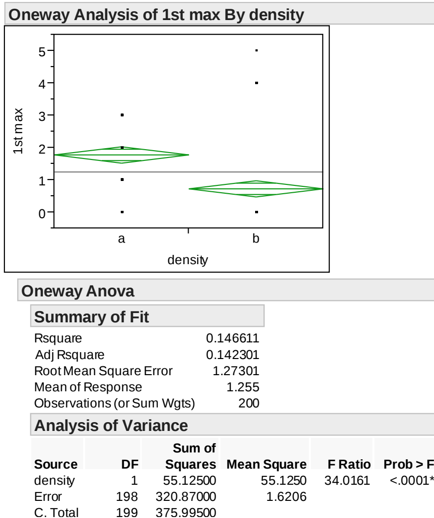
Figure A.17: Statistical analysis of the time of the maximum control for different starting densities in the model with predation
