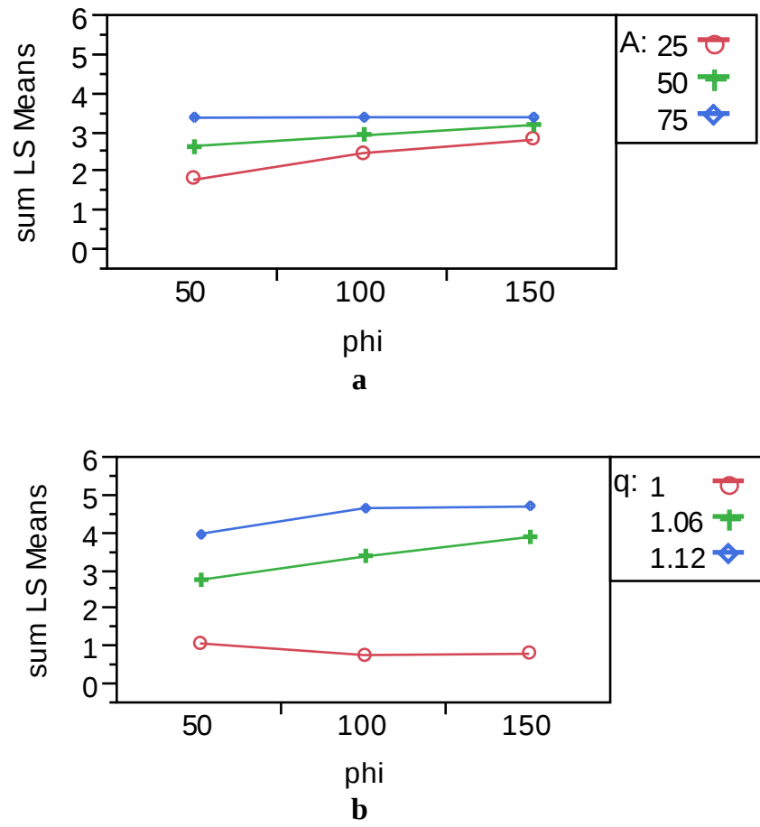
Figure A.9: Interaction plots in the host-pathogen model with sum of controls over a period of 20 years as a response variable. a A\phi . b. q\phi
