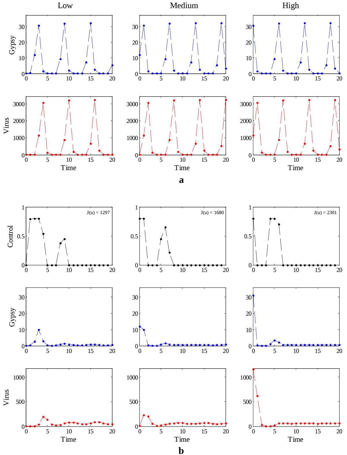
Figure 2.12: Variation for initial conditions for the optimal control, low, medium and high densities of gypsy moth in the host-pathogen model. a. Dynamics without control. b. Dynamics with control. With parameters in Table 2.1
