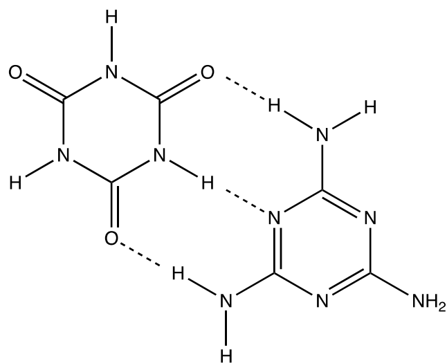
Figure 5.1 : Structure of melamine cyanurate (MC) showing hydrogen bonding between cyanuric acis (left) and melamine (right)
