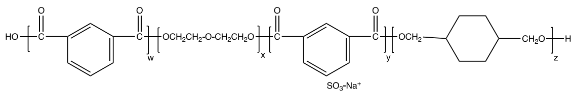
Figure 5.2 General structure of Eastman AQ series sulfopolyesters. AQ55S and AQ65S contain different ratios of the four monomeric blocks.
