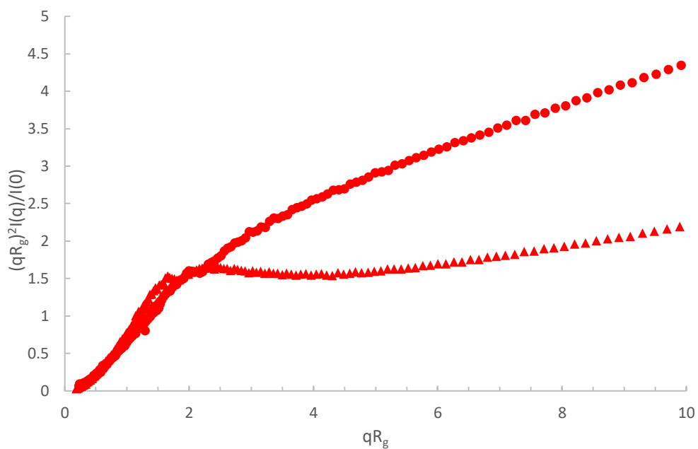
Figure 2.2 Dimensionless Kratky plot of low crosslinking nanostructures. a.) PS, b.) PEHMA; ● = 0%XL, ■ = 0.1%XL, ▲ = 0.4%XL in both plots
