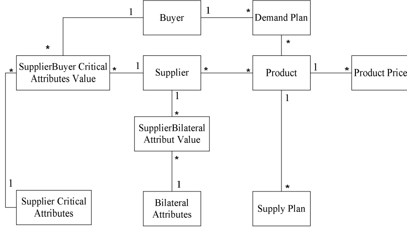
Figure 2.1: Simplified Class Diagram
