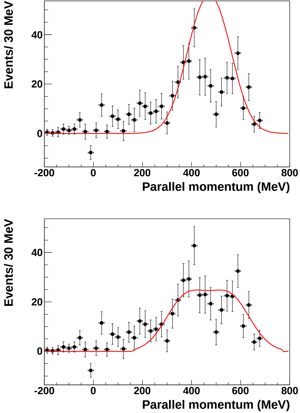
Figure 6.3: The final momentum distribution of ^{107}\text{Sn} residues in the first excited state following the one-neutron knockout from ^{108}\text{Sn} is compared to theoretical calculations assuming \ell = 2 (top) and \ell = 4 (bottom) knockout.
