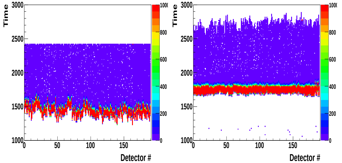
Figure 4.12: (left) Uncalibrated time plotted as a function of detector numbers. (right) Timing spectrum calibrated by shifting the times reported by each detector. The timing spectra are of a ^{88}\text{Y} source run.
