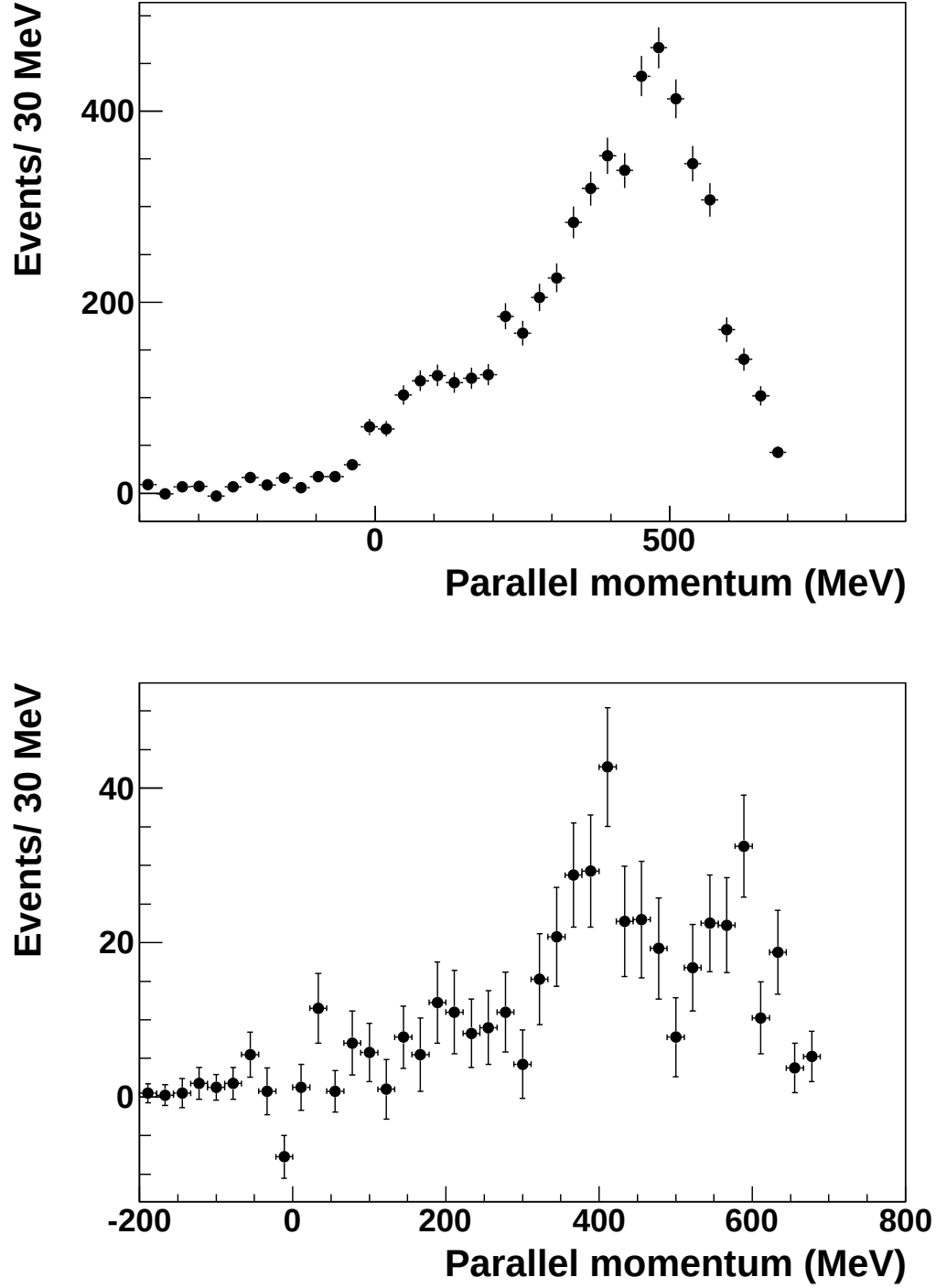
Figure 5.7: (top) The final momentum distribution for the ground state of ^{107}\text{Sn} fragment following reaction on ^{108}\text{Sn} beam. (bottom) The final momentum distribution for the first excited state of ^{107}\text{Sn} fragment following reaction on ^{108}\text{Sn} beam.
