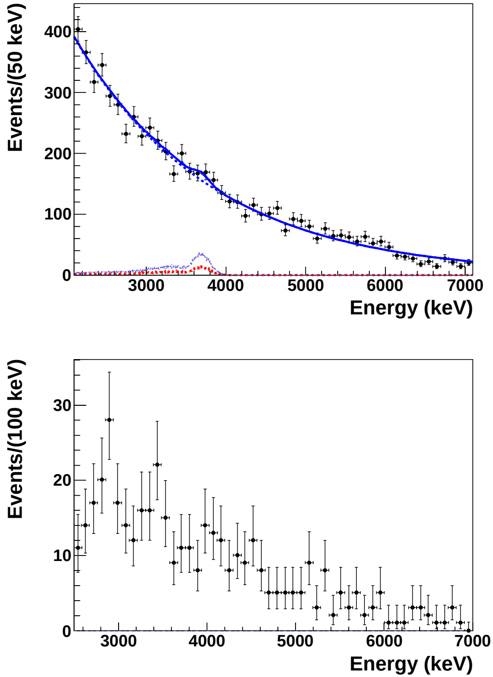
Figure 6.1: The high energy \gamma -rays are plotted for ^{107}\text{Sn} (top) and ^{105}\text{Sn} (bottom). The ^{107}\text{Sn} shows hints of a high energy \gamma -ray transition. The ^{105}\text{Sn} suffers from low statistics and makes fitting unreliable.
