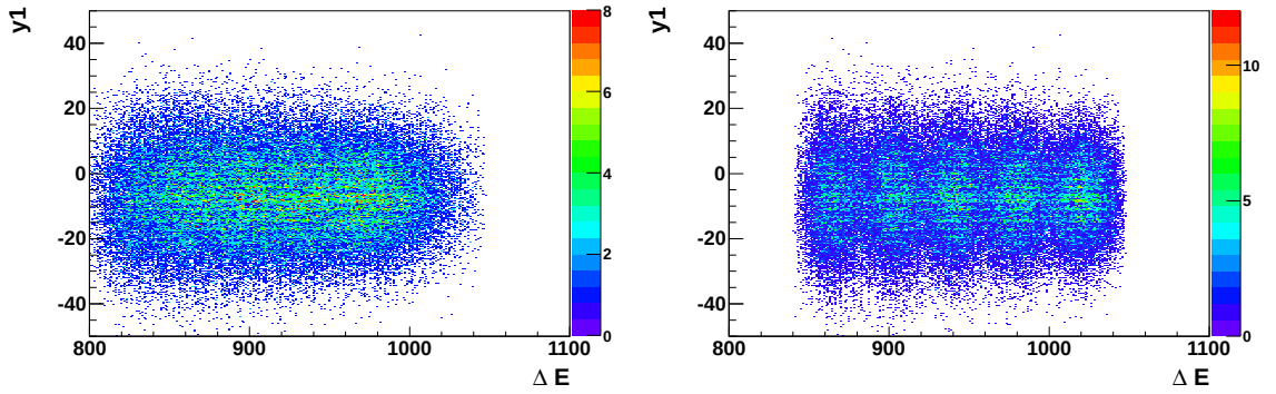
Figure 4.3: The energy loss of five isotopes are plotted with respect to the y (non-dispersive) position of the particles. In the uncalibrated (left) spectrum, the isotopes are not resolved in \Delta E . The calibrated (right) spectrum clearly shows each one.
