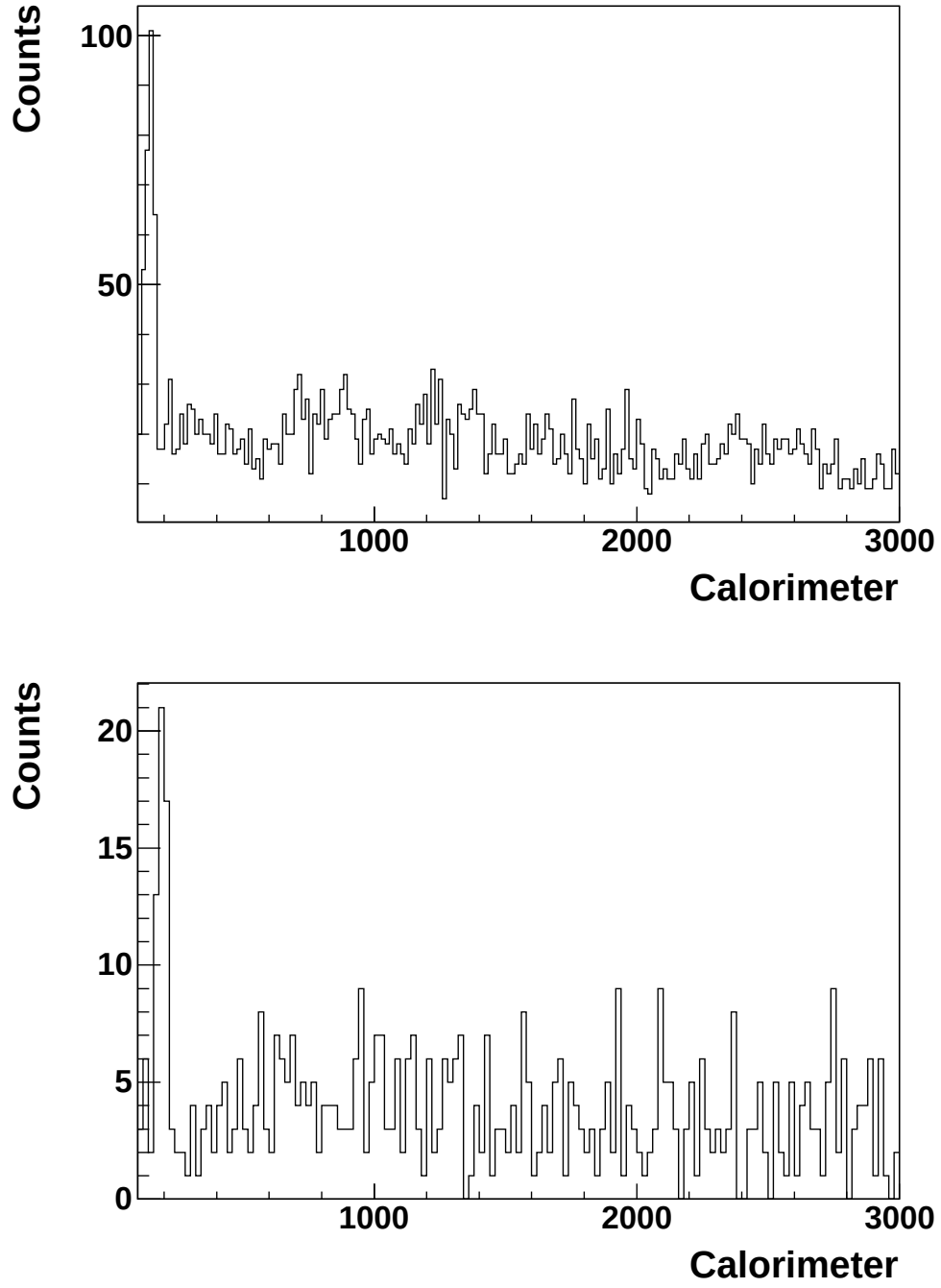
Figure 5.9: The calorimeter is the sum of all \gamma -rays in a single event. The ^{107}\text{Sn} (top) and ^{105}\text{Sn} (bottom) calorimeters provide a lower limit on the cross section for knockout to the first excited state.
