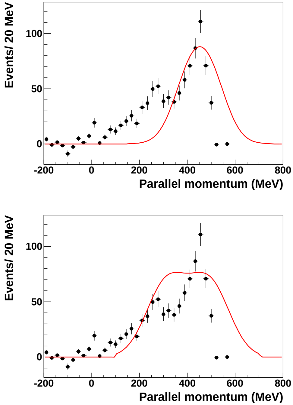
Figure 6.4: The final momentum distribution of ^{105}\text{Sn} residues in the ground state following the one-neutron knockout from ^{106}\text{Sn} is compared to theoretical calculations assuming \ell = 2 (top) and \ell = 4 (bottom) knockout.
