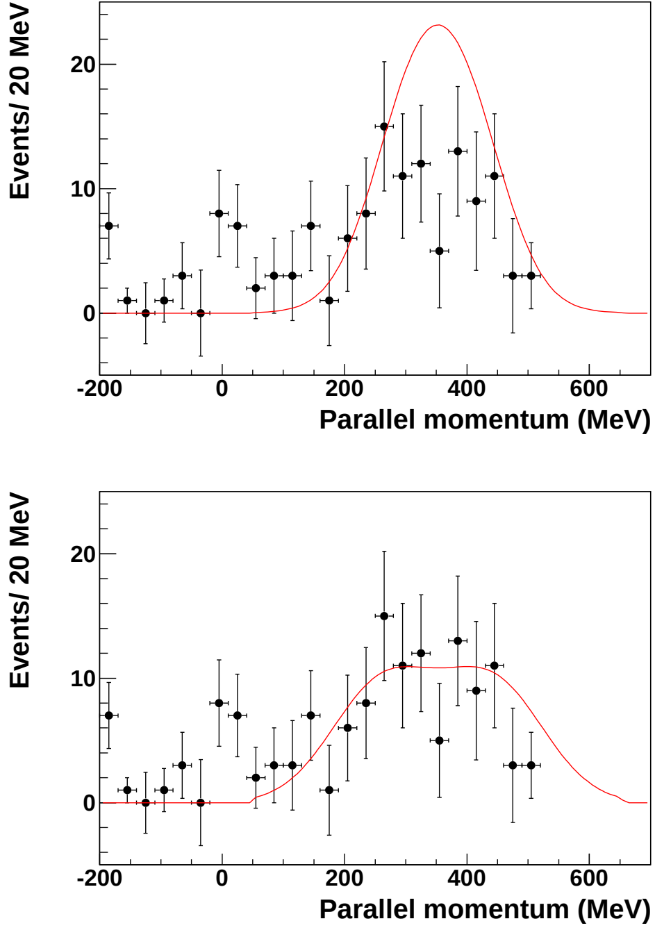
Figure 6.5: The final momentum distribution of ^{105}\text{Sn} residues in the first excited state following the one-neutron knockout from ^{106}\text{Sn} is compared to theoretical calculations assuming \ell = 2 (top) and \ell = 4 (bottom) knockout.
