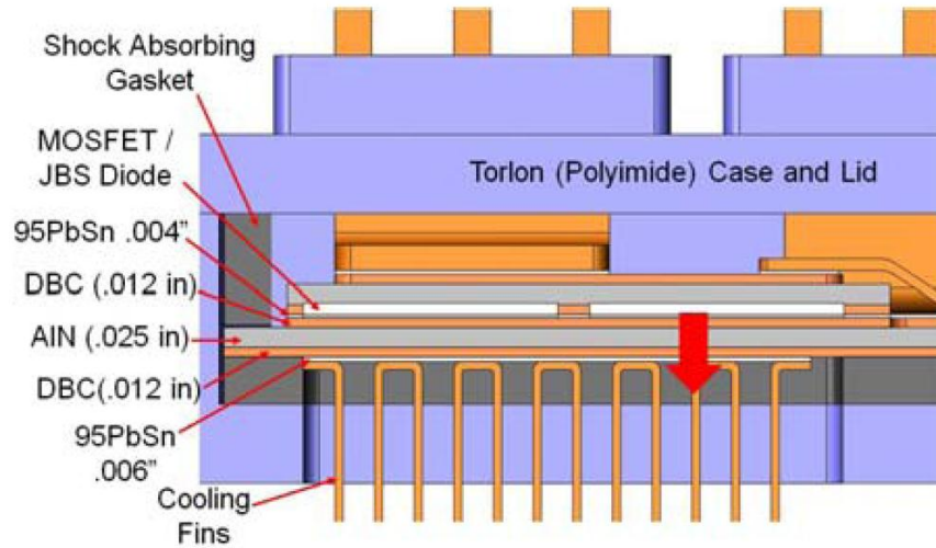
Figure 4.10 "Cross-sectional view of Gen-II design" [11]
