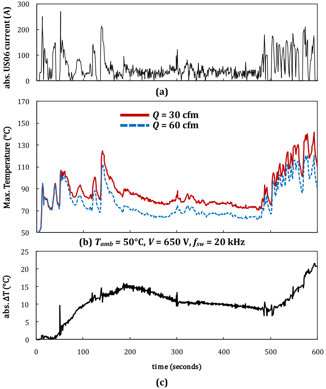
Figure 5.11 Transient thermal results for showing the affect of Q : (a) reference abs. US06 current (b) T_{max} for T_{amb} = 50^{\circ}\text{C} , V = 650 V, f_{sw} = 20 kHz (c) abs. difference of temperature profiles in (b)
