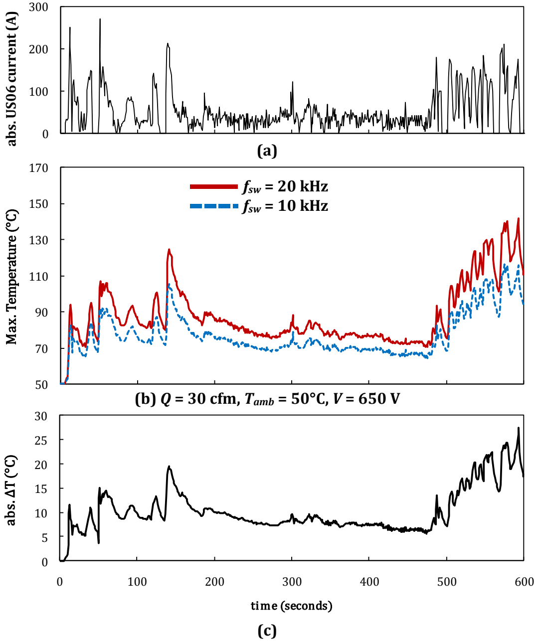
Figure 5.14 Transient thermal results showing the affect of f_{sw} : (a) reference abs. US06 current (b) T_{max} for Q = 30 \text{ cfm} , T_{amb} = 50^\circ\text{C} , V = 650 \text{ V} (c) abs. difference of temperature profiles in (b)
