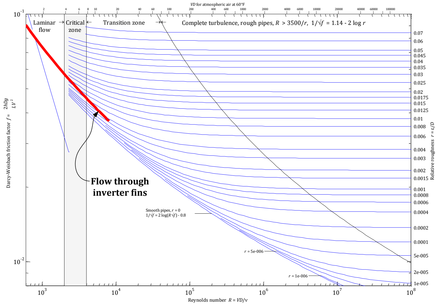
Figure 4.12 Moody diagram showing flow through inverter fins
