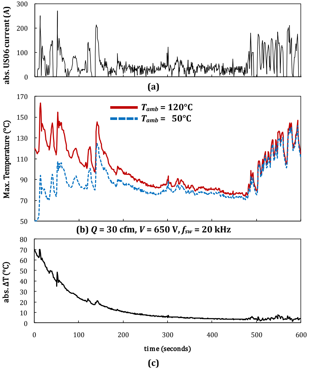
Figure 5.12 Transient thermal results showing the affect of T_{amb} : (a) reference abs. US06 current (b) T_{max} for Q = 30 \text{ cfm} , V = 650 \text{ V} , f_{sw} = 20 \text{ kHz} (c) abs. difference of temperature profiles in (b)
