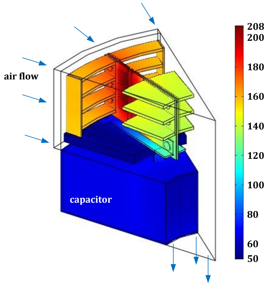
Figure 1.2 One of one of nine identical sections of the radial inflow inverter concept temperature plot ( ^{\circ}\text{C} ) [3]
