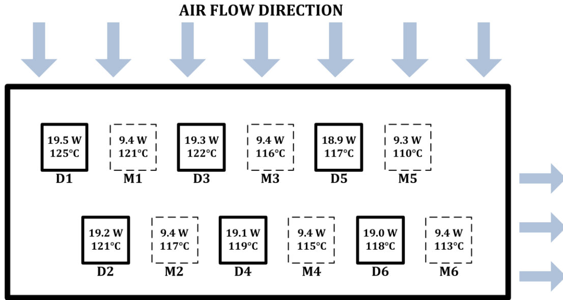
Figure 5.15 Heat generated, \dot{q} , and steady-state device temperature, T_j ( ^{\circ}\text{C} ).
