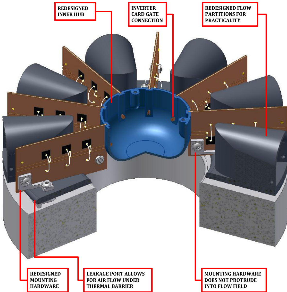
Figure 4.5 Axial inflow inverter Revision DB
