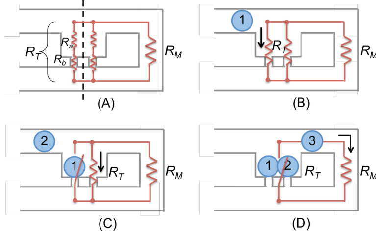
Figure 13. Schematic of hydrodynamic flow resistances in a single, 2-droplet trap. (A) Diagram of an unfilled trap designed for two droplets, where each lane of the unfilled trap has an equivalent resistance of R_a + R_b . (B) Droplet 1 enters the trap when the total trap resistance, R_T , is less than resistance of the main channel, R_M . (C) Droplet 2 enters the open lane of the same trap if R_T through the remaining portion of the trap is still less than R_M . (D) R_T becomes greater than R_M once two droplets are trapped, causing following droplets to bypass the filled trap.
