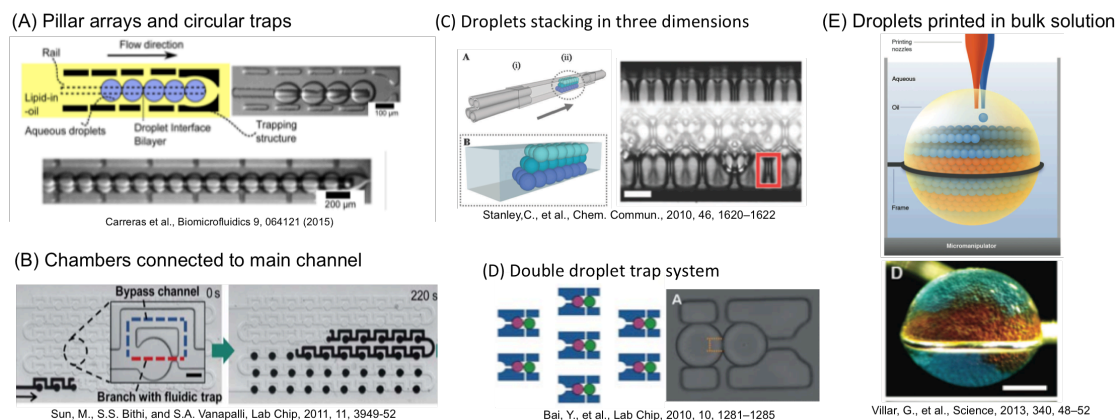
Figure 7. Microfluidic techniques used to form highly packed arrays of surfactant-stabilized droplets or discrete pairs of DIBs include (A) pillar arrays or circular traps, (B) chambers connected to the main channel, (C) stacking droplets in 3D to fill a channel, (D) a double droplet trap system, and (E) droplet printing.
