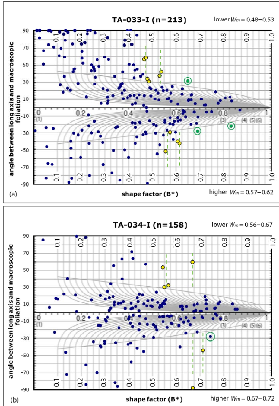
Figure 4-4. Difference comparison of TA-033-I (a) and TA-034-I (b) via RGN plot, data points in blue. Green dashed lines indicate the upper and lower range of W_m . Yellow dots encircled in black indicate the critical data points that were employed to draw the upper and lower boundaries of W_m . Outliers consist of green dots enclosed in a green circle. All data were collected from feldspar porphyroclasts.
