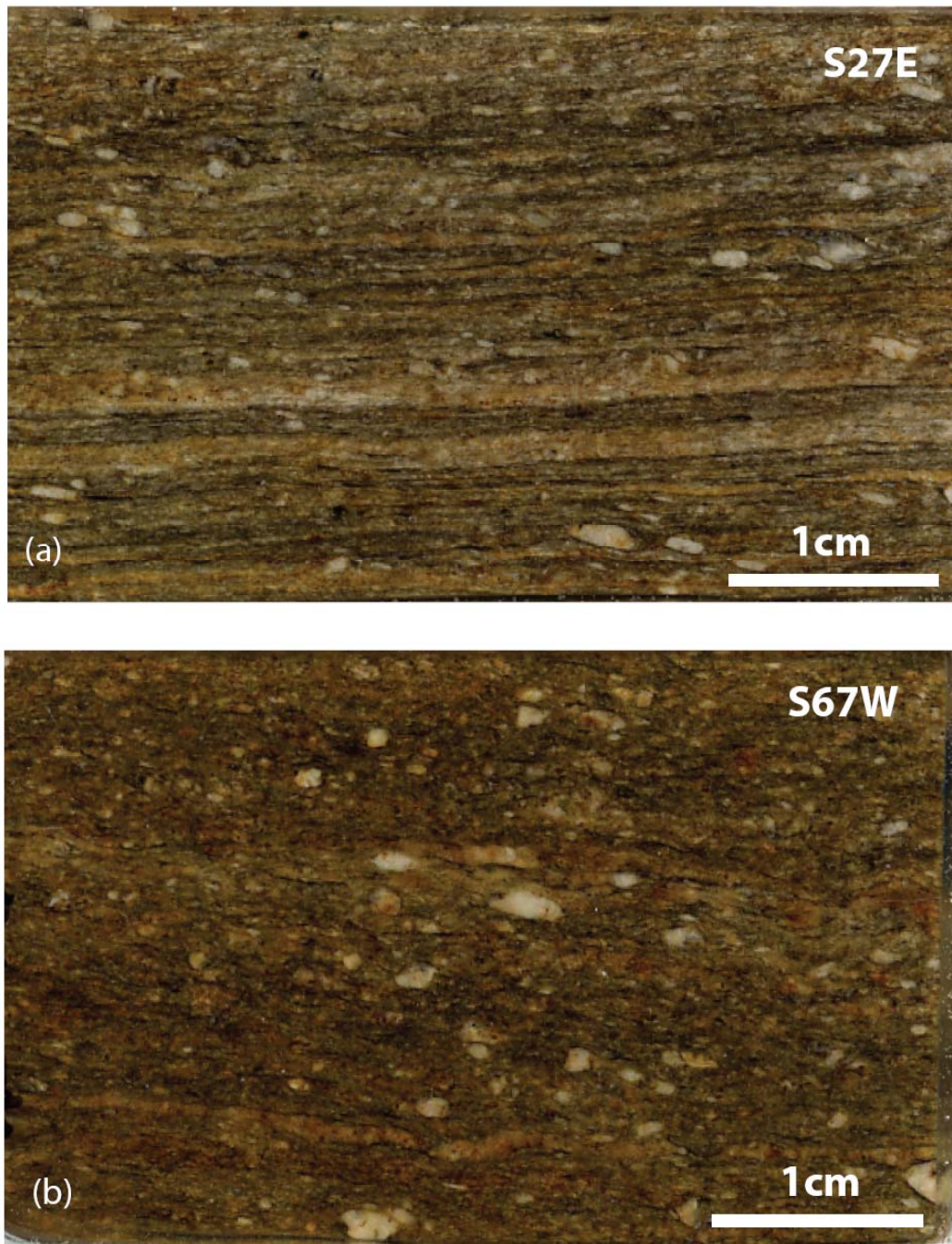
Figure 1-7. Scanned rock chips. Feldspar porphyroclasts in the fine-grained matrices of MHG. Samples were collected from US-76, Whetstone quadrangle, SC (N 34° 45.395', W 083° 14.366'). Oriented samples (a) and (b) illustrate the banded texture parallel and perpendicular to mineral lineation, respectively.
