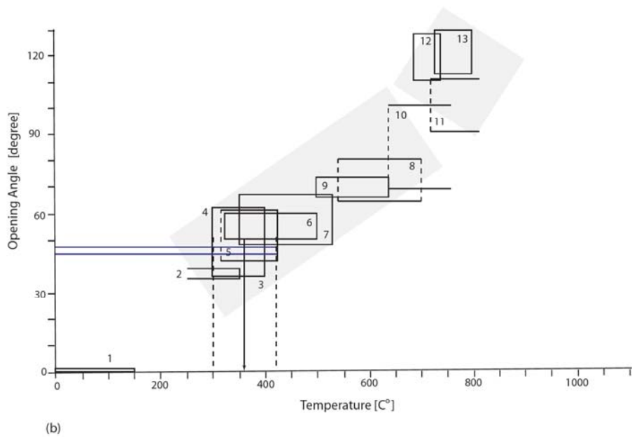
Figure E-1. Quartz c-axis central girdle opening angle (a). Possible deformation temperature (b) (after Kruhl, 1998).
