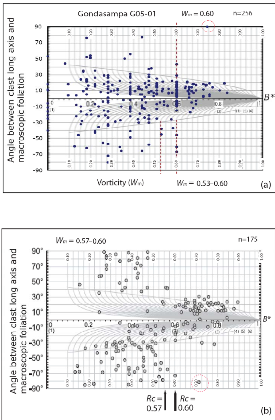
Figure 3-9. Comparison of the calibration result (a) and the result (b) from Jessup et al. (2007).
