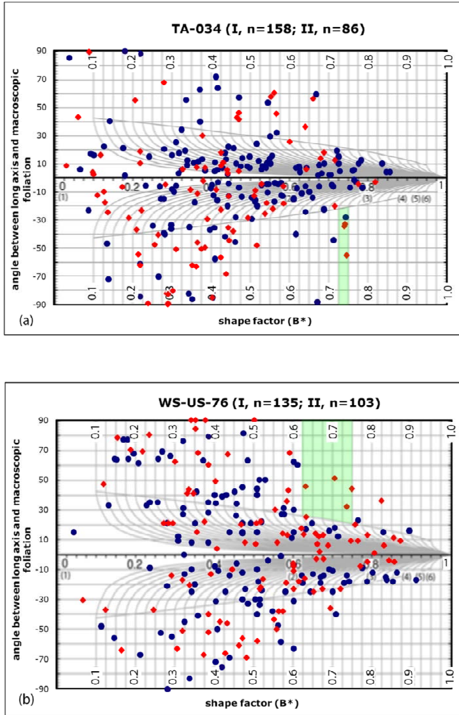
Figure 4-3. Using RGN diagrams to compare XZ- and YZ- plane. Samples TA-034 (a) and WS-US-76 (b). Blue and red dots represent W_m estimates in the XZ- and YZ-planes, respectively. Discrepancy is highlighted in green. All data were collected from feldspar porphyroclasts.
