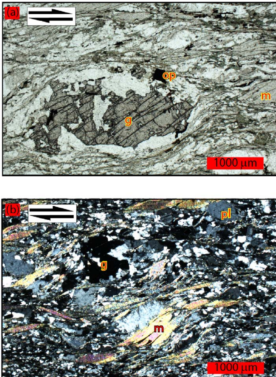
Figure 3-4. Photomicrograph of MG sample WS-027-I from SC 28, Whetstone quadrangle, SC. (a) skeletal garnet in plane light. (b) mica fish in MG (crossed polars). m = muscovite; g = garnet; pl = plagioclase; op = opaque. Shear sense is top-to-the-right.
