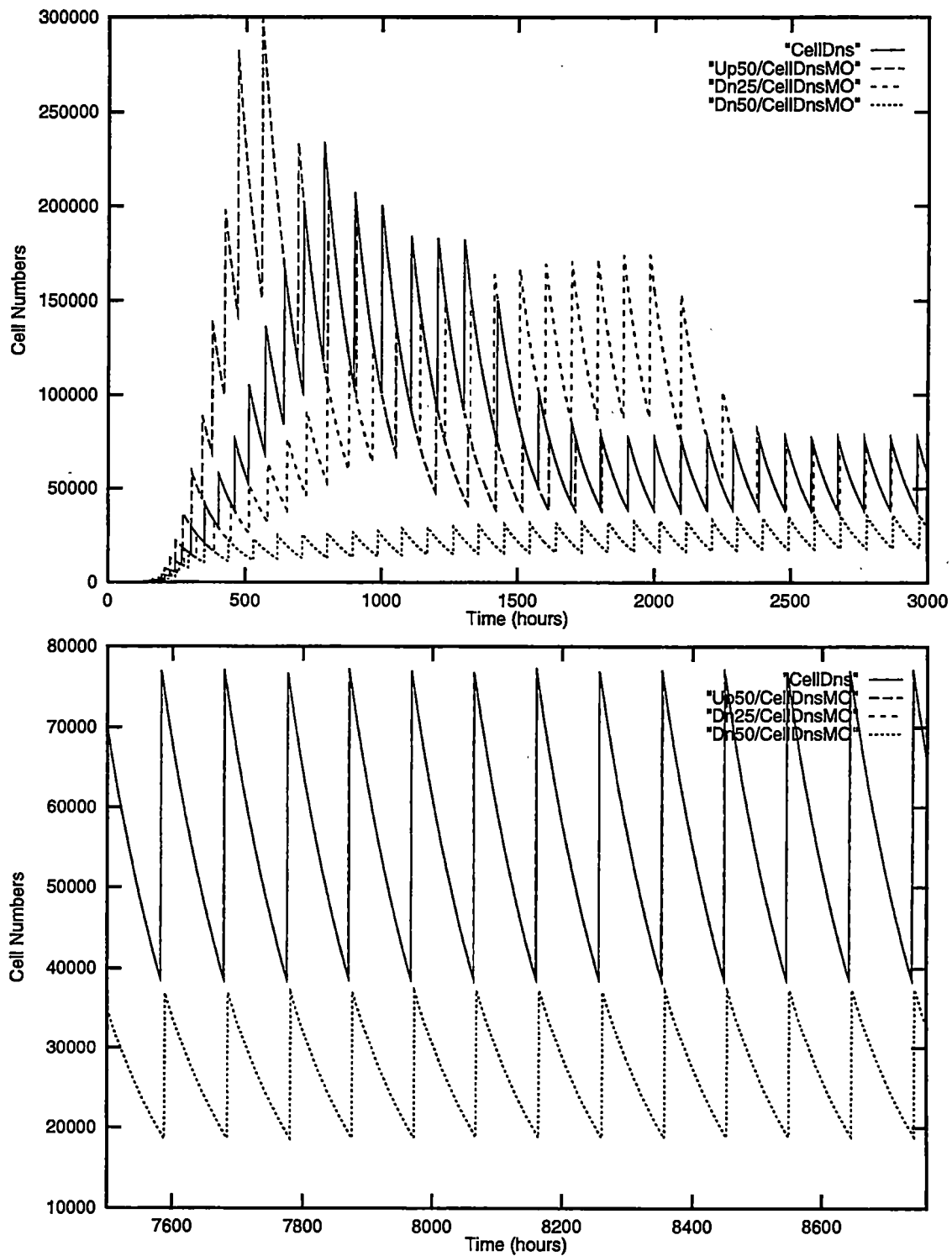
Figure 2.10: Transient and steady state behavior of 50% increase and 25% and 50% decrease in original M_O value in a silicate limited system.
