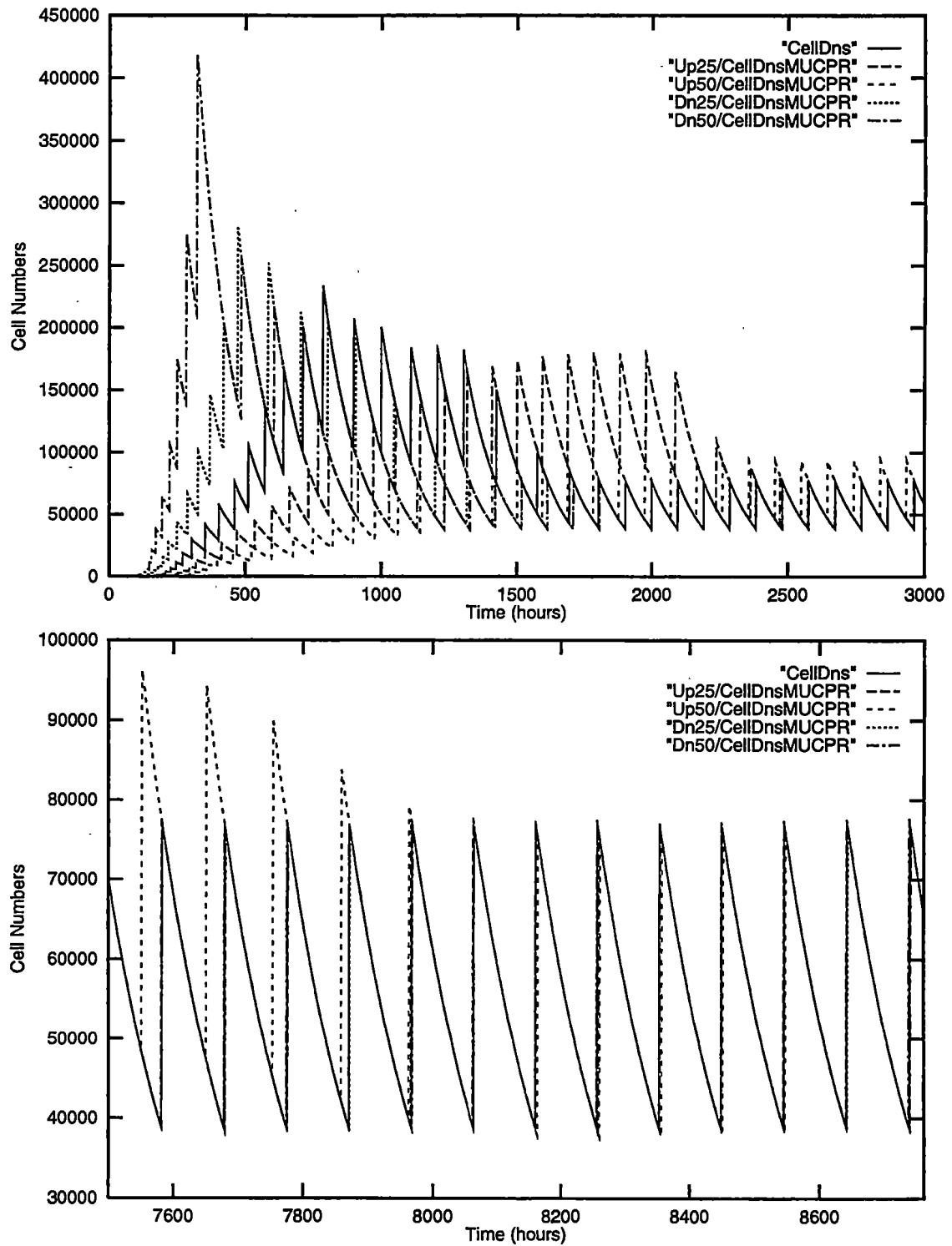
Figure 2.11: Transient and steady state behavior of 25% and 50% increase and 25% and 50% decrease in original \mu_{C,Pr} value in a silicate limited system.
