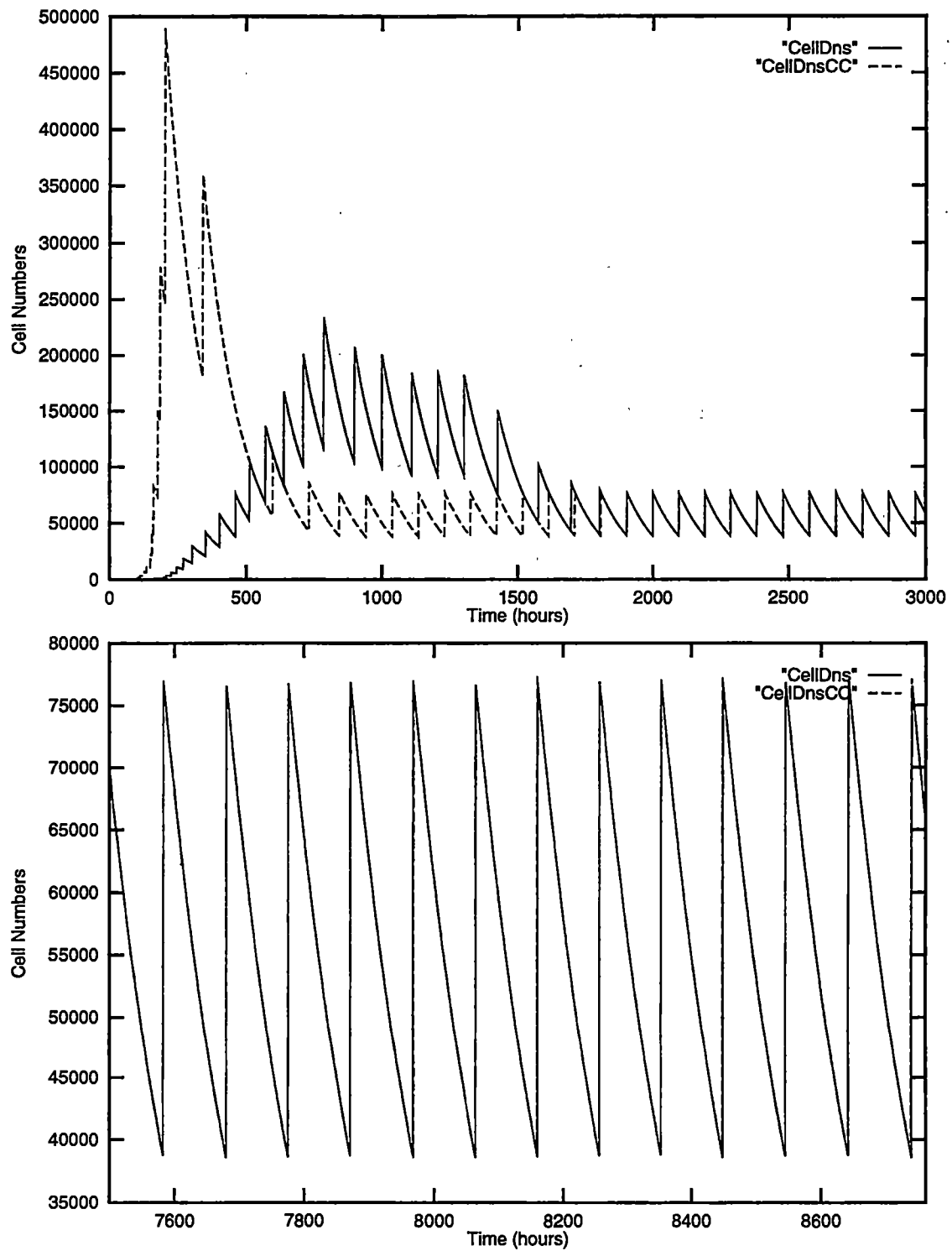
Figure 2.9: Transient and steady state behavior of 50% decrease in original c'_C value in a silicate limited system.
