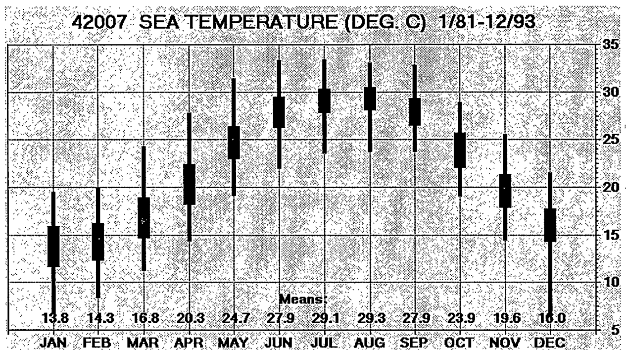
Figure B.1: Data from anchored buoy, south-southeast of Biloxi, Mississippi
