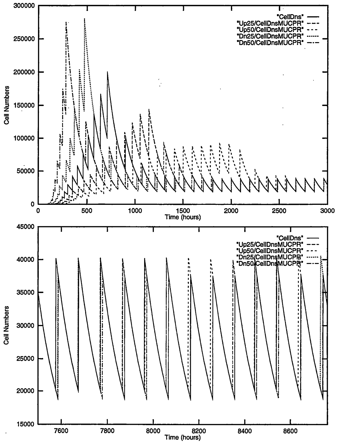
Figure 2.27: Transient and steady state behavior of 25% and 50% increase and 25% and 50% decrease in original \mu_{C,Pr} value in a nitrogen limited system.
