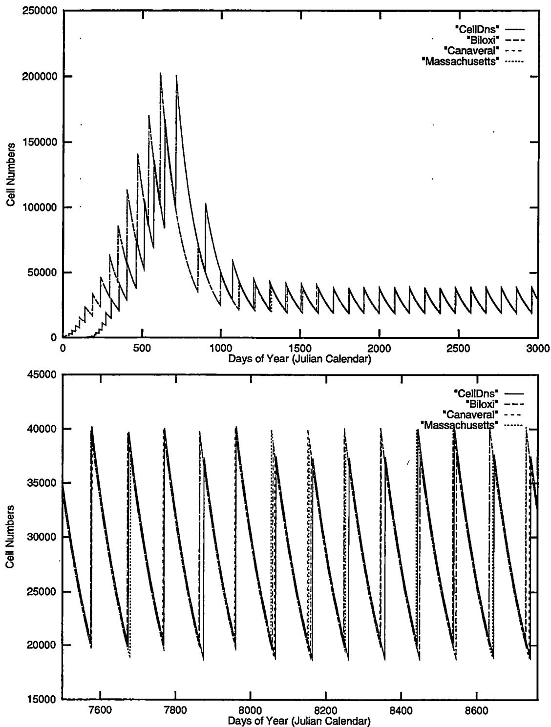
Figure 3.5: Nitrogen limited system (CellDns) simulated with temperature curves for Biloxi, Mississippi (Biloxi), Cape Canaveral, Florida (Canaveral), and Boston, Massachusetts (Massachusetts)
