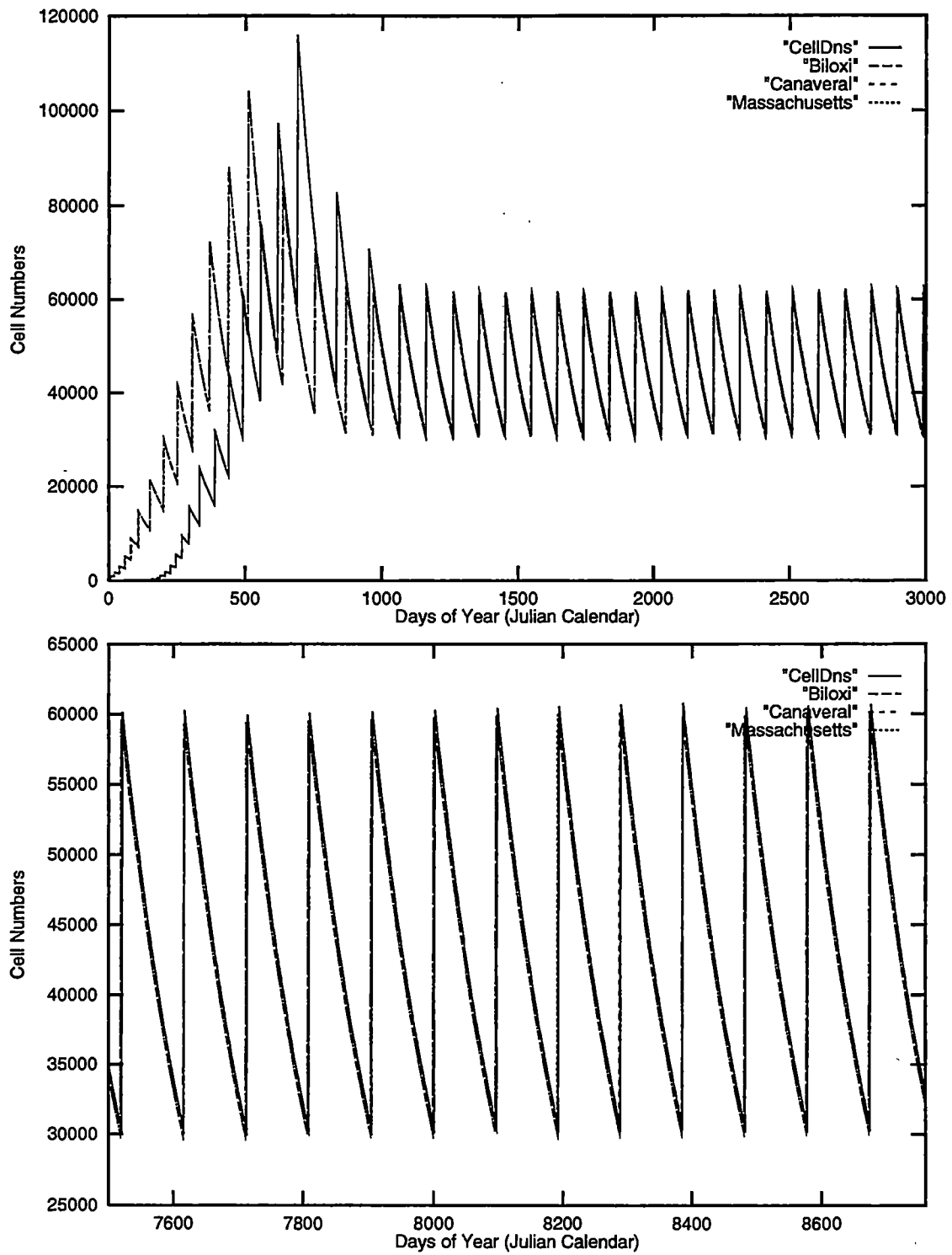
Figure 3.4: Phosphorous limited system (CellDns) simulated with temperature curves for Biloxi, Mississippi (Biloxi), Cape Canaveral, Florida (Canaveral), and Boston, Massachusetts (Massachusetts)
