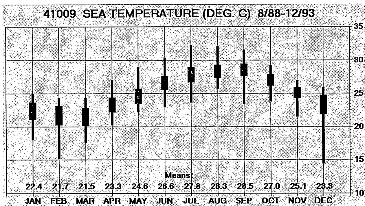
Figure B.2: Data from anchored buoy, Cape Canaveral, Florida
