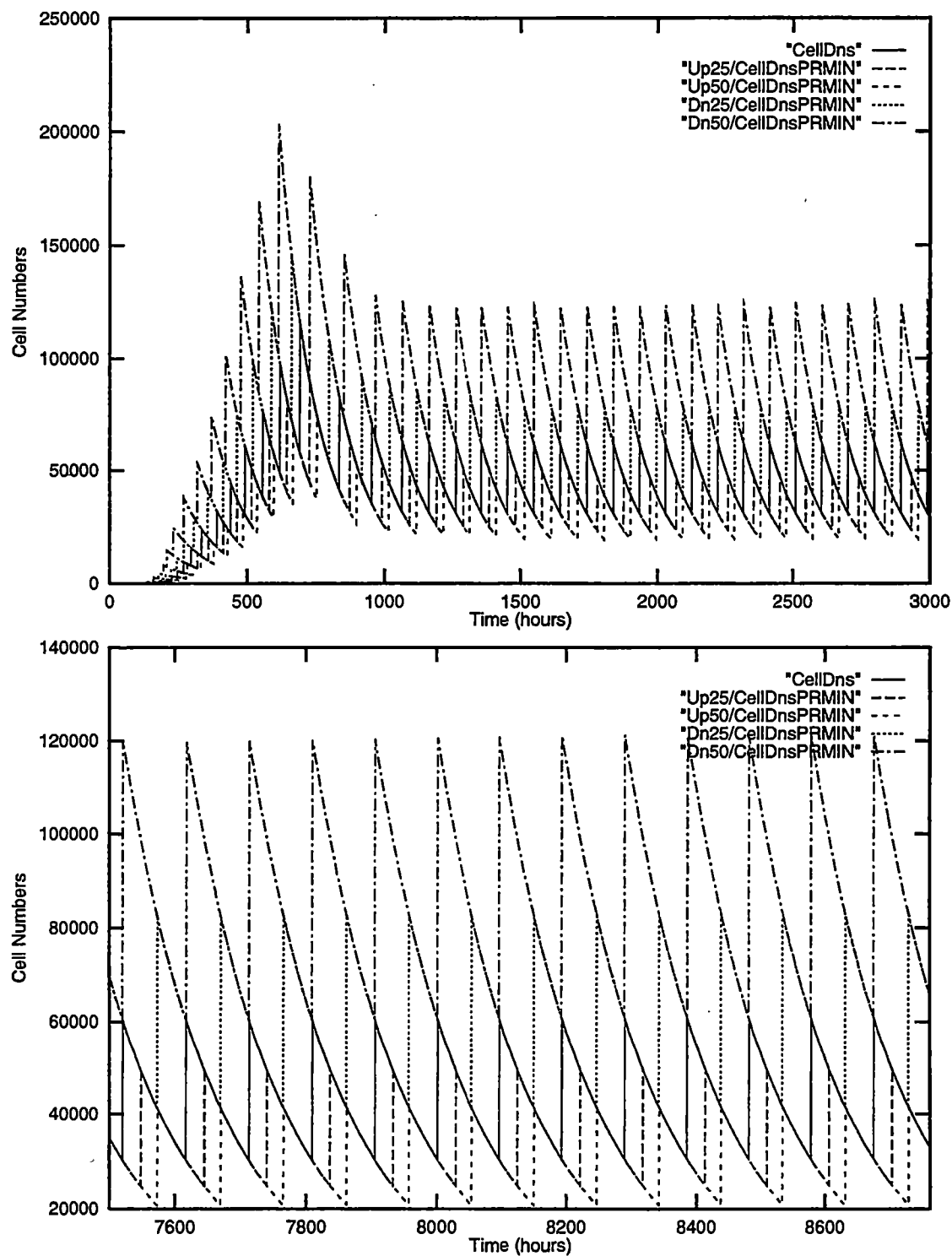
Figure 2.23: Transient and steady state behavior of 25% and 50% increase and 25% and 50% decrease in original Pr_{min} value in a phosphorous limited system.
