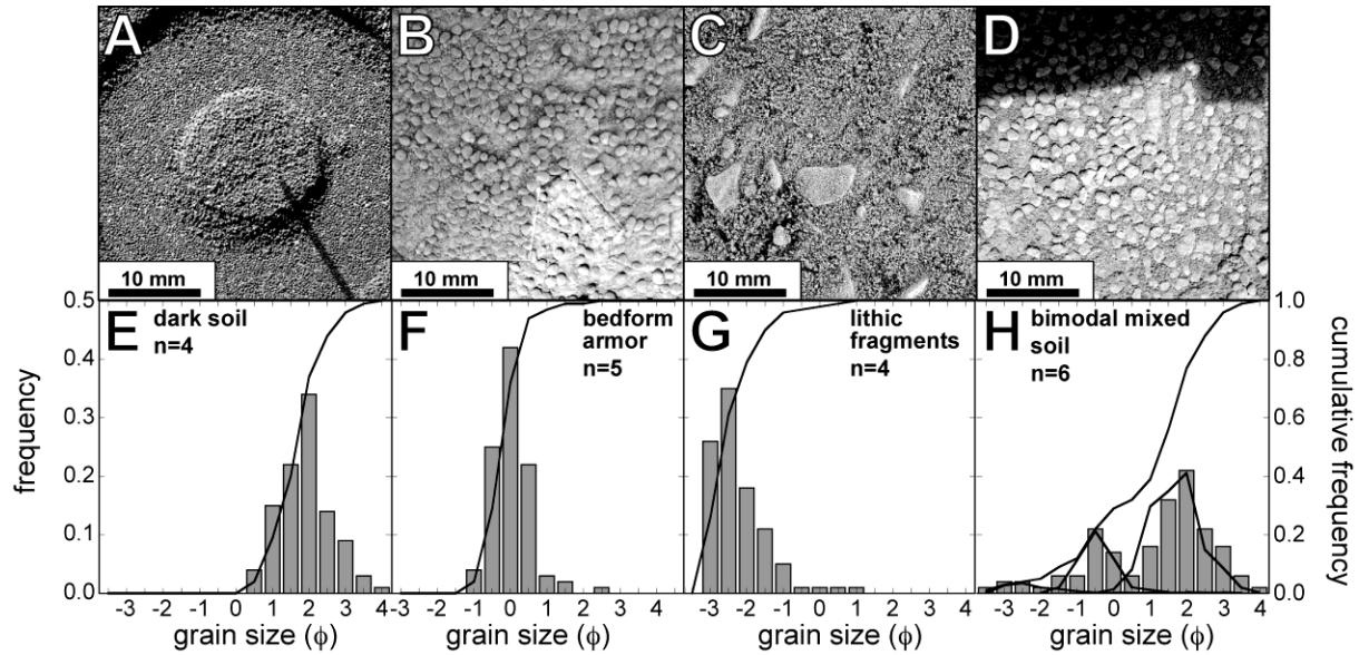
Figure 2.3. Major soil classes grouped by grain sizes and representative soil targets viewed by the microscopic imager (MI). Dust ( < 100 \mu\text{m} ) is present in most soils. (a) Dark soil (El Dorado shadow sol 709); (b) bed form armor (Arena Crest sol 41); the upper part of image has been adjusted to remove a shadow for clarity; (c) lithic fragments (Grande Flats Trout 1 sol 46); (d) bimodal mixed soil (Pequod Doubloon sol 499); (e) mean grain size histogram for dark soil; (f) mean grain size histogram for bed form armor soil; (g) mean grain size histogram for lithic fragment soil; (h) mean grain size distribution of bimodal mixed soil.
