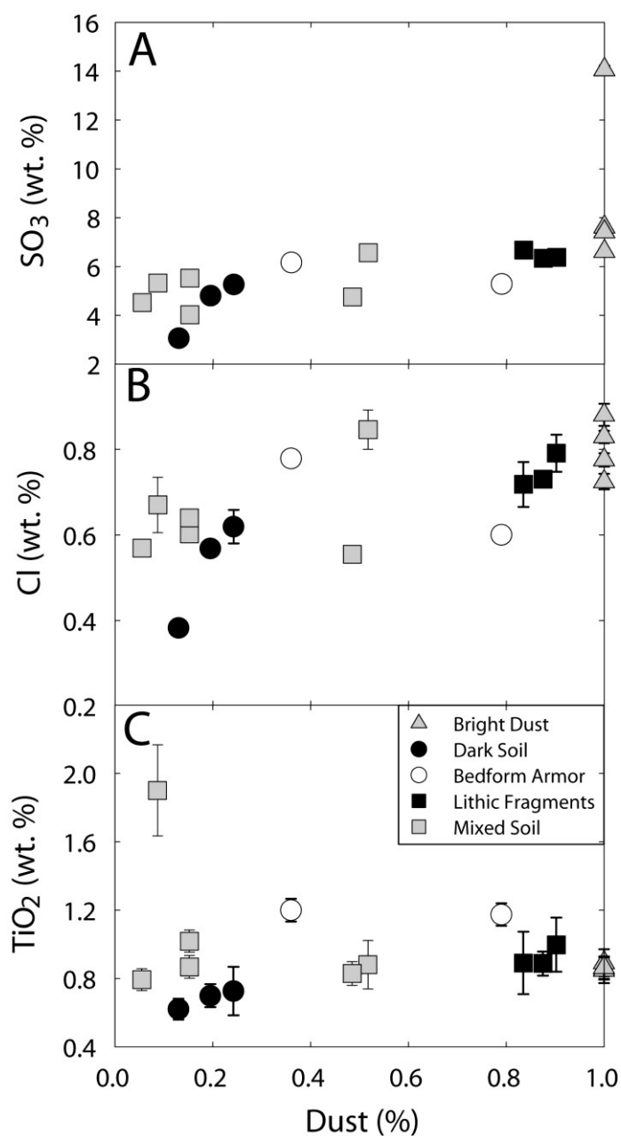
Figure 3.4. Gusev soils blanketed with fines ( <100\ \mu\text{m} ) surface dust (bright dust) or with high dust cover (lithic fragments) are generally enriched in (A) sulfur ( \text{SO}_3 ) and (B) chlorine (Cl) when compared to relatively dust free surfaces, confirming a \text{SO}_3 + \text{Cl} dust component. (C) Concentrations of \text{TiO}_2 are homogeneous, and are independent of dust fraction.
