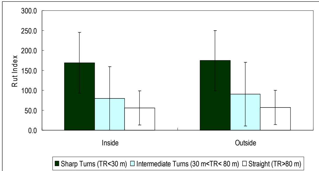
Fig. 2-17 Rut index of the APC.
