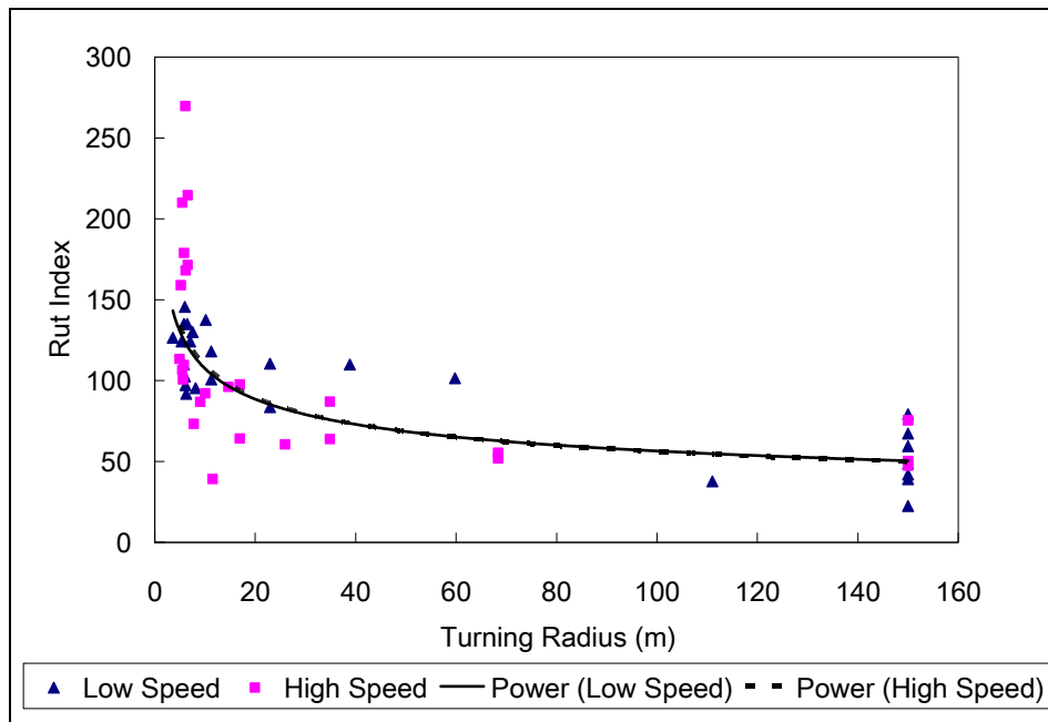
Fig. 3-17 Relationship between HMMWV turning radius and outside rut index influenced by vehicle speeds.
