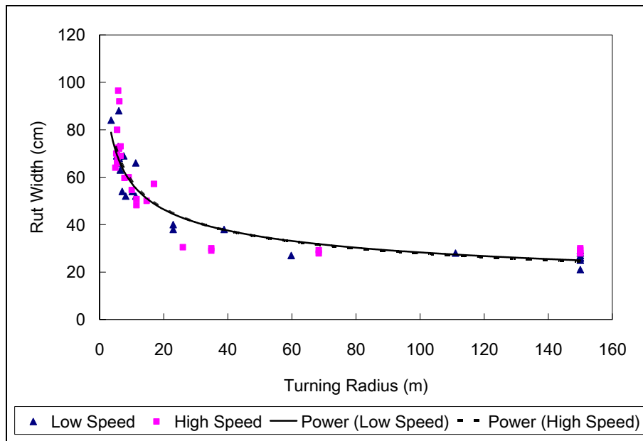
Fig. 3-12 Relationship between HMMWV turning radius and inside rut width influenced by vehicle speeds.
