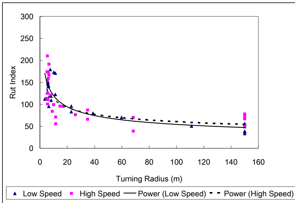
Fig. 3-16 Relationship between HMMWV turning radius and inside rut index influenced by vehicle speeds.
