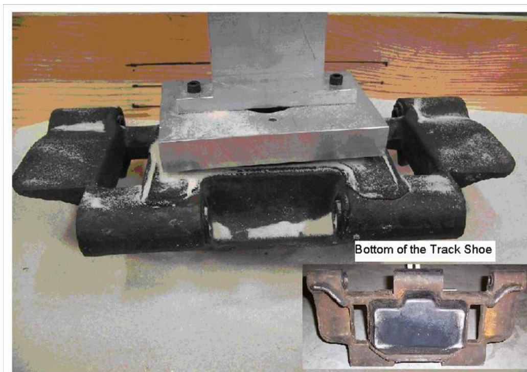
Fig. 5-4 Track shoe.
