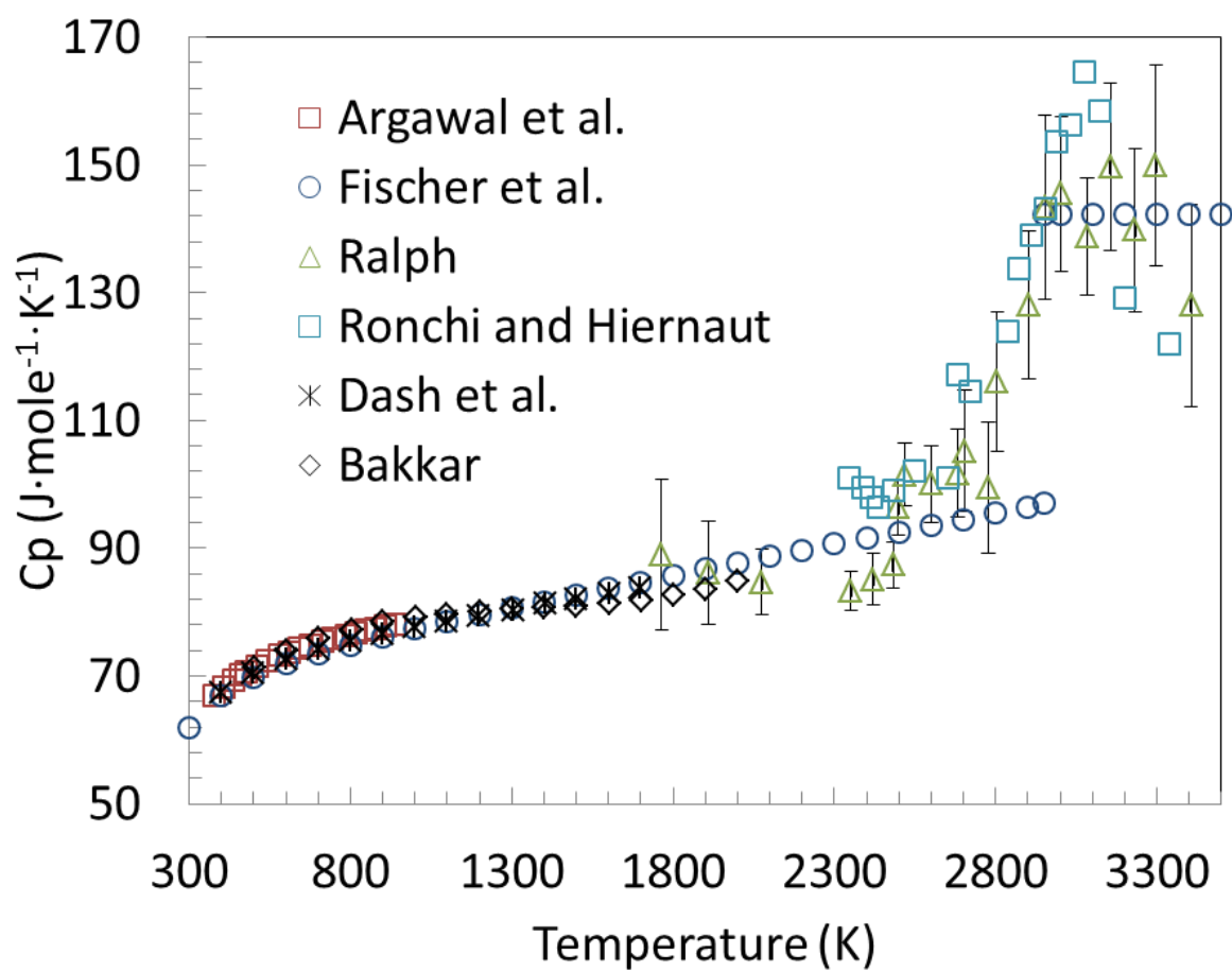
Fig. 3.13. Experimentally determined molar heat capacity from the studies for \text{ThO}_2 [69, 72-76] reviewed in this work.
