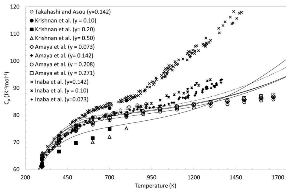
Fig. 6.9. Computed (lines) and experimental molar heat capacity ( c_p ) data (points) versus temperature for \text{U}_{1-y}\text{Gd}_y\text{O}_2 . The dashed line represents the c_p for \text{UO}_2 computed from the CEF model.
