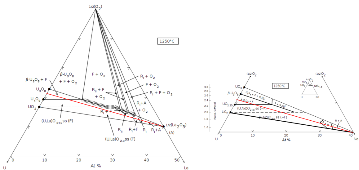
Fig. 3.8. Experimentally determined phase diagrams from [62] and [63]. The red line shows the oxygen rich extent of the fluorite phase considering U^{5+} as the maximum oxidation state. (Reprinted with permission of The American Ceramic Society, www.ceramics.org All rights reserved.)
