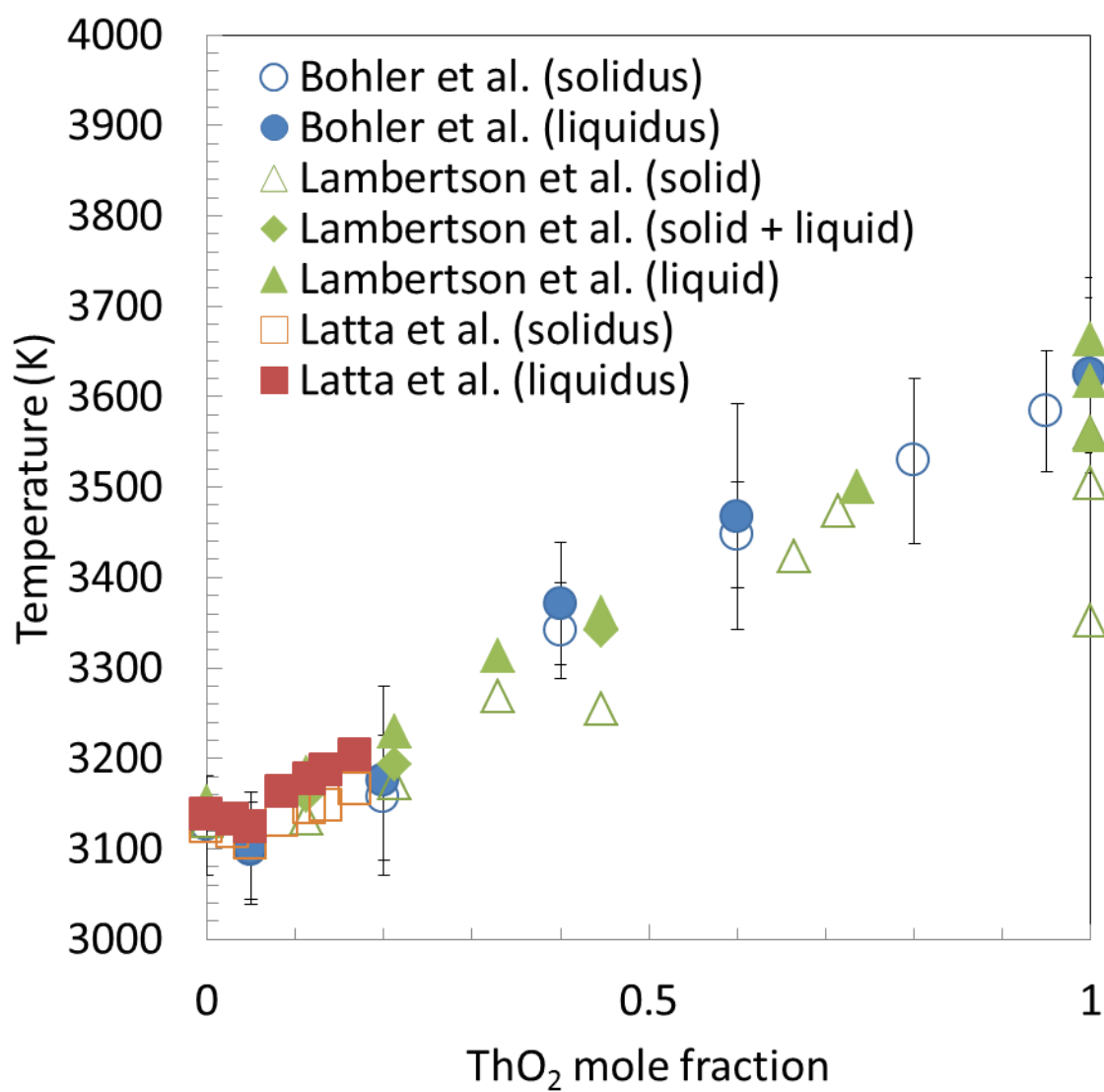
Fig. 4.6. Solidus (open symbols) and liquidus (closed symbols) data from [151-153] along the UO 2 -ThO 2 pseudobinary isopleth.
