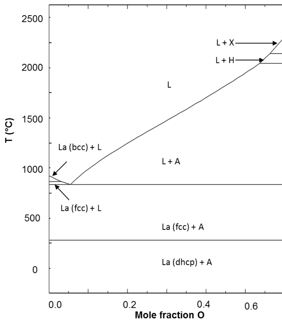
Fig. 6.10. The La-O binary phase diagram computed using the ideal partially ionic two-sublattice liquid model parameters derived from optimization of the inferred pseudo-binary \text{UO}_2\text{-LaO}_{1.5} system.
