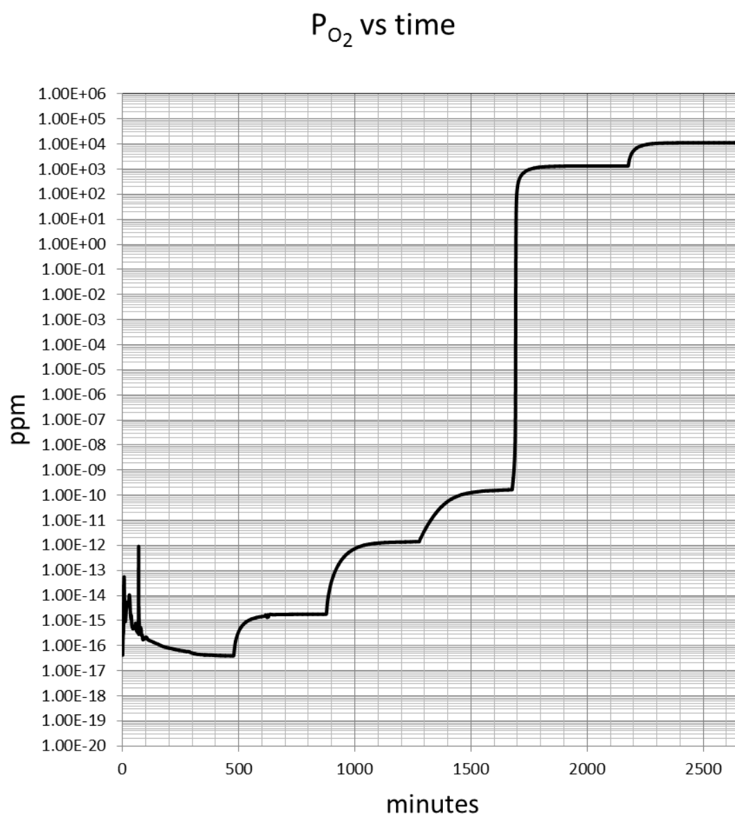
Fig. 5.3. The measured O_2 concentration from the Centorr unit using the test gas combinations given in Table 5.1 to verify instrument calibration.
