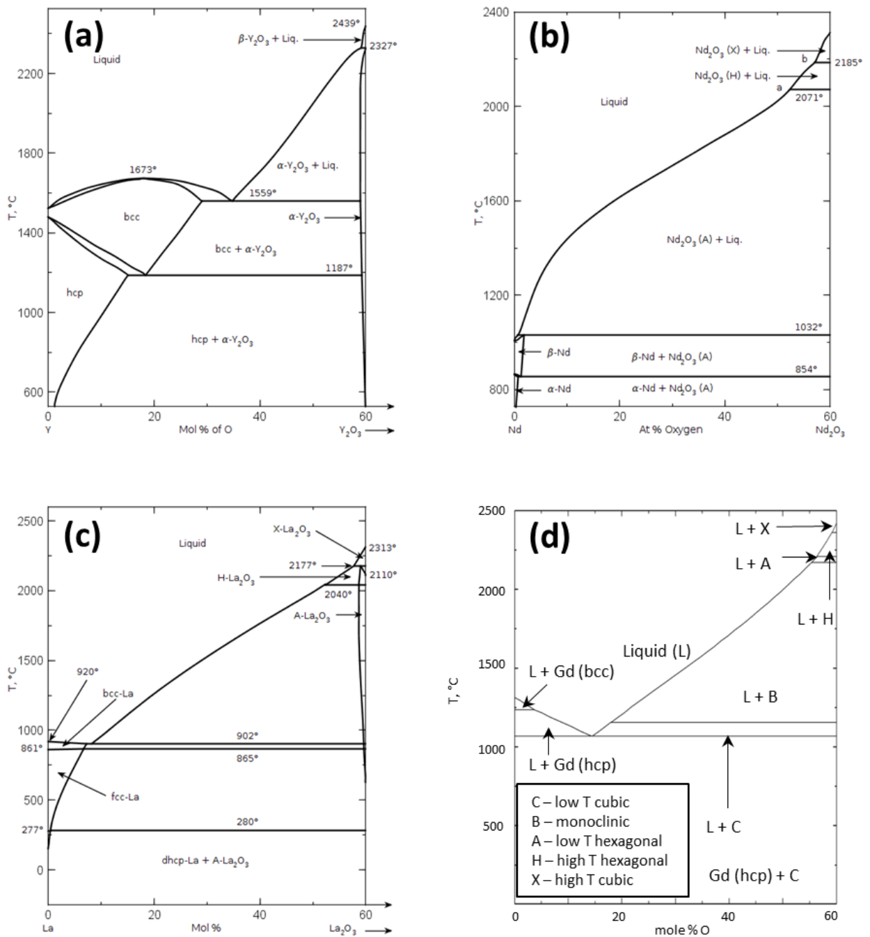
Fig. 6.3. Reported phase diagrams for the Y-O (a) Nd-O (b) and La-O (c) systems from [102, 105, 107]. (Reprinted with permission of The American Ceramic Society, www.ceramics.org All rights reserved.) The tentative T-x phase diagram for the Gd-O from this work is shown in (d) . (Gd 2 O 3 polymorphs: C=low temperature cubic, B=monoclinic, A=low temperature hexagonal, H=high temperature hexagonal, X=high temperature cubic).
