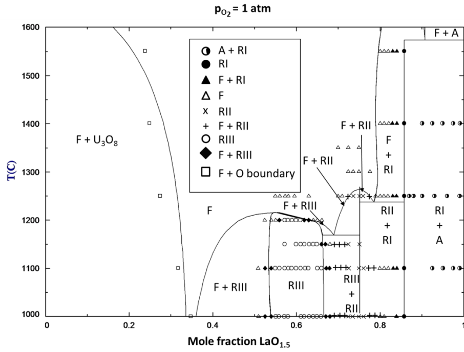
Fig. 6.14. Computed pseudo-binary diagram (lines) of fully oxidized U-La with the experimentally determined phase relations from [62] (points) shown as well. (F=fluorite solid solution, RI=rhombohedral \text{ULa}_6\text{O}_{12-x} , RII= rhombohedral \text{U}_2\text{La}_6\text{O}_{15} , A=hexagonal \text{La}_2\text{O}_3 , O=orthorhombic \text{U}_3\text{O}_8 )
