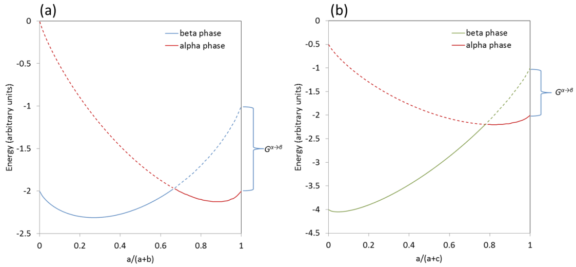
Fig. 3.4. Gibbs curves from the ideal solution model as a function of composition for the \alpha and \beta phases in the hypothetical a-b and a-c systems. The dashed lines represent “extrapolations” into the unstable phase regions. The difference between the extrapolated end points and the pure stable phase is the lattice stability. Note that the lattice stability for pure a in both the a -b and a -c binaries are the same, i.e. the G^{\alpha \rightarrow \beta} value is independent of the system.
